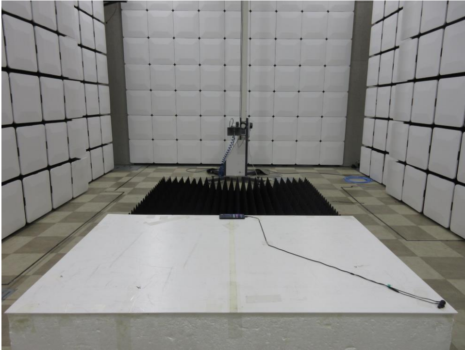
EUT & Earphone
