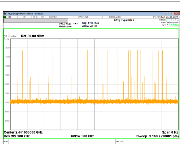
NUMBER OF PULSES IN 3.16 SECOND OBSERVATION PERIOD – DH3
