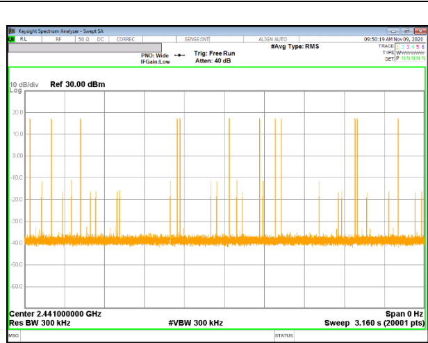
NUMBER OF PULSES IN 3.16 SECOND OBSERVATION PERIOD – DH5
