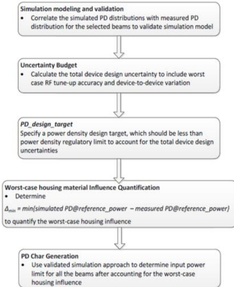
Figure 4-2: Flow chart for Power density characterization
