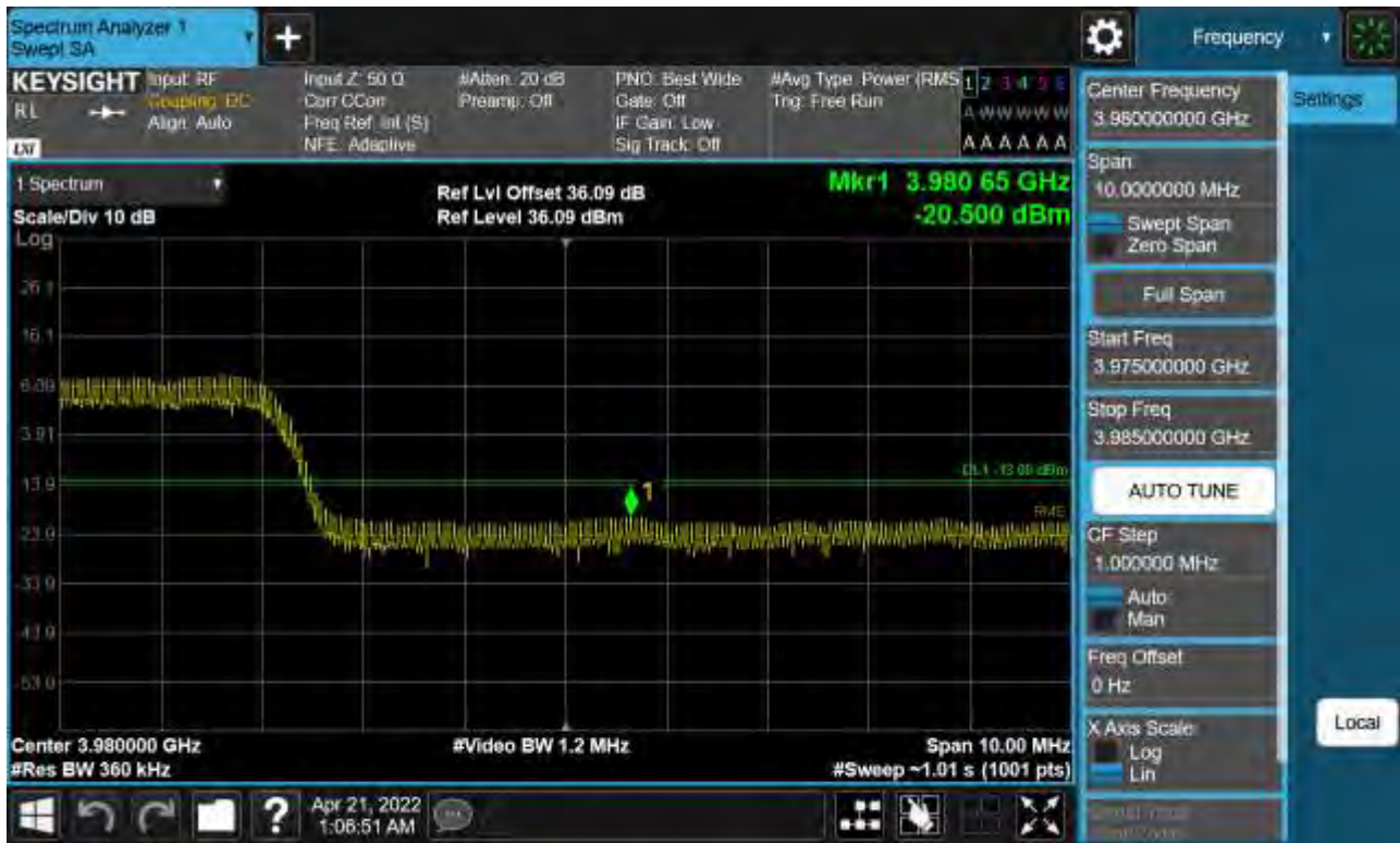
Sub6 n77. High Band Edge Plot (50 M BW Ch.663666 BPSK FullRB)(1)
