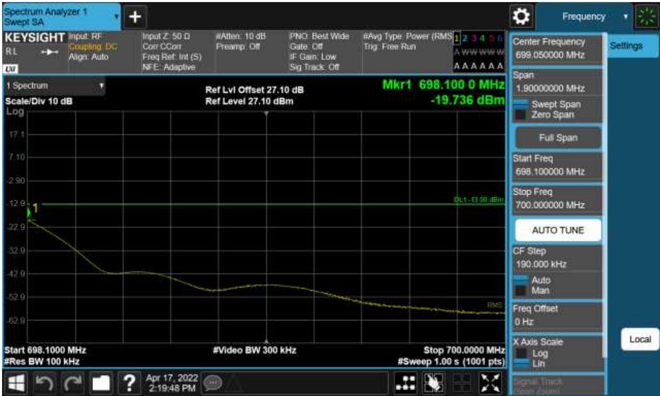
Sub6 n71. Upper Band Edge Plot (10 M BW Ch.138600 BPSK_RB1_Offset 51)-2
