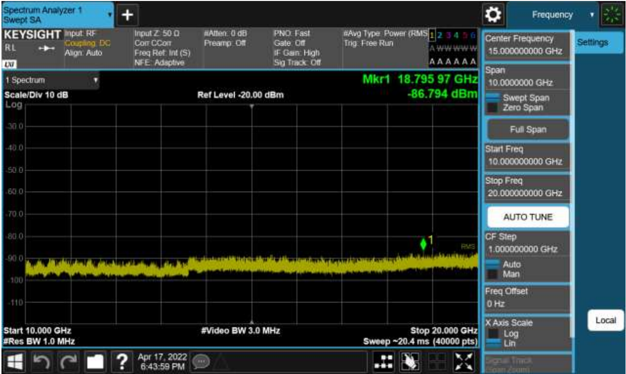
Sub6 n66. Conducted Spurious Plot_2 (349000ch_5 MHz_BPSK_RB 1_1)
