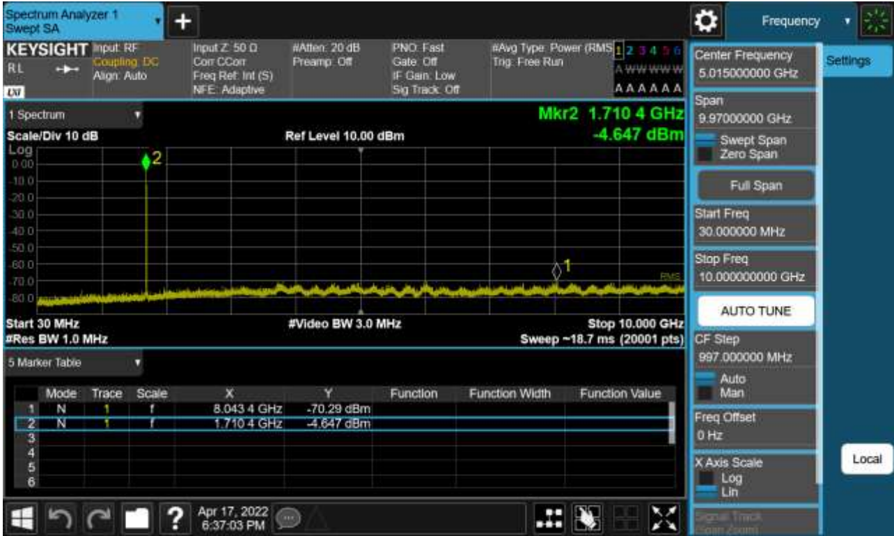
Sub6 n66. Conducted Spurious Plot_1 (342500ch_5 MHz_BPSK_RB 1_1)
