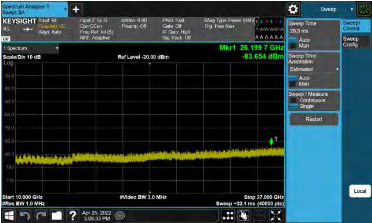
Sub6 n41. Conducted Spurious Plot 2 (100 MHz Ch.510000 BPSK RB 1)
