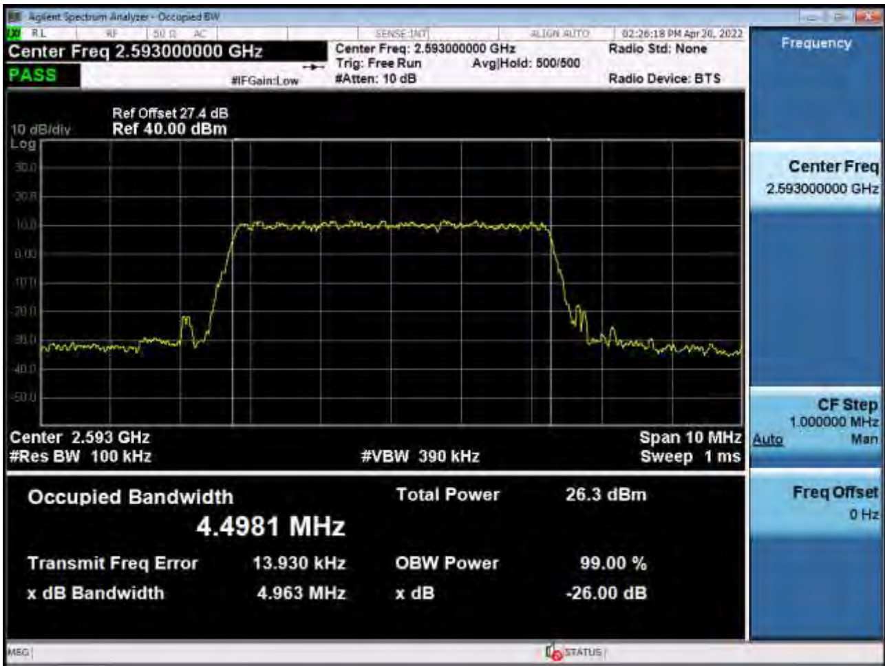
Occupied Bandwidth Plot (5 MHz Ch.40620 256-QAM RB 25) (POWER CLASS 3)
