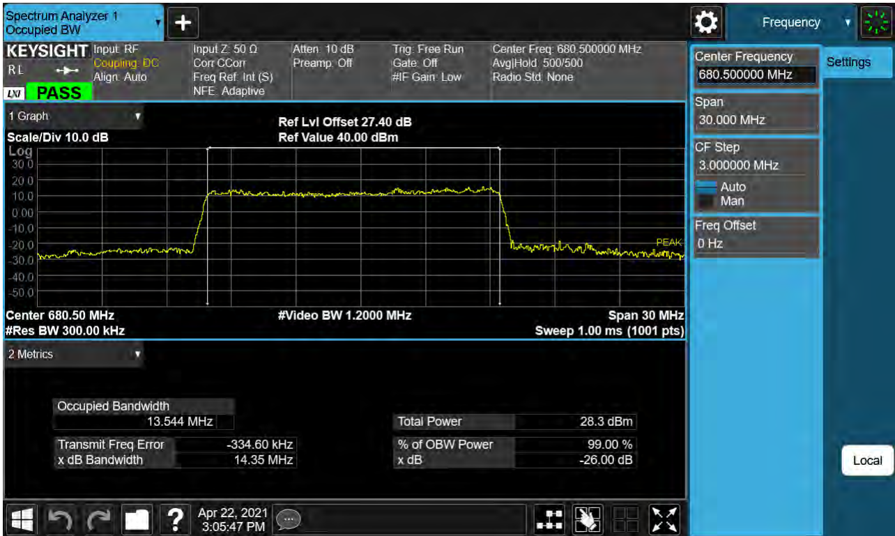
Sub6 n71. Occupied Bandwidth Plot (15M BW Ch.136100 256QAM_RB75_0)
