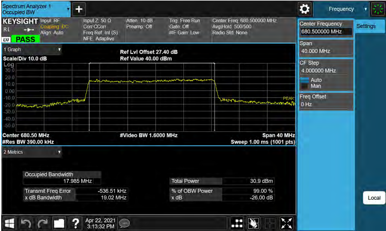
Sub6 n71. Occupied Bandwidth Plot (20M BW Ch.136100 64QAM_RB100_0)
