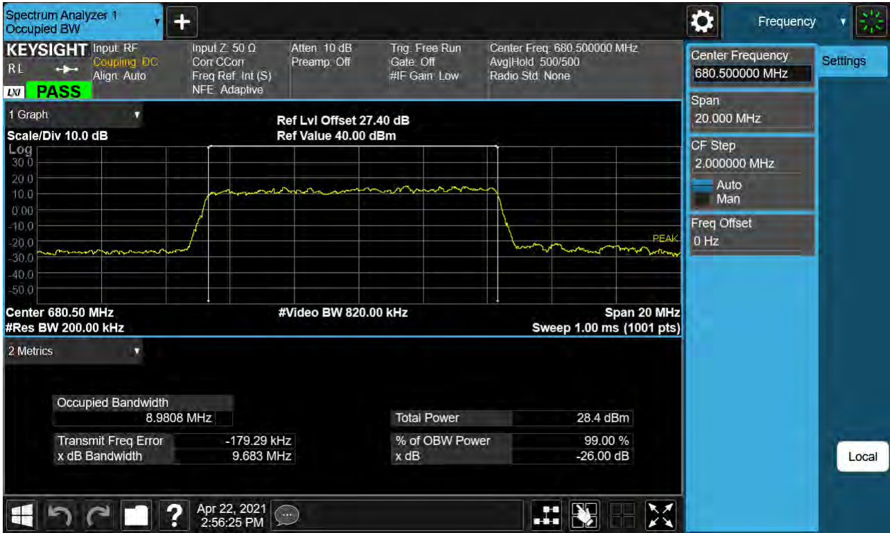
Sub6 n71. Occupied Bandwidth Plot (10M BW Ch.136100 256QAM_RB50_0)
