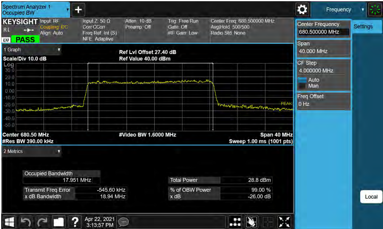
Sub6 n71. Occupied Bandwidth Plot (20M BW Ch.136100 256QAM_RB100_0)
