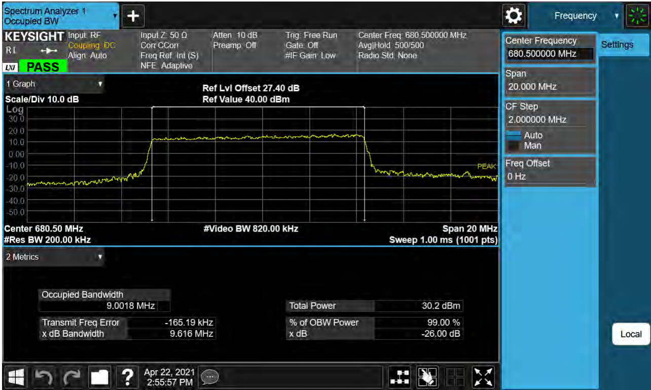
Sub6 n71. Occupied Bandwidth Plot (10M BW Ch.136100 64QAM_RB50_0)
