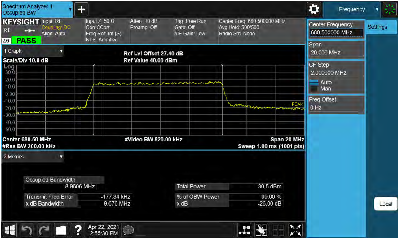
Sub6 n71. Occupied Bandwidth Plot (10M BW Ch.136100 16QAM_RB50_0)
