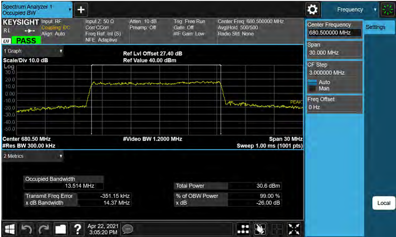
Sub6 n71. Occupied Bandwidth Plot (15M BW Ch.136100 64QAM_RB75_0)
