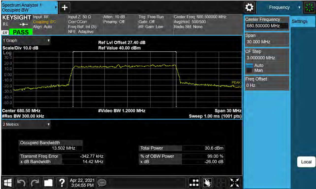
Sub6 n71. Occupied Bandwidth Plot (15M BW Ch.136100 16QAM_RB75_0)
