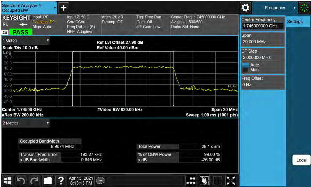
Sub6 n66. Occupied Bandwidth Plot (10M BW Ch.349000 256QAM RB 50)
