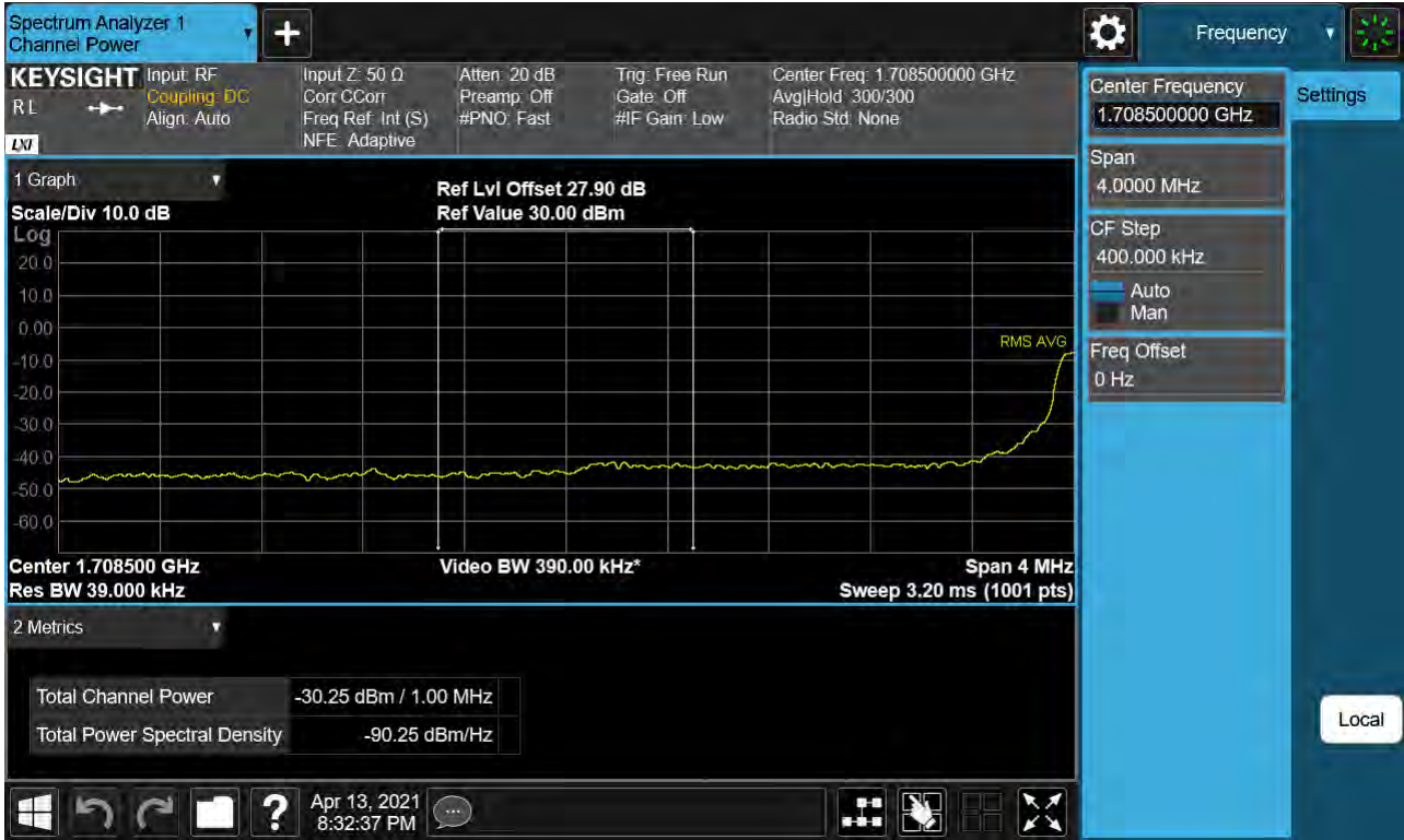
Sub6 n66. Lower Extended Band Edge Plot (20M BW Ch.344000 BPSK_RB100_0) -3
