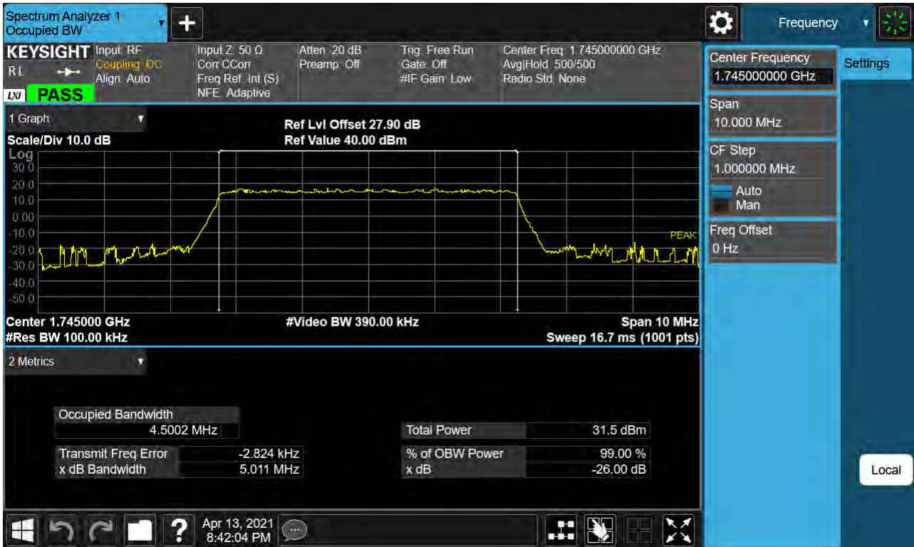
Sub6 n66. Occupied Bandwidth Plot (5M BW Ch.349000 QPSK RB 25)
