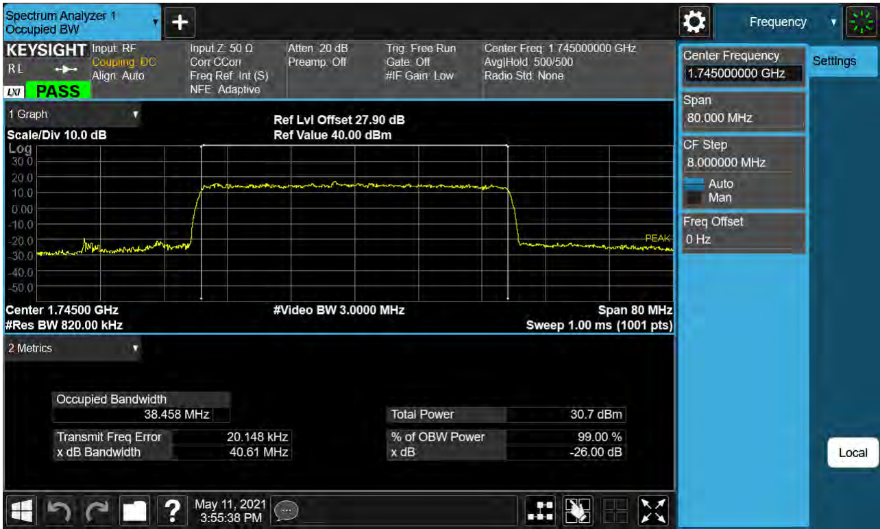
Sub6 n66. Occupied Bandwidth Plot (40M BW Ch.349000 64QAM RB 216)
