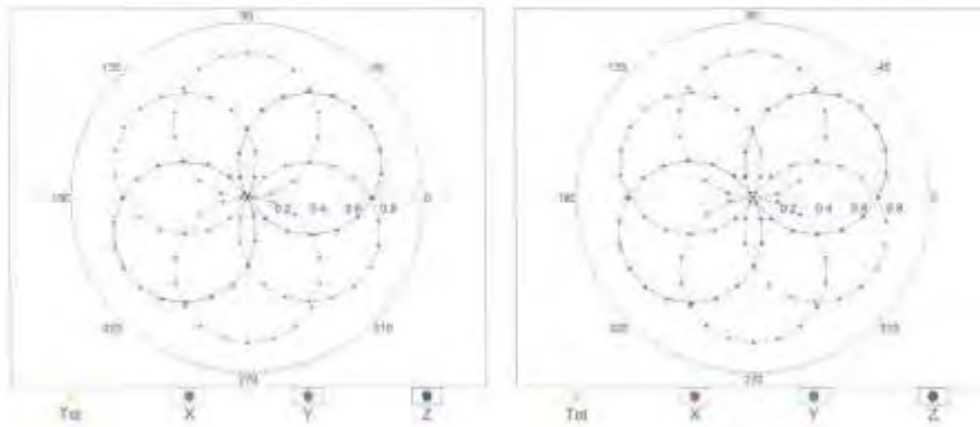
f=600 MHz,TEM
