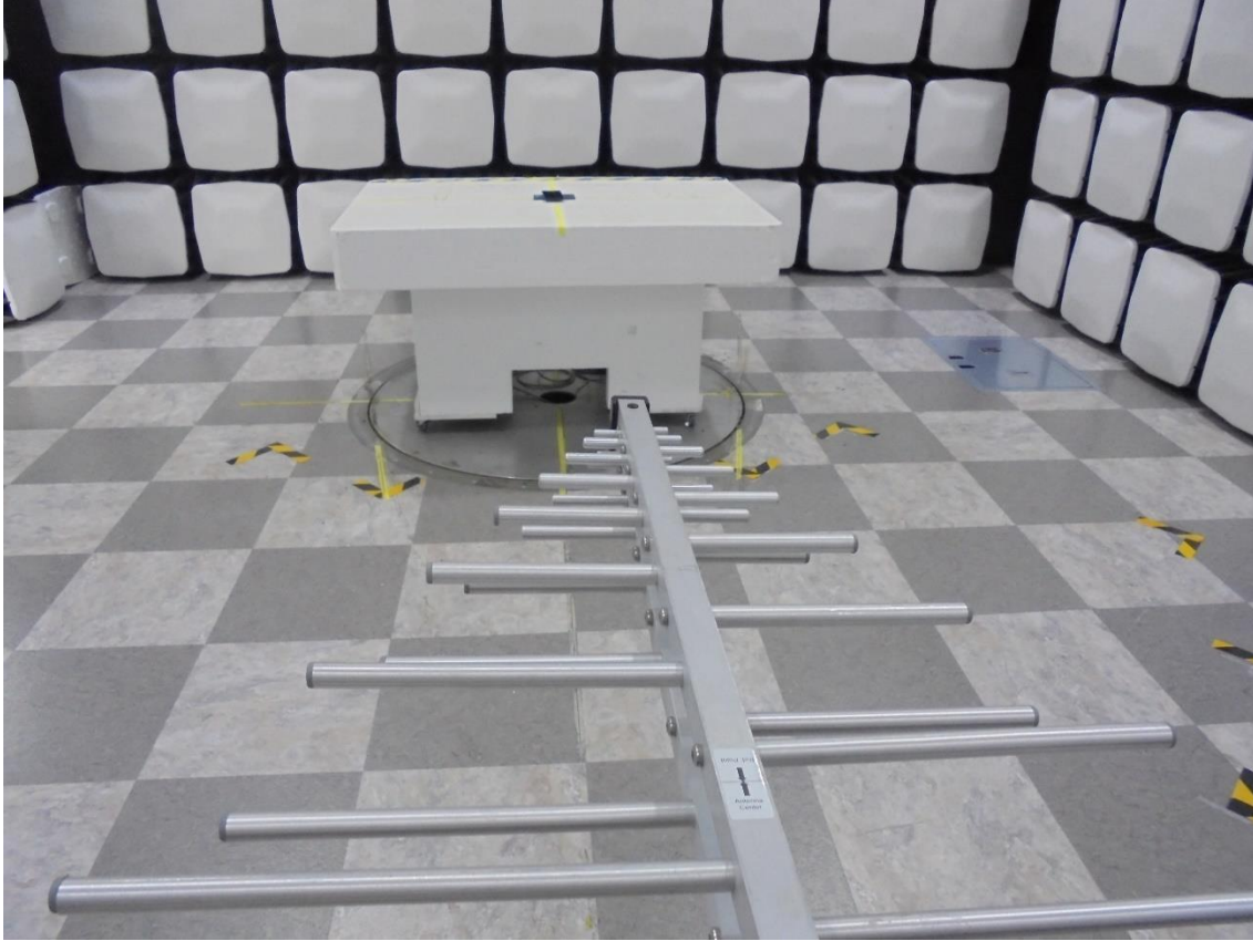
WPT Radiated Test Setup Photo for 30 MHz ~ 1 GHz :
