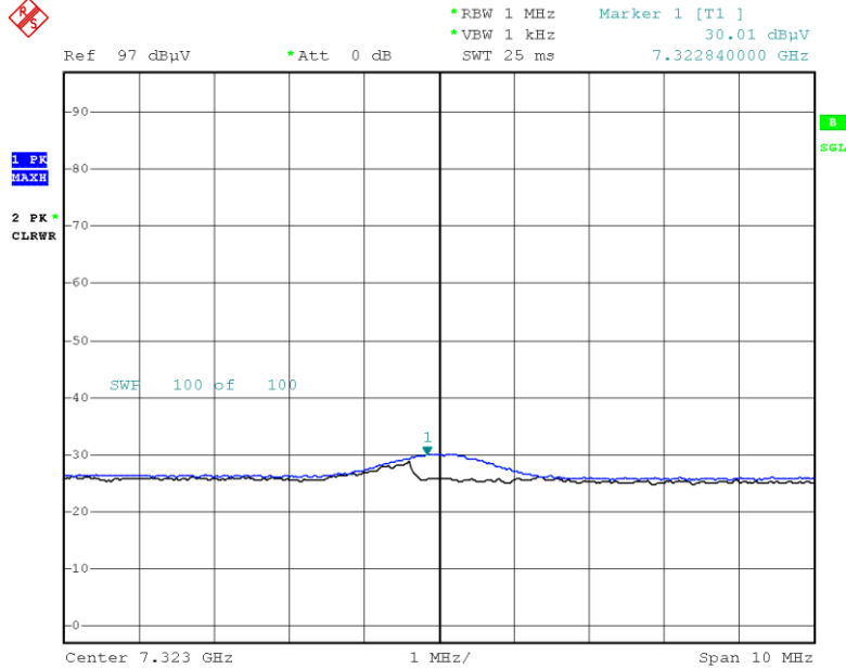
Radiated Spurious Emissions plot – Average Result (GFSK, Ch. 39 3rd Harmonic, H)
