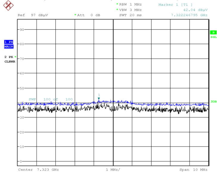
Radiated Spurious Emissions plot –Peak Result (3rd Harmonic, X-V)
