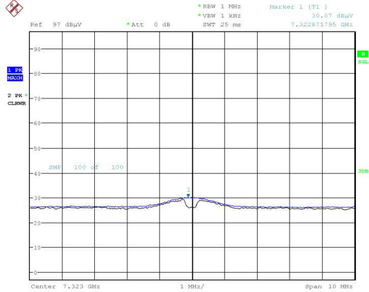
Radiated Spurious Emissions plot – Average Result (3rd Harmonic, X-V)
