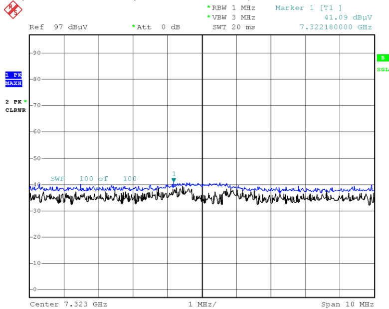
Radiated Spurious Emissions plot – Peak Result (GFSK, Ch. 39 3rd Harmonic, H)
