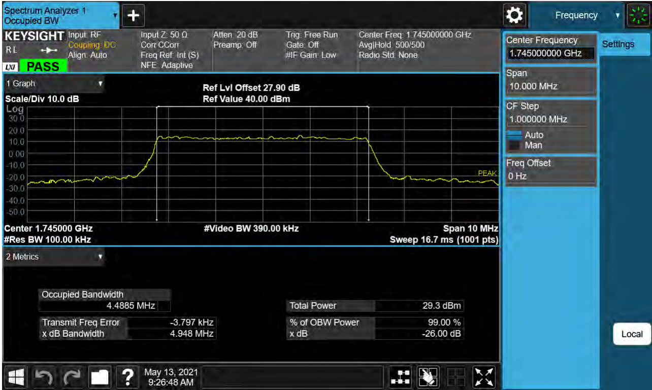
Sub6 n66. Occupied Bandwidth Plot (5M BW Ch.349000 64QAM RB 25)
