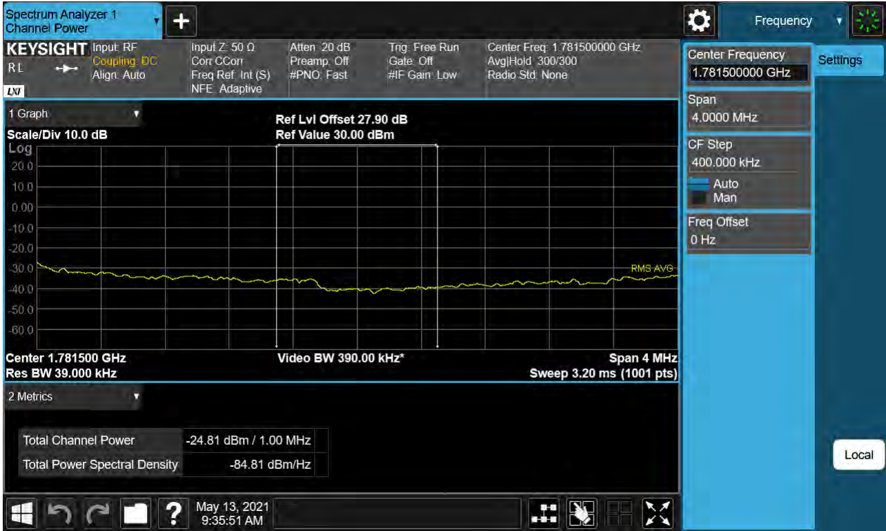
Sub6 n66. Upper Extended Band Edge Plot (10M BW Ch.355000 BPSK_RB50_0) -3
