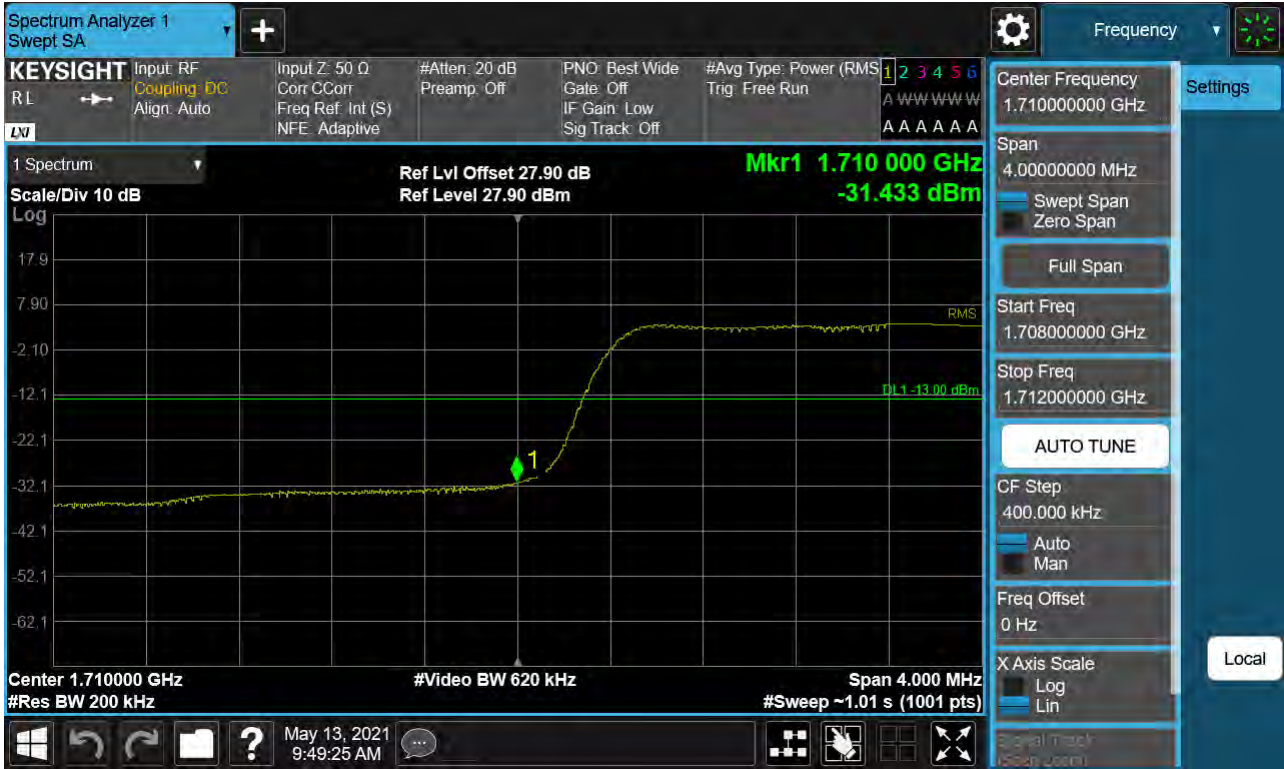
Sub6 n66. Lower Band Edge Plot (20M BW Ch.344000 BPSK RB 100_0) -2
