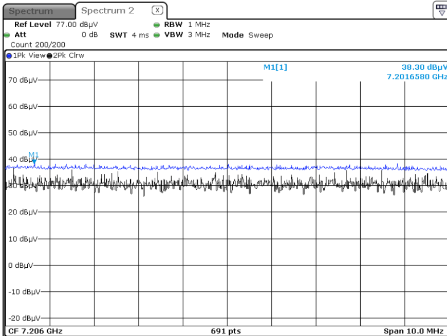
Radiated Spurious Emissions plot –Peak Reading (8DPSK, Ch.0 3rd Harmonic, X-H)
