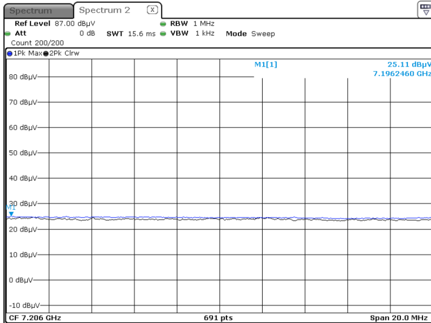
Radiated Spurious Emissions plot – Average Reading (Test case 3_3rd Harmonic, X-H)
