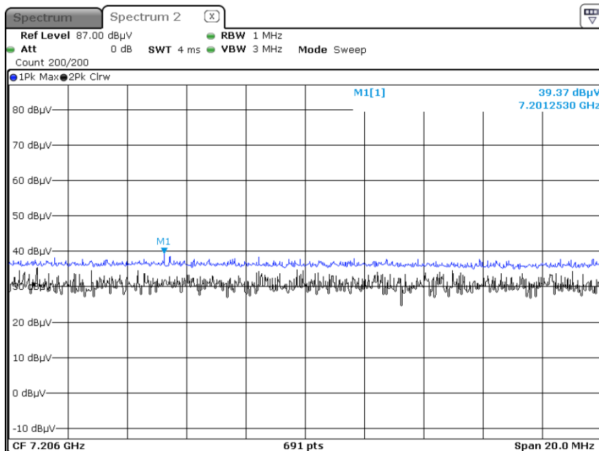
Radiated Spurious Emissions plot –Peak Reading (Test case 3_3rd Harmonic, X-H)
