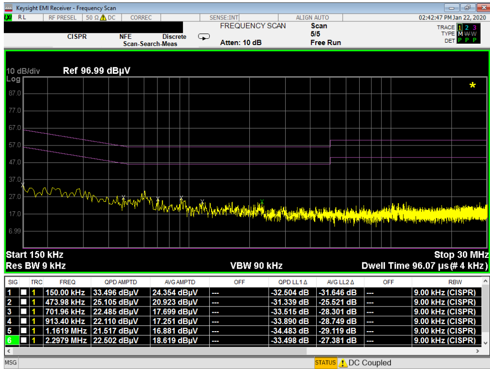
Plot 7-5. Line-Conducted Test Plot (L1) with Antenna Terminated in 50 Ω
