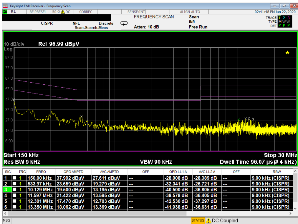
Plot 7-6. Line-Conducted Test Plot (N) with Antenna Terminated in 50 Ω
