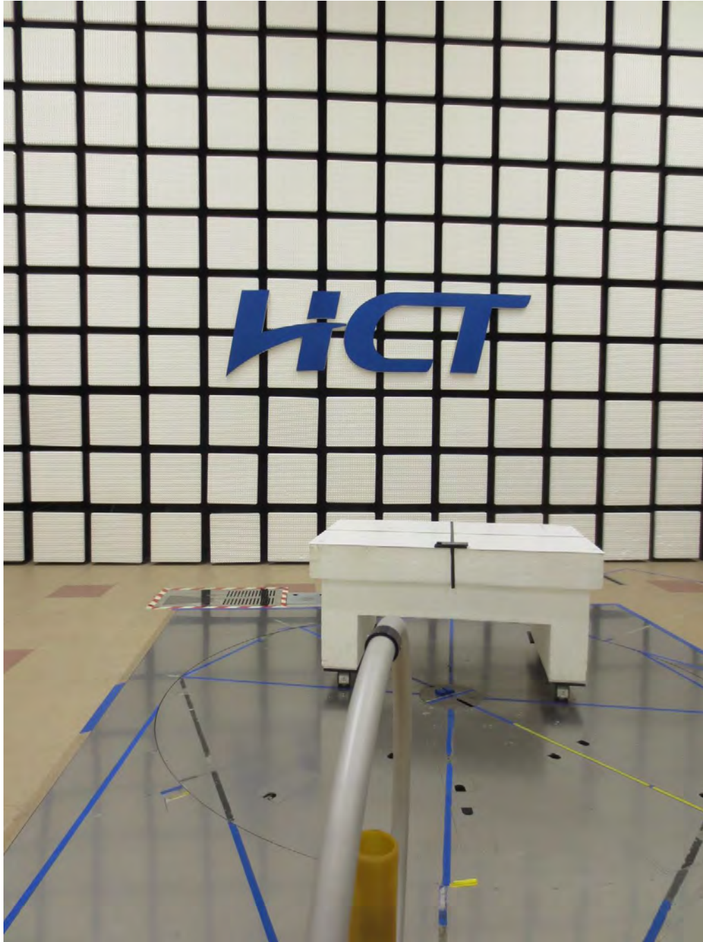
Radiated Test Setup Photo(WPT) for below 30 MHz:
