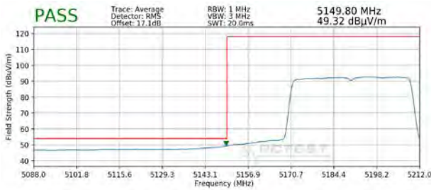
Plot 7-314. Radiated Lower Band Edge Plot SISO ANT2 (Average – UNII Band 1)
