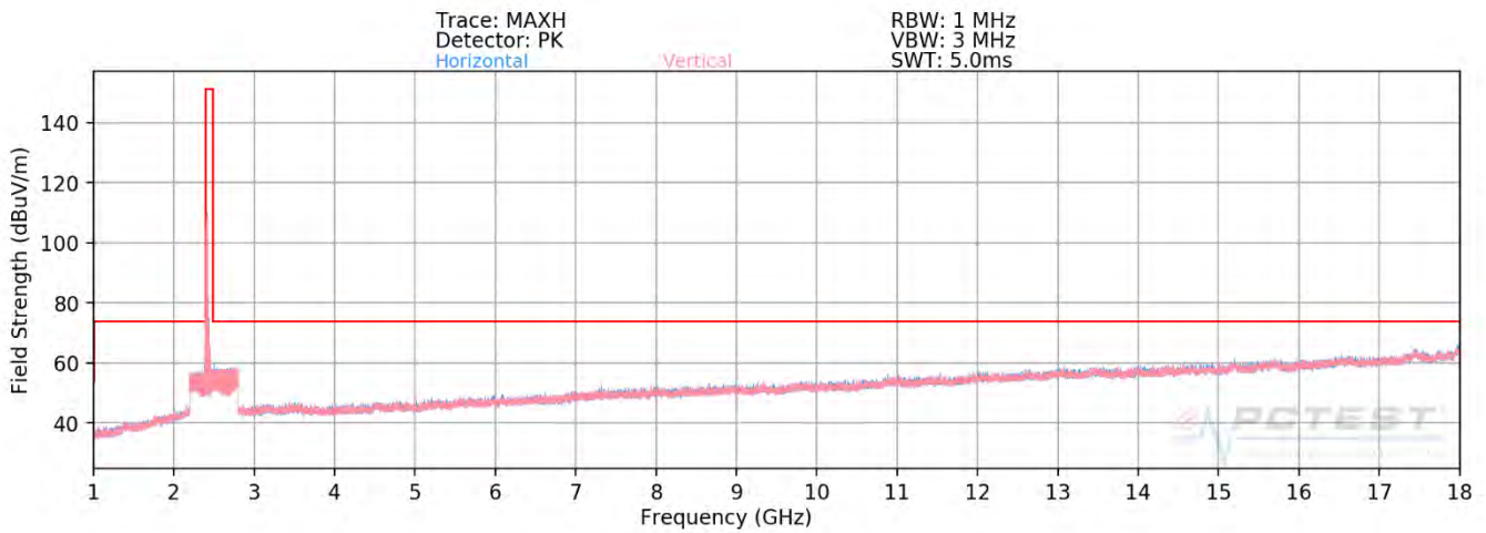
Plot 7-74. Radiated Spurious Plot above 1GHz SISO ANT1 (802.11ax OFDMA – 242 Tones – Ch. 1)
