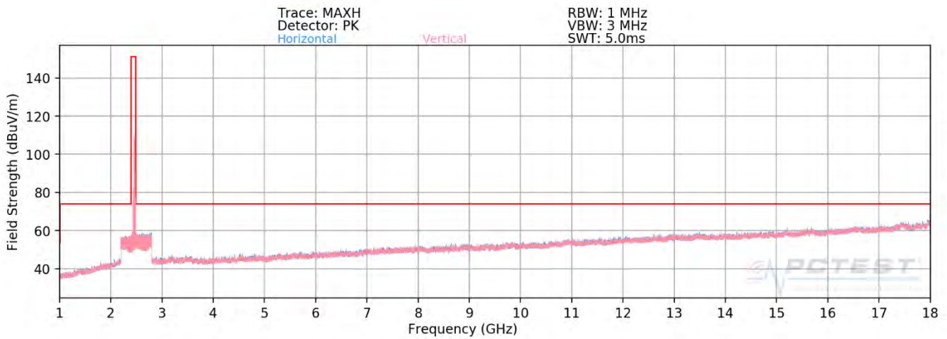
Plot 7-76. Radiated Spurious Plot above 1GHz SISO ANT1 (802.11ax OFDMA – 242 Tones – Ch. 11)
