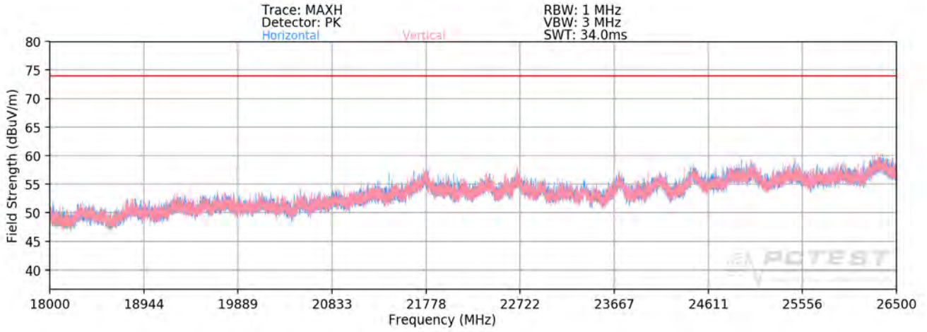
Plot 7-94. Radiated Spurious Plot above 18GHz SISO ANT1
