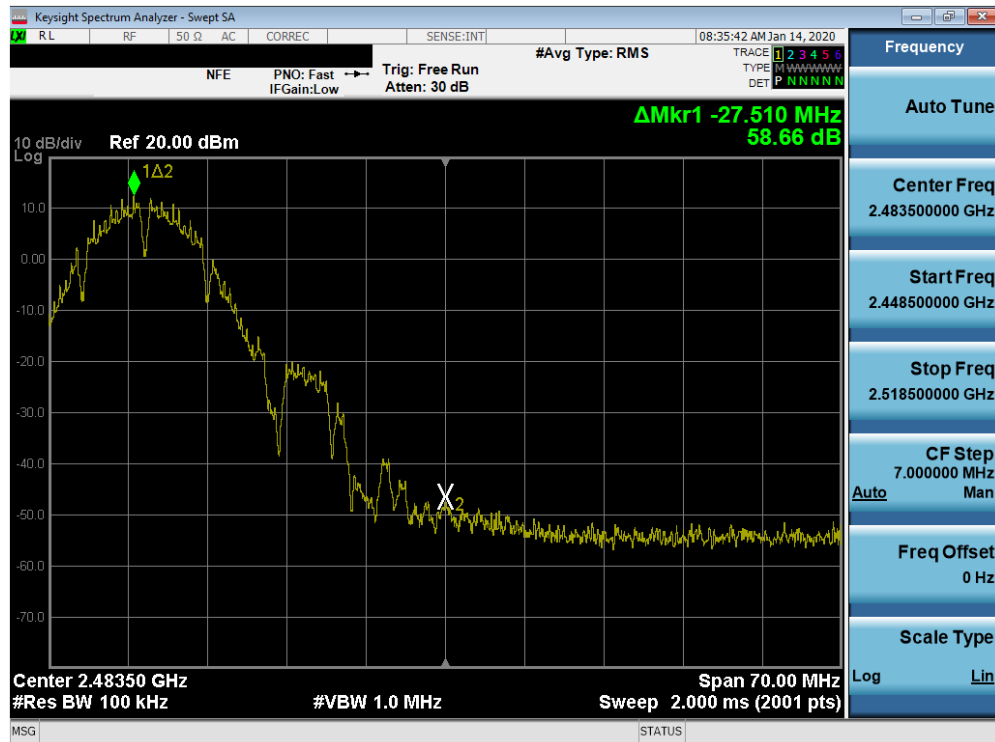
Plot 7-68. Band Edge Plot SISO ANT2 (802.11b – Ch. 10)
