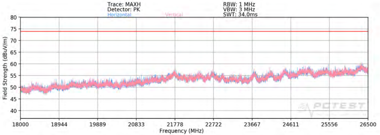
Plot 7-98. Radiated Spurious Plot above 18GHz SISO ANT2
