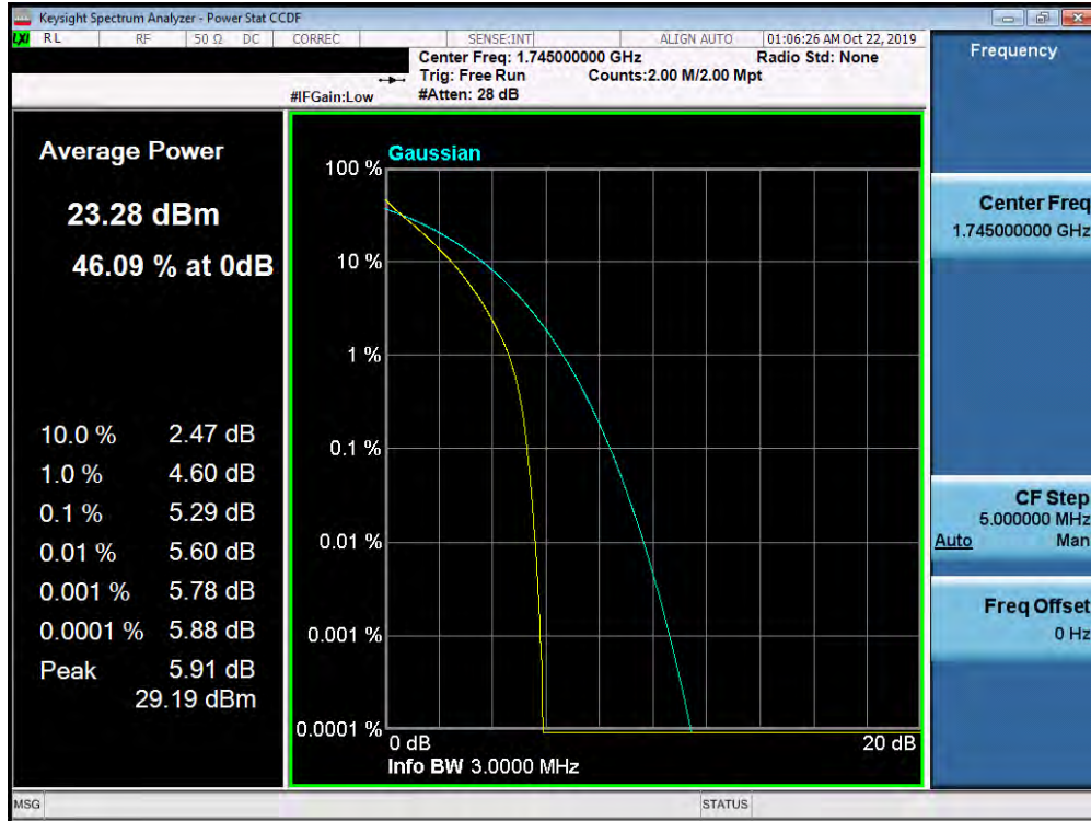
Plot 7-434. PAR Plot (Band 66/4 - 3.0MHz QPSK - Full RB Configuration)
