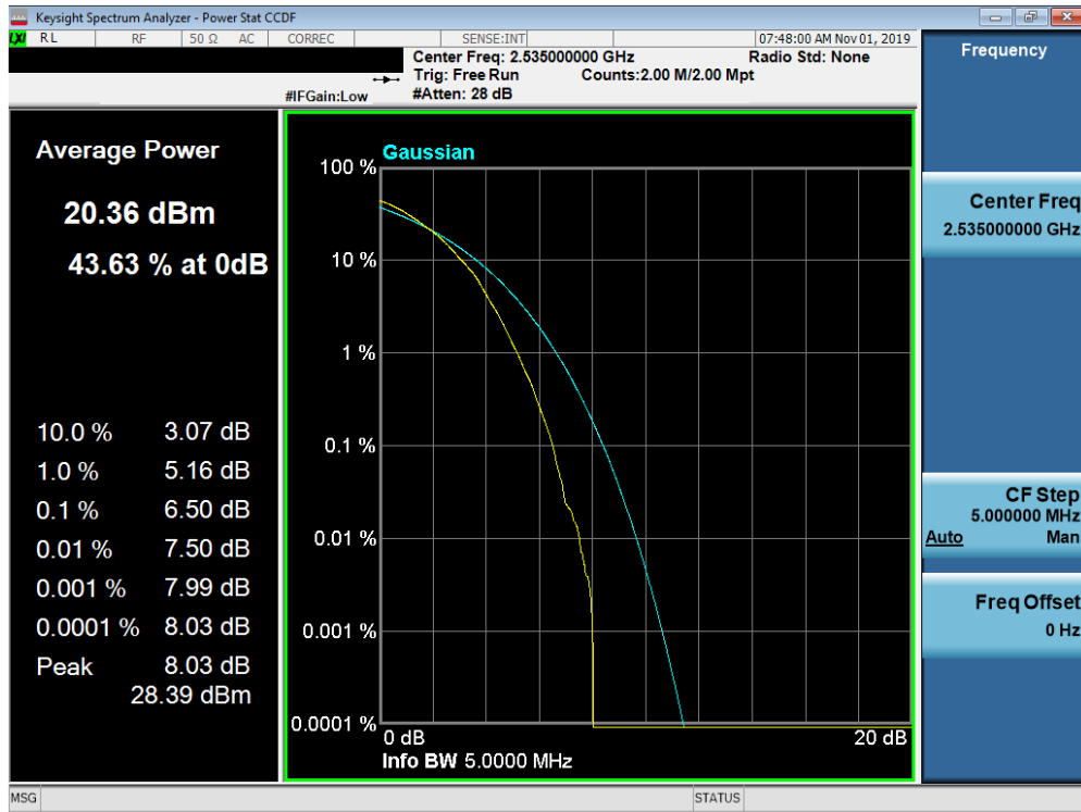
Plot 7-464. PAR Plot (Band 7 – 5.0MHz 64-QAM - Full RB Configuration)
