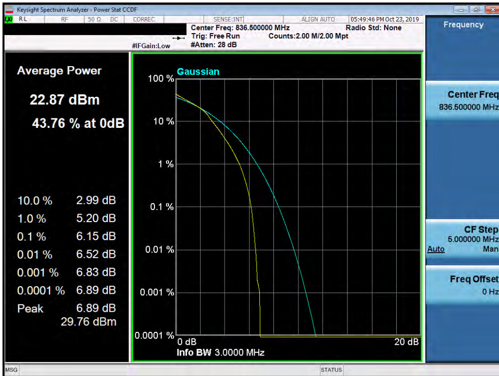
Plot 7-395. PAR Plot (Band 5 – 3.0MHz 16-QAM - Full RB Configuration)
