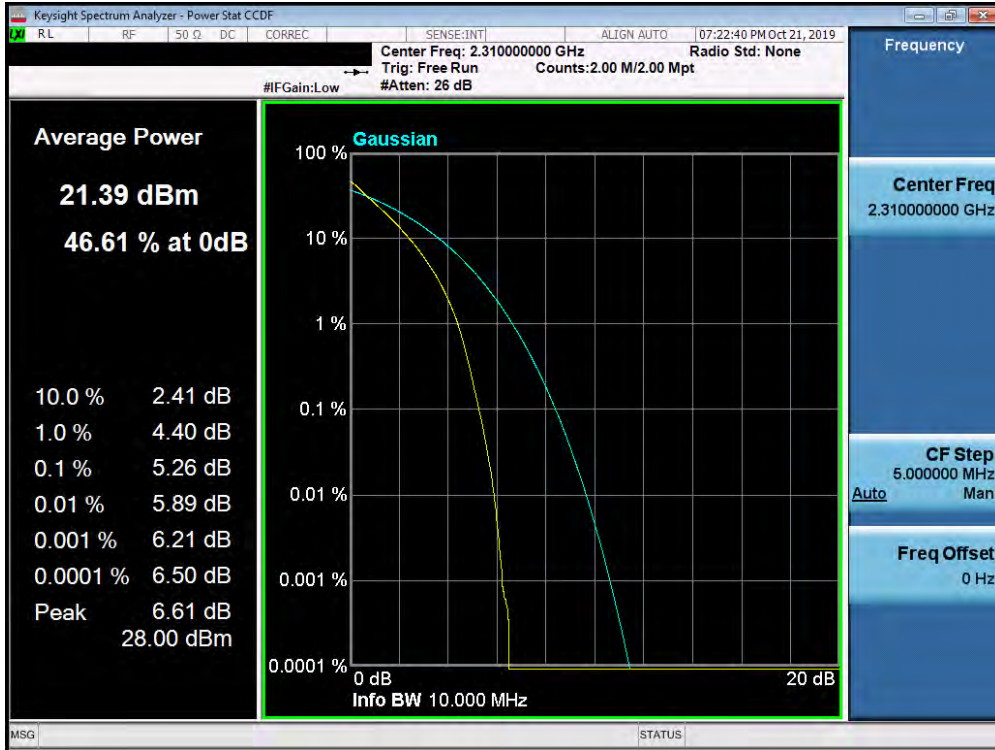
Plot 7-458. PAR Plot (Band 30 – 10.0MHz QPSK - Full RB Configuration)
