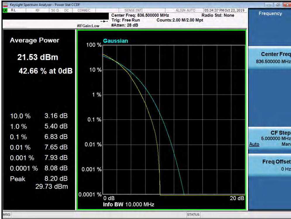
Plot 7-404. PAR Plot (Band 5 – 10.0MHz 64-QAM - Full RB Configuration)
