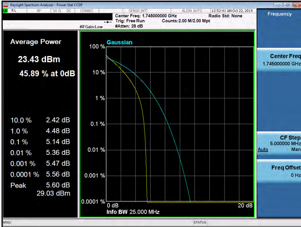
Plot 7-446. PAR Plot (Band 66/4 - 15.0MHz QPSK - Full RB Configuration)
