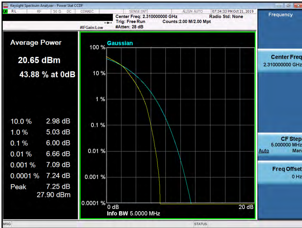
Plot 7-455. PAR Plot (Band 30 – 5.0MHz 16-QAM - Full RB Configuration)
