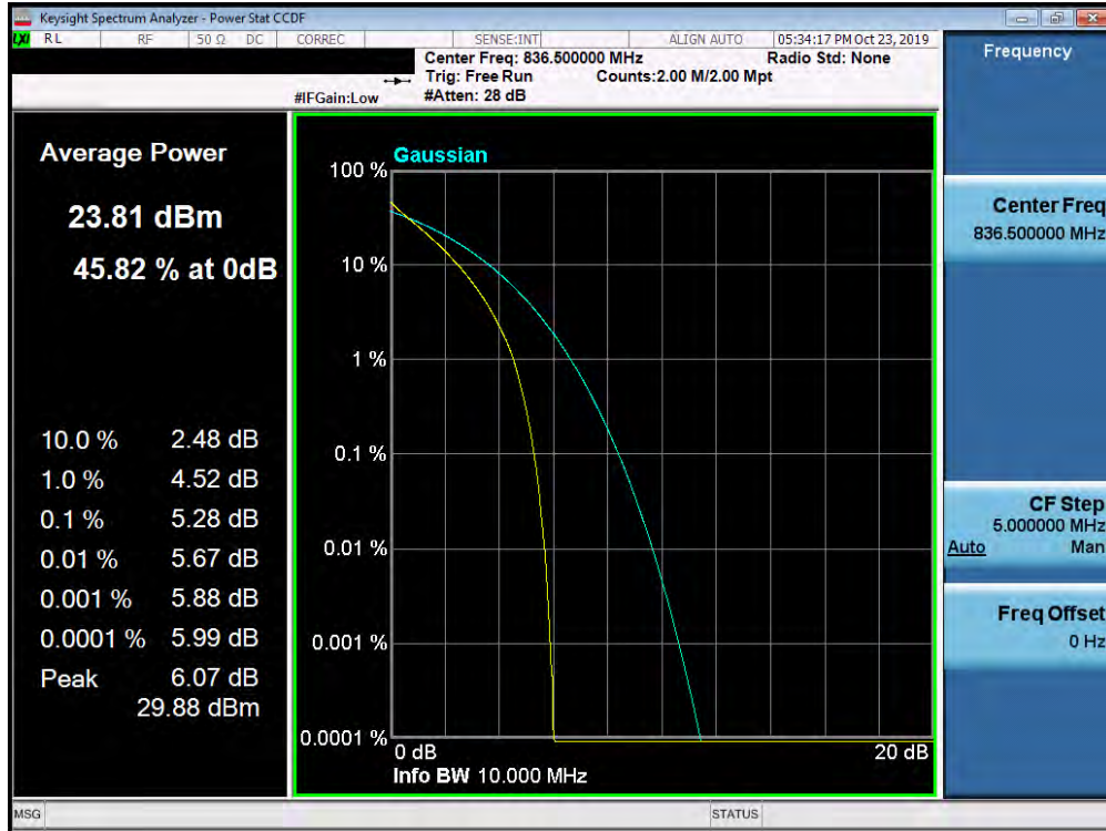
Plot 7-402. PAR Plot (Band 5 – 10.0MHz QPSK - Full RB Configuration)
