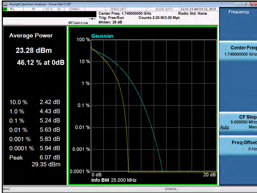
Plot 7-450. PAR Plot (Band 66/4 - 20.0MHz QPSK - Full RB Configuration)
