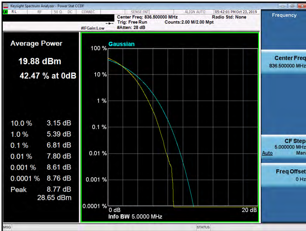
Plot 7-401. PAR Plot (Band 5 – 5.0MHz 256-QAM - Full RB Configuration)
