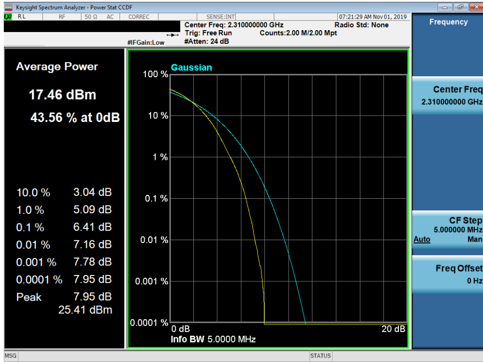
Plot 7-457. PAR Plot (Band 30 – 5.0MHz 256-QAM - Full RB Configuration)
