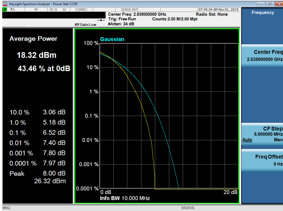
Plot 7-469. PAR Plot (Band 7 – 10.0MHz 256-QAM - Full RB Configuration)
