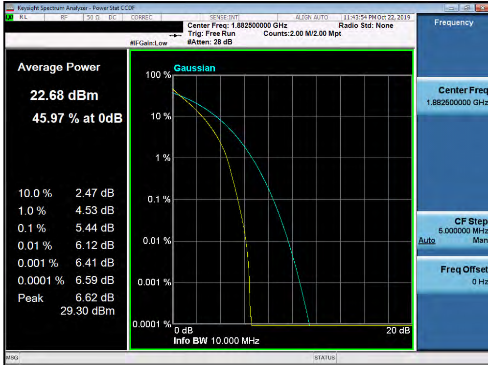
Plot 7-418. PAR Plot (Band 25/2 - 10.0MHz QPSK - Full RB Configuration)
