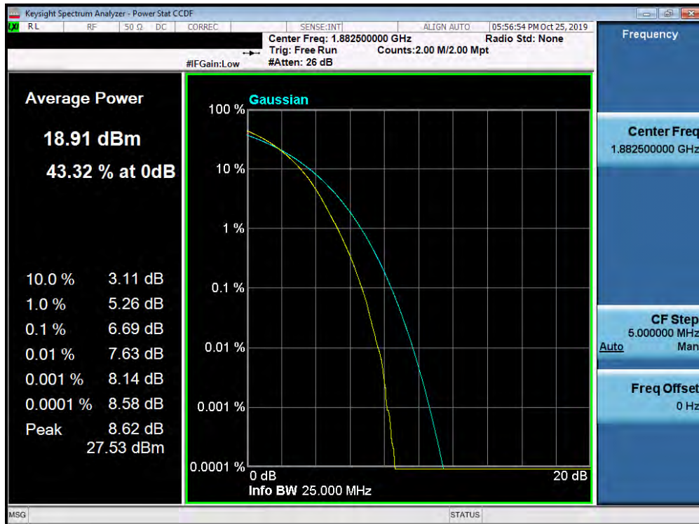
Plot 7-425. PAR Plot (Band 25/2 - 15.0MHz 256-QAM - Full RB Configuration)
