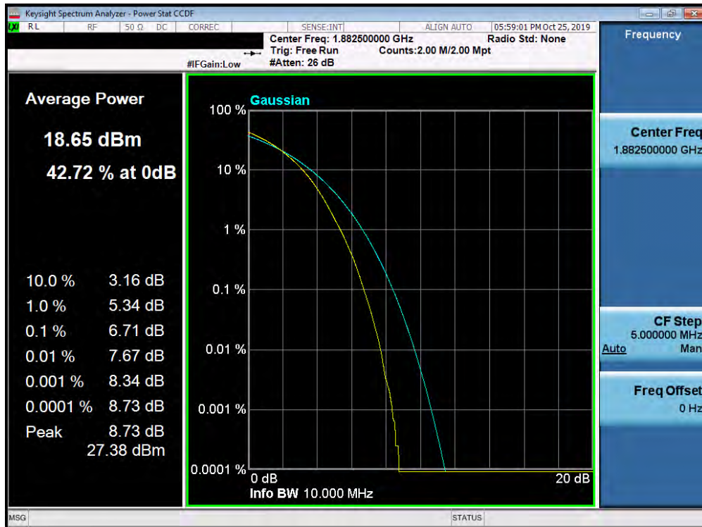
Plot 7-421. PAR Plot (Band 25/2 - 10.0MHz 256-QAM - Full RB Configuration)
