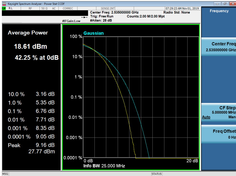
Plot 7-477. PAR Plot (Band 7 – 20.0MHz 256-QAM - Full RB Configuration)
