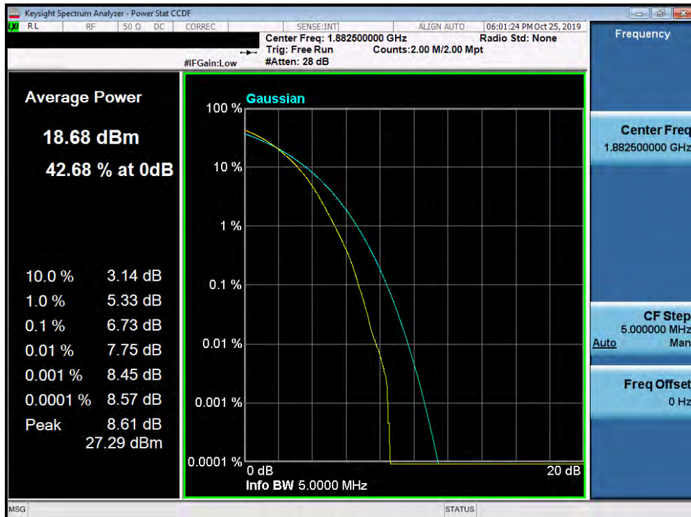
Plot 7-417. PAR Plot (Band 25/2 - 5.0MHz 256-QAM - Full RB Configuration)
