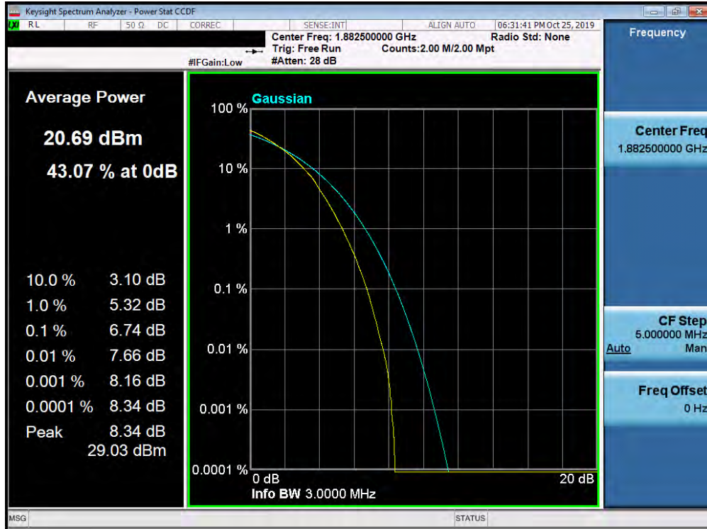
Plot 7-412. PAR Plot (Band 25/2 - 3.0MHz 64-QAM - Full RB Configuration)
