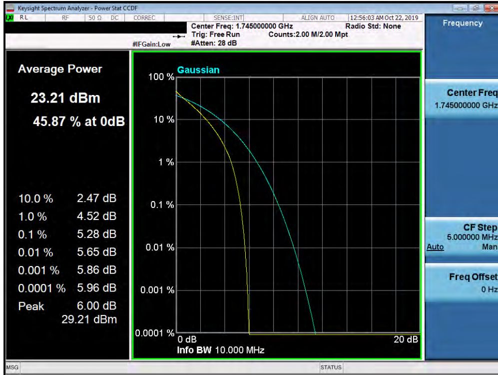
Plot 7-442. PAR Plot (Band 66/4 - 10.0MHz QPSK - Full RB Configuration)
