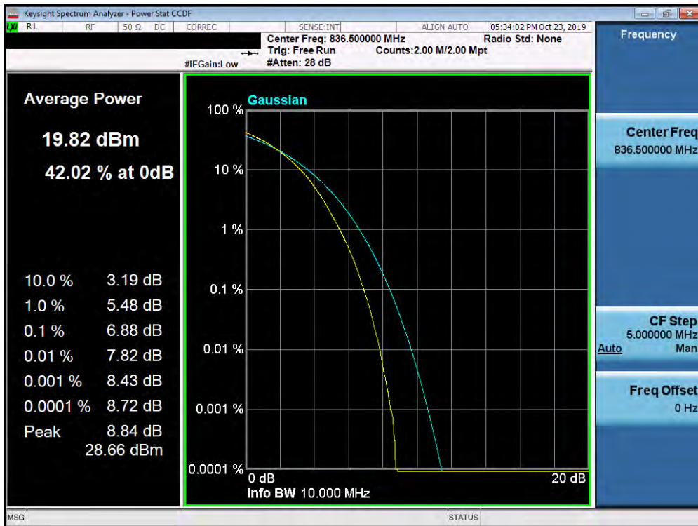
Plot 7-405. PAR Plot (Band 5 – 10.0MHz 256-QAM - Full RB Configuration)
