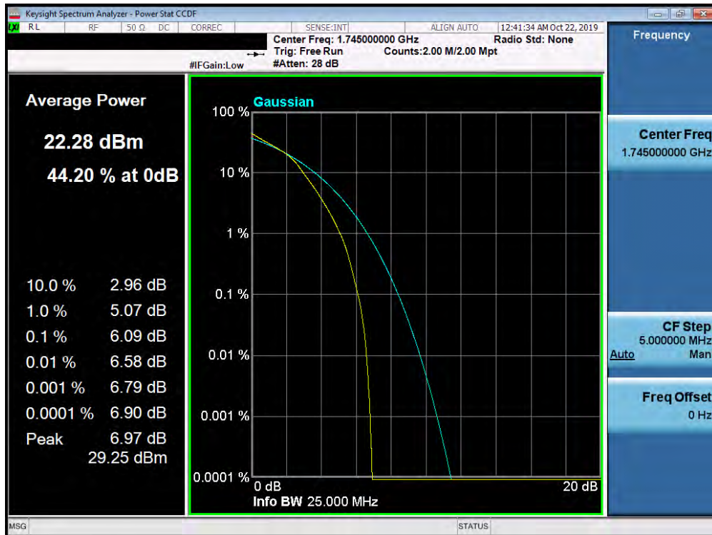
Plot 7-451. PAR Plot (Band 66/4 - 20.0MHz 16-QAM - Full RB Configuration)
