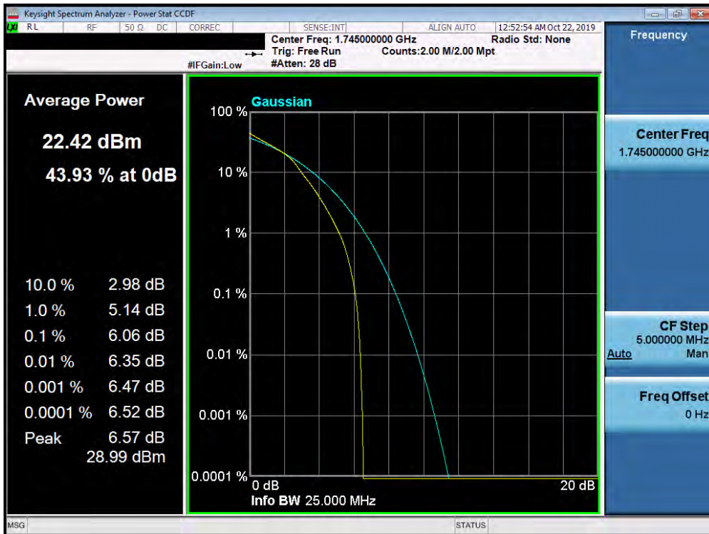
Plot 7-447. PAR Plot (Band 66/4 - 15.0MHz 16-QAM - Full RB Configuration)
