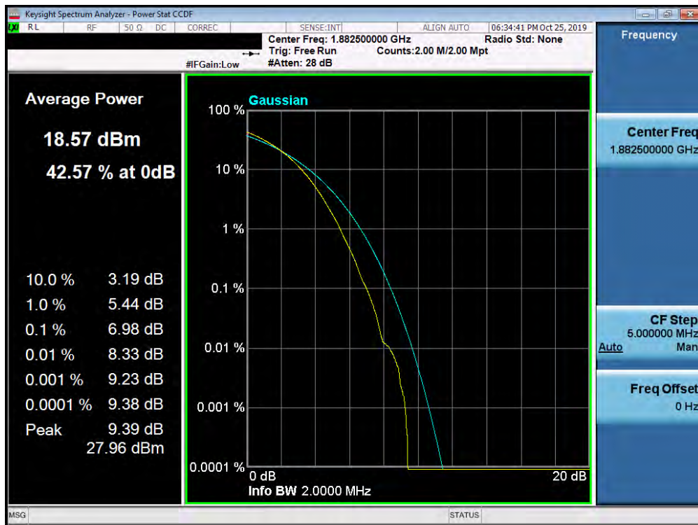
Plot 7-409. PAR Plot (Band 25/2 - 1.4MHz 256-QAM - Full RB Configuration)
