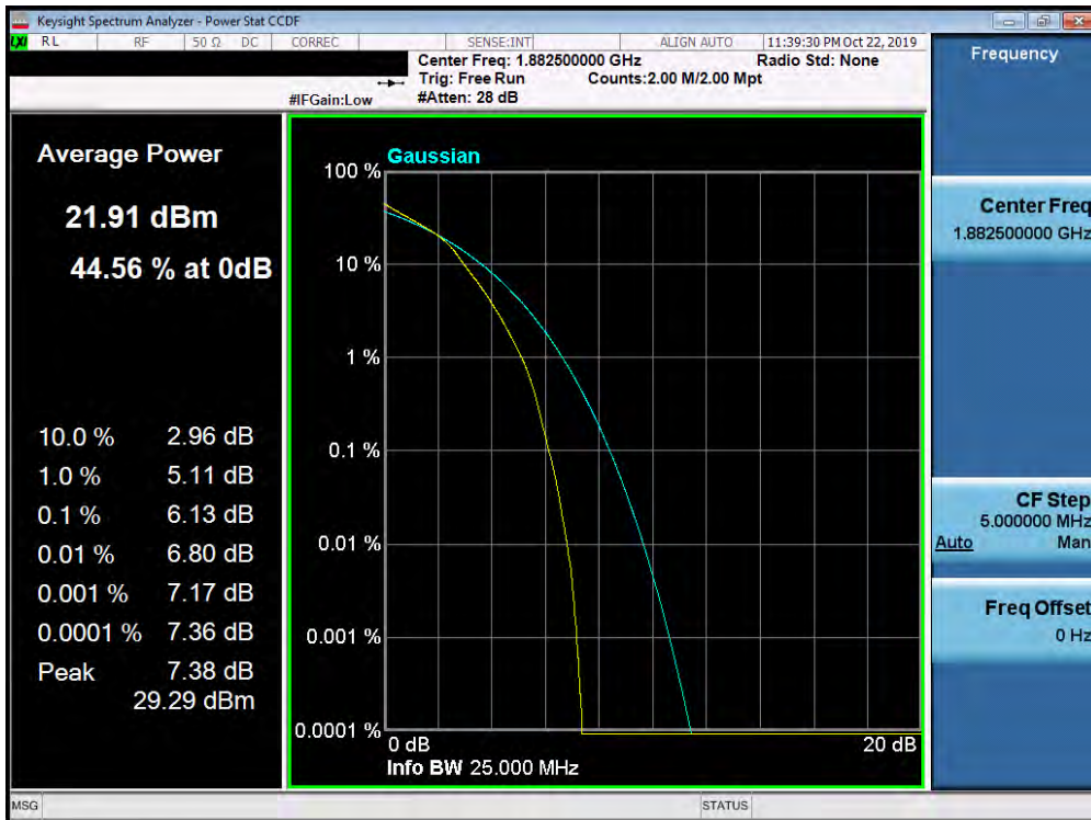
Plot 7-423. PAR Plot (Band 25/2 - 15.0MHz 16-QAM - Full RB Configuration)
