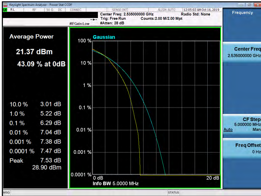
Plot 7-463. PAR Plot (Band 7 – 5.0MHz 16-QAM - Full RB Configuration)
