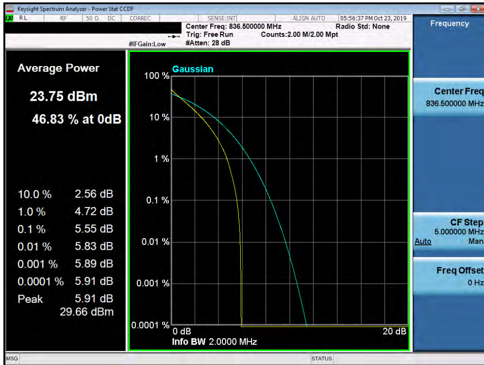
Plot 7-391. PAR Plot (Band 5 – 1.4MHz 16-QAM - Full RB Configuration)
