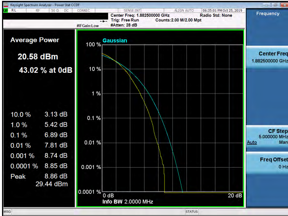
Plot 7-408. PAR Plot (Band 25/2 - 1.4MHz 64-QAM - Full RB Configuration)
