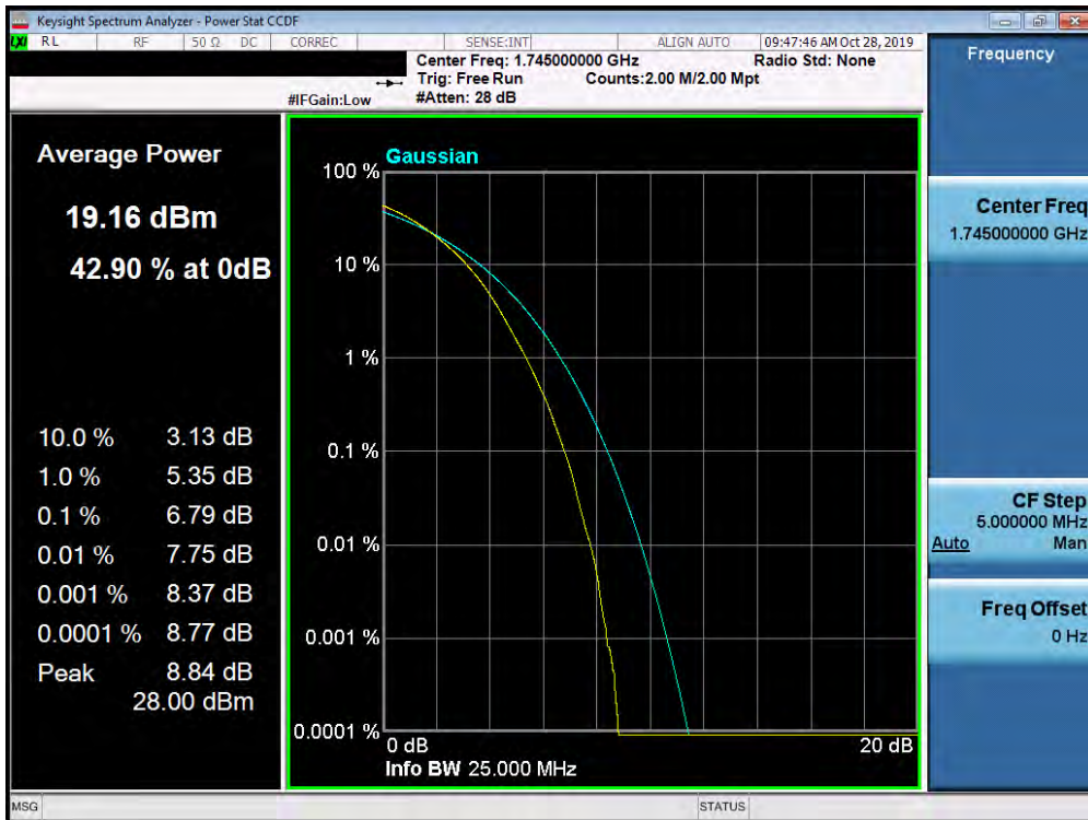
Plot 7-449. PAR Plot (Band 66/4 - 15.0MHz 256-QAM - Full RB Configuration)
