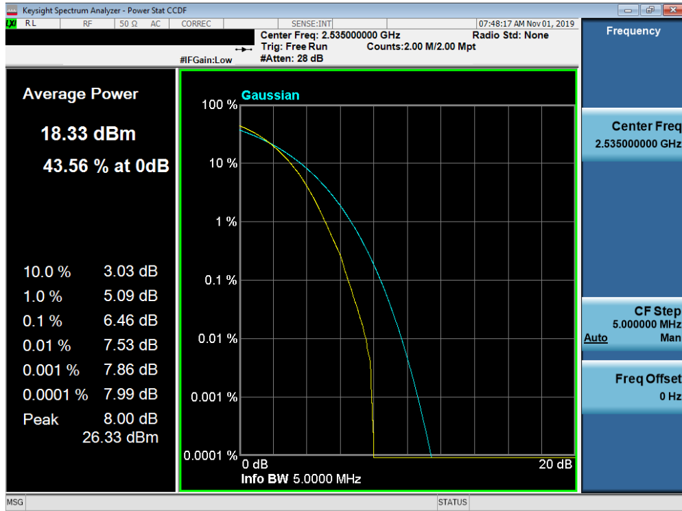
Plot 7-465. PAR Plot (Band 7 – 5.0MHz 256-QAM - Full RB Configuration)
