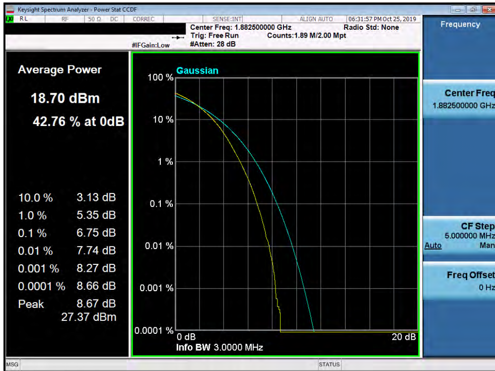
Plot 7-413. PAR Plot (Band 25/2 - 3.0MHz 256-QAM - Full RB Configuration)
