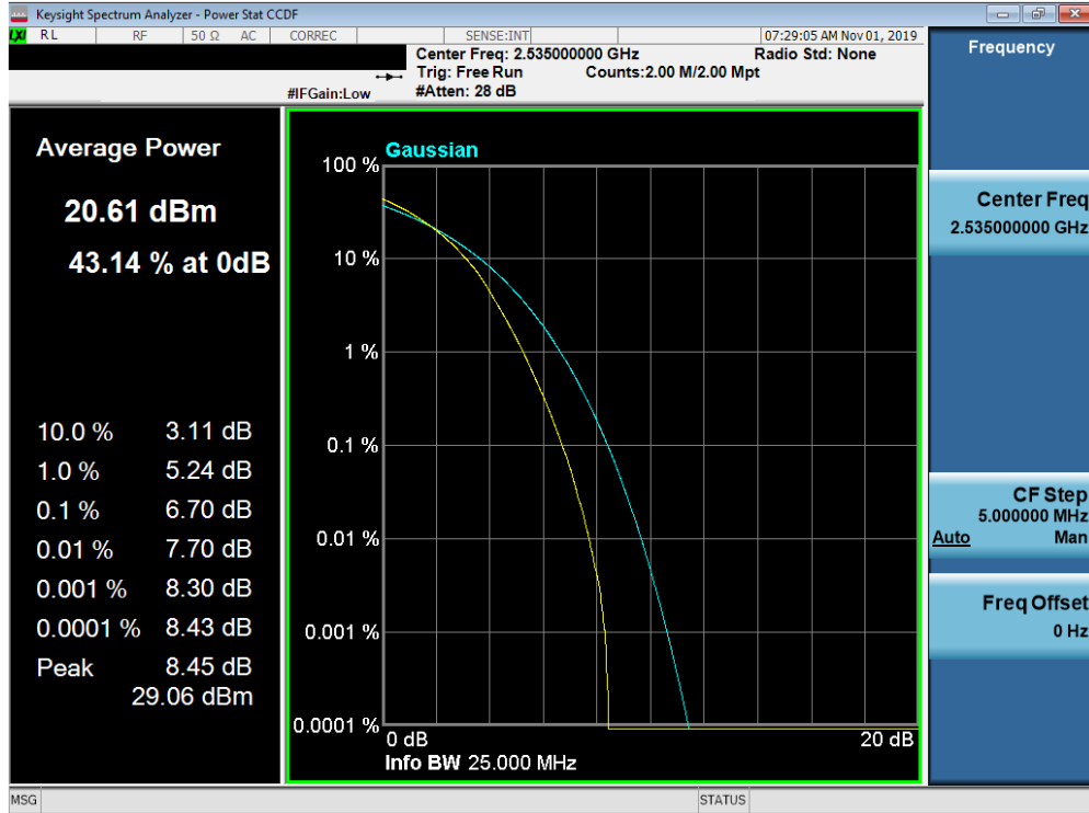
Plot 7-476. PAR Plot (Band 7 – 20.0MHz 64-QAM - Full RB Configuration)
