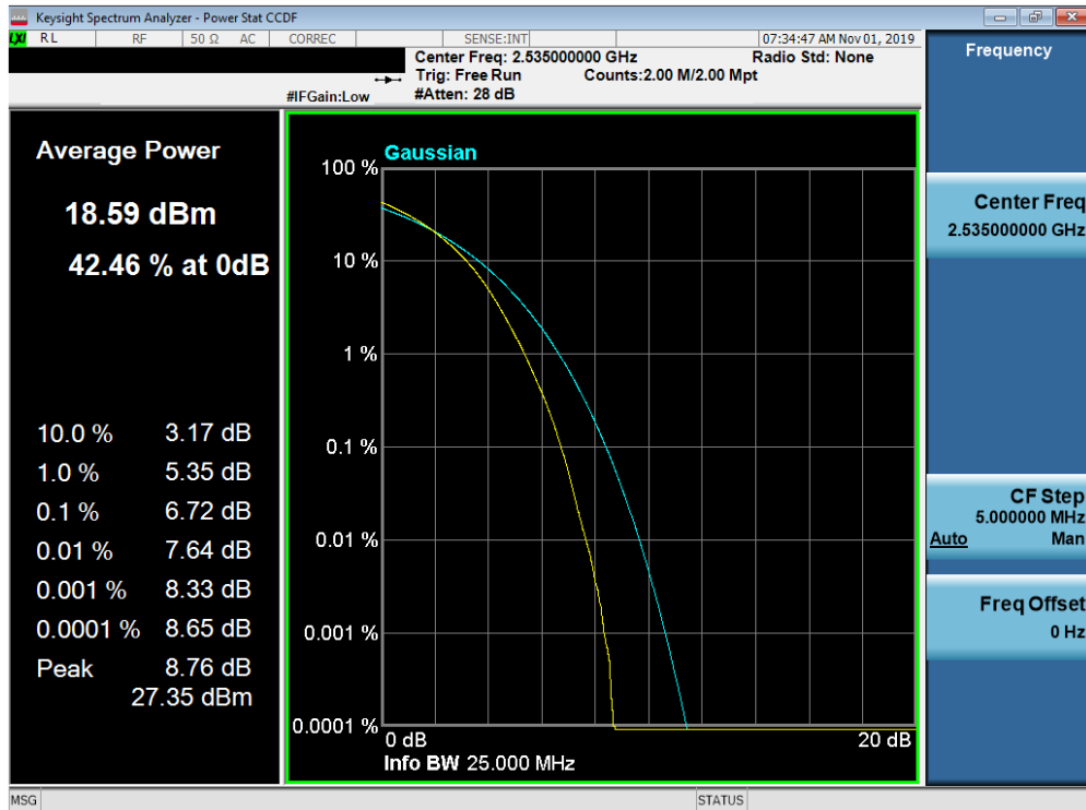
Plot 7-473. PAR Plot (Band 7 – 15.0MHz 256-QAM - Full RB Configuration)
