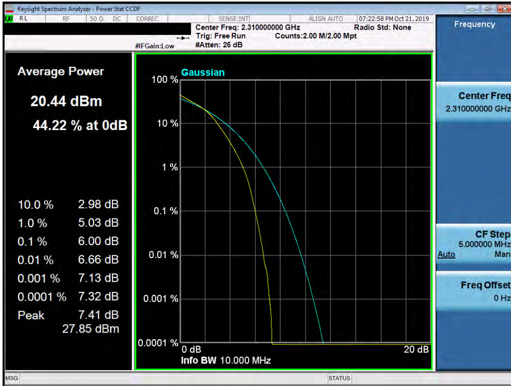
Plot 7-459. PAR Plot (Band 30 – 10.0MHz 16-QAM - Full RB Configuration)
