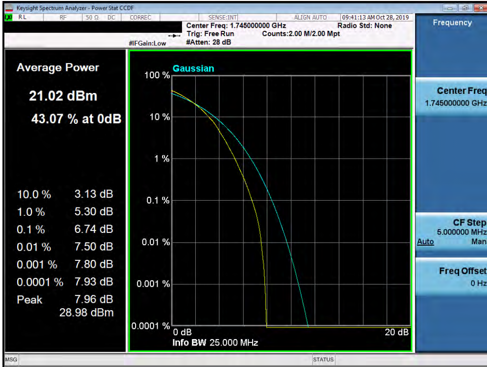
Plot 7-452. PAR Plot (Band 66/4 - 20.0MHz 64-QAM - Full RB Configuration)
