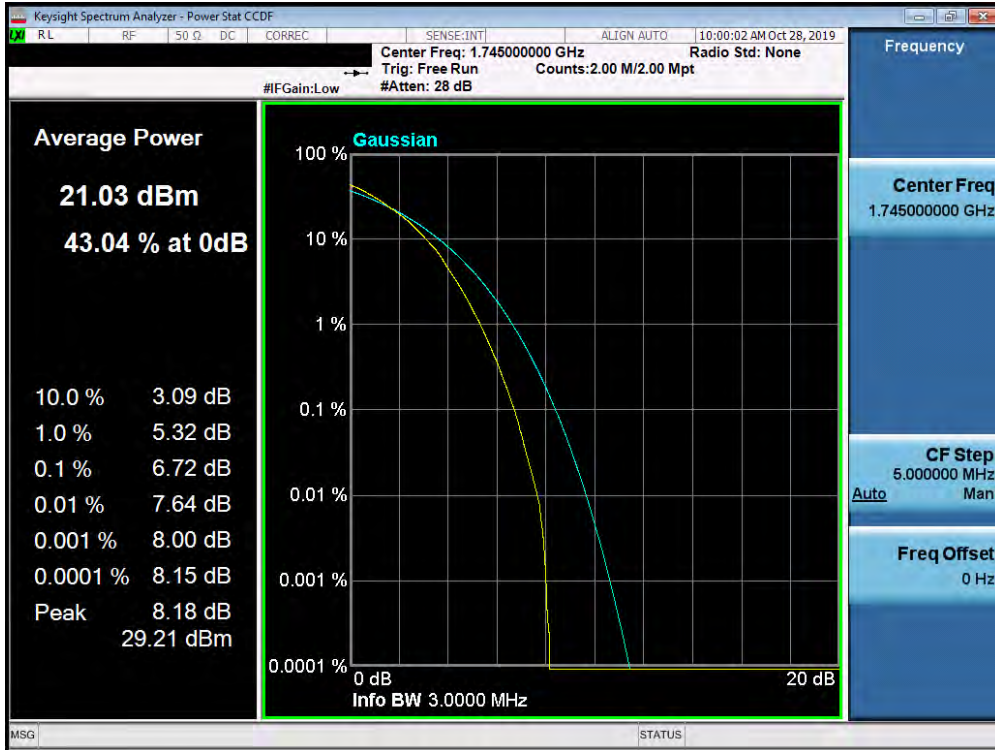
Plot 7-436. PAR Plot (Band 66/4 - 3.0MHz 64-QAM - Full RB Configuration)
