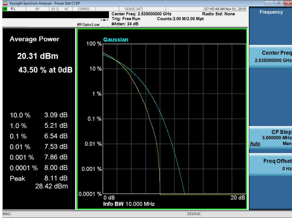
Plot 7-468. PAR Plot (Band 7 – 10.0MHz 64-QAM - Full RB Configuration)
