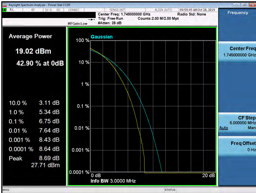
Plot 7-437. PAR Plot (Band 66/4 - 3.0MHz 256-QAM - Full RB Configuration)
