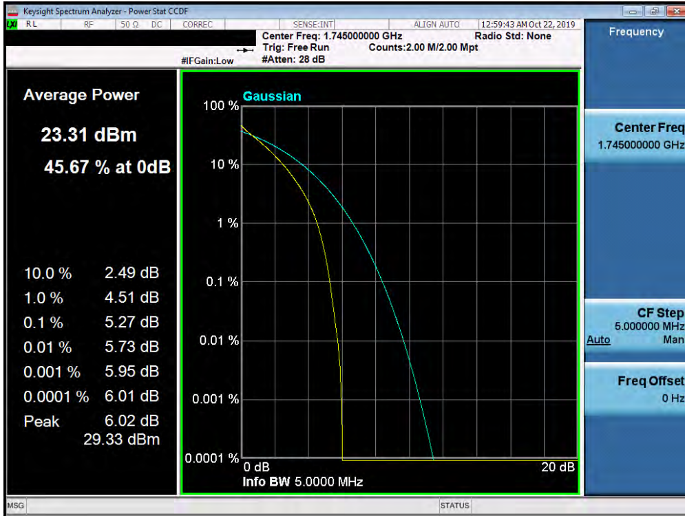
Plot 7-438. PAR Plot (Band 66/4 - 5.0MHz QPSK - Full RB Configuration)
