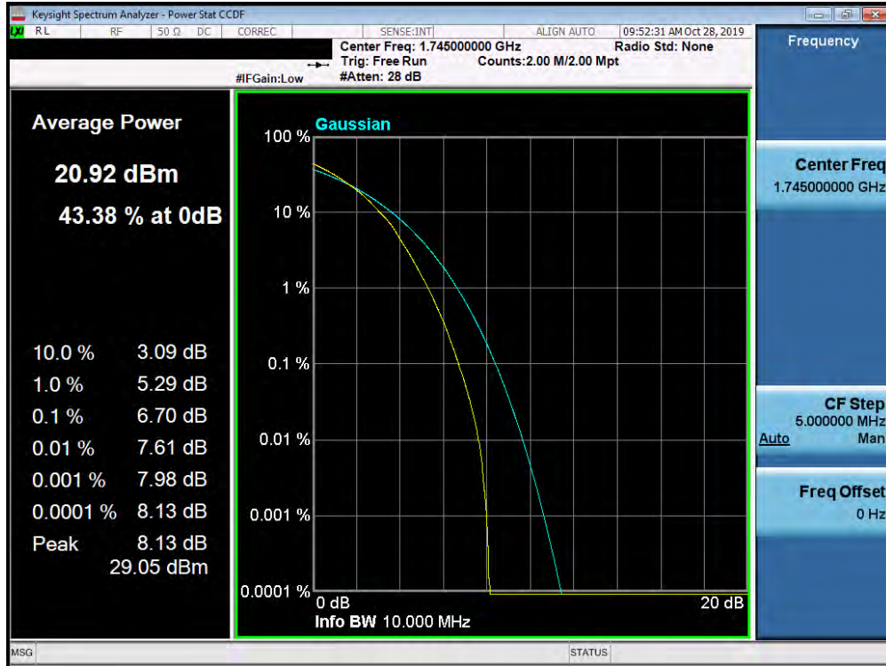
Plot 7-444. PAR Plot (Band 66/4 - 10.0MHz 64-QAM - Full RB Configuration)
