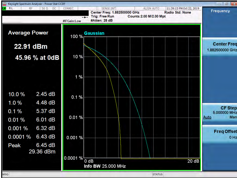
Plot 7-422. PAR Plot (Band 25/2 - 15.0MHz QPSK - Full RB Configuration)
