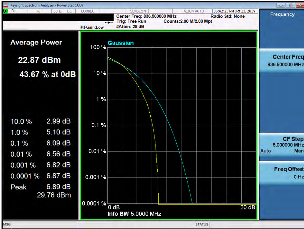
Plot 7-399. PAR Plot (Band 5 – 5.0MHz 16-QAM - Full RB Configuration)
