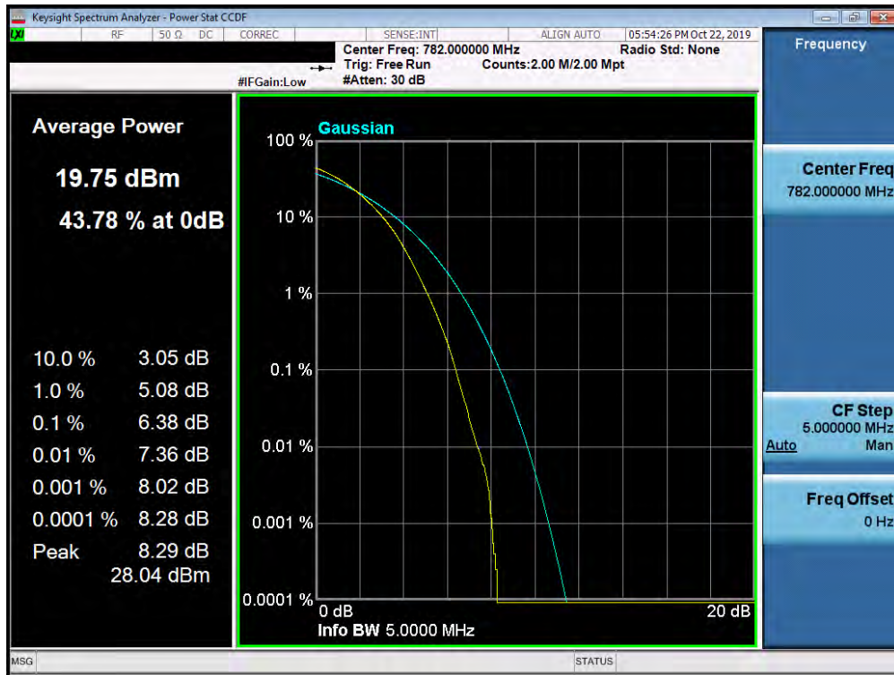
Plot 7-385. PAR Plot (Band 13 – 5.0MHz 256-QAM - Full RB Configuration)
