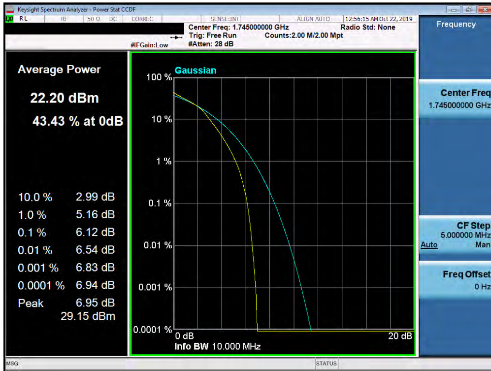
Plot 7-443. PAR Plot (Band 66/4 - 10.0MHz 16-QAM - Full RB Configuration)
