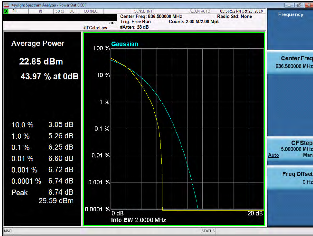
Plot 7-390. PAR Plot (Band 5 – 1.4MHz QPSK - Full RB Configuration)
