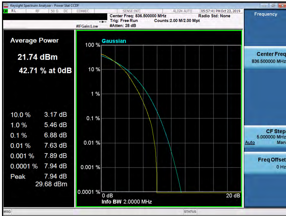
Plot 7-392. PAR Plot (Band 5 – 1.4MHz 64-QAM - Full RB Configuration)
