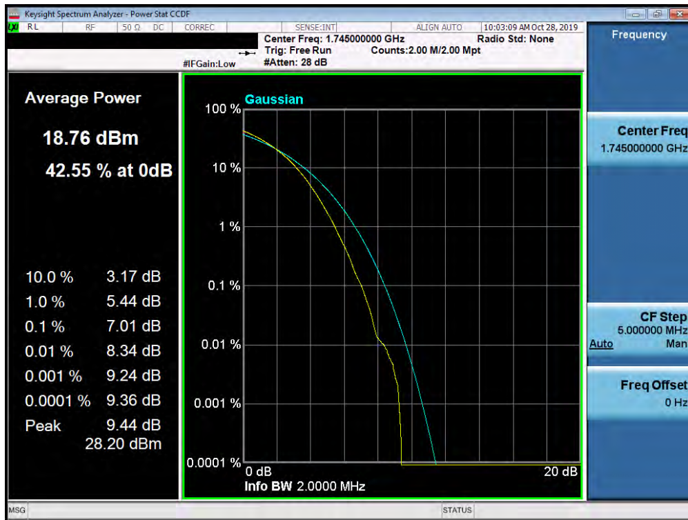
Plot 7-433. PAR Plot (Band 66/4 - 1.4MHz 256-QAM - Full RB Configuration)
