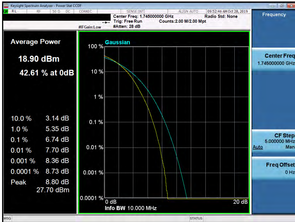
Plot 7-445. PAR Plot (Band 66/4 - 10.0MHz 256-QAM - Full RB Configuration)
