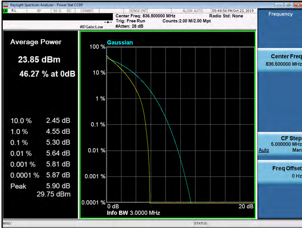
Plot 7-394. PAR Plot (Band 5 – 3.0MHz QPSK - Full RB Configuration)
