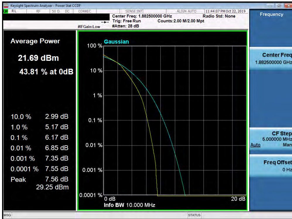
Plot 7-419. PAR Plot (Band 25/2 - 10.0MHz 16-QAM - Full RB Configuration)
