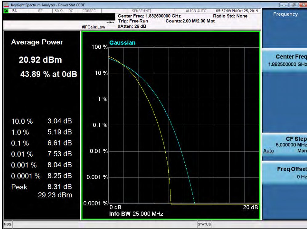
Plot 7-424. PAR Plot (Band 25/2 - 15.0MHz 64-QAM - Full RB Configuration)
