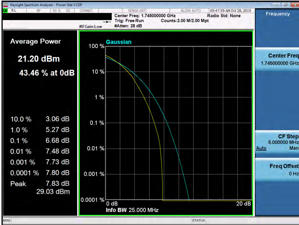
Plot 7-448. PAR Plot (Band 66/4 - 15.0MHz 64-QAM - Full RB Configuration)
