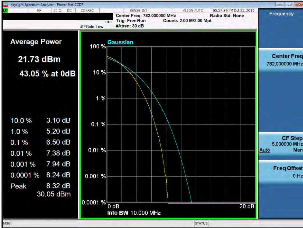
Plot 7-388. PAR Plot (Band 13 – 10.0MHz 64-QAM - Full RB Configuration)
