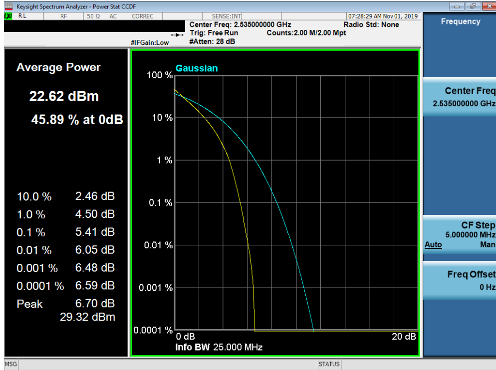
Plot 7-474. PAR Plot (Band 7 – 20.0MHz QPSK - Full RB Configuration)
