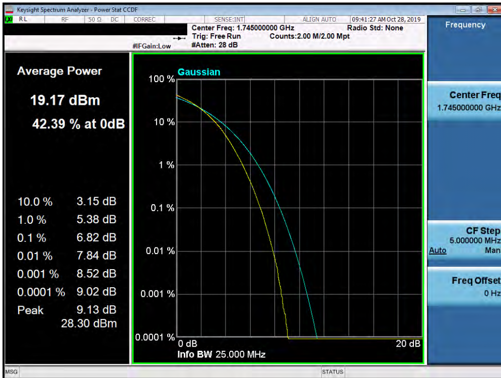
Plot 7-453. PAR Plot (Band 66/4 - 20.0MHz 256-QAM - Full RB Configuration)
