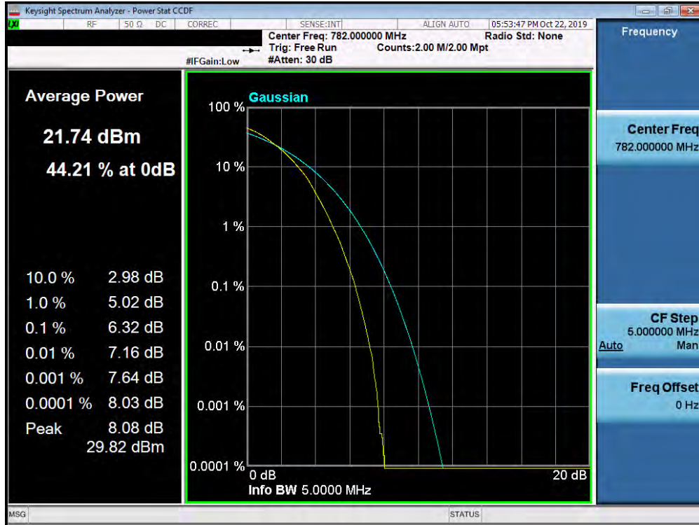
Plot 7-384. PAR Plot (Band 13 – 5.0MHz 64-QAM - Full RB Configuration)
