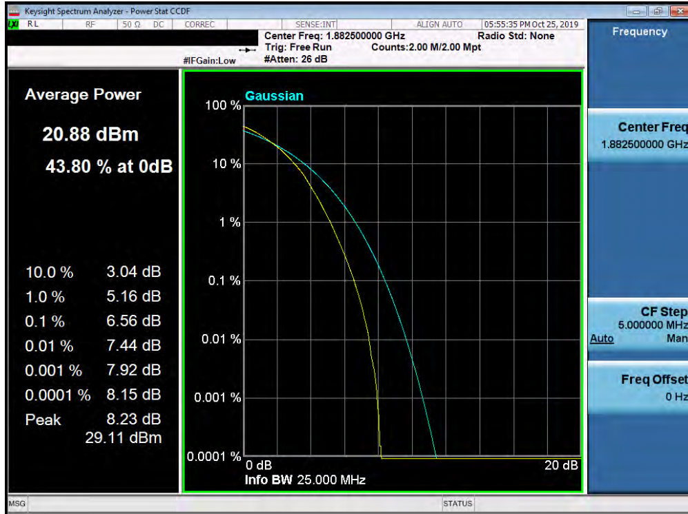
Plot 7-428. PAR Plot (Band 25/2 - 20.0MHz 64-QAM - Full RB Configuration)
