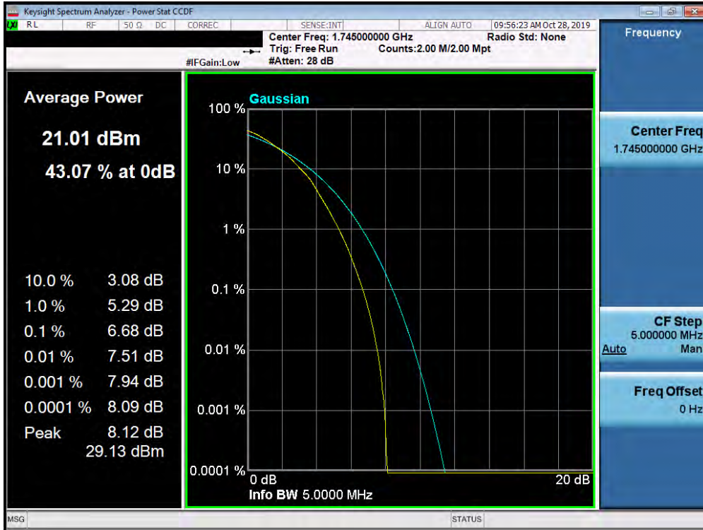
Plot 7-440. PAR Plot (Band 66/4 - 5.0MHz 64-QAM - Full RB Configuration)
