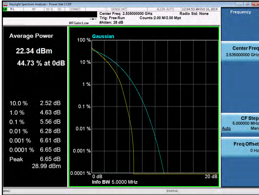
Plot 7-462. PAR Plot (Band 7 – 5.0MHz QPSK - Full RB Configuration)
