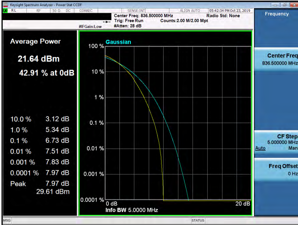
Plot 7-400. PAR Plot (Band 5 – 5.0MHz 64-QAM - Full RB Configuration)
