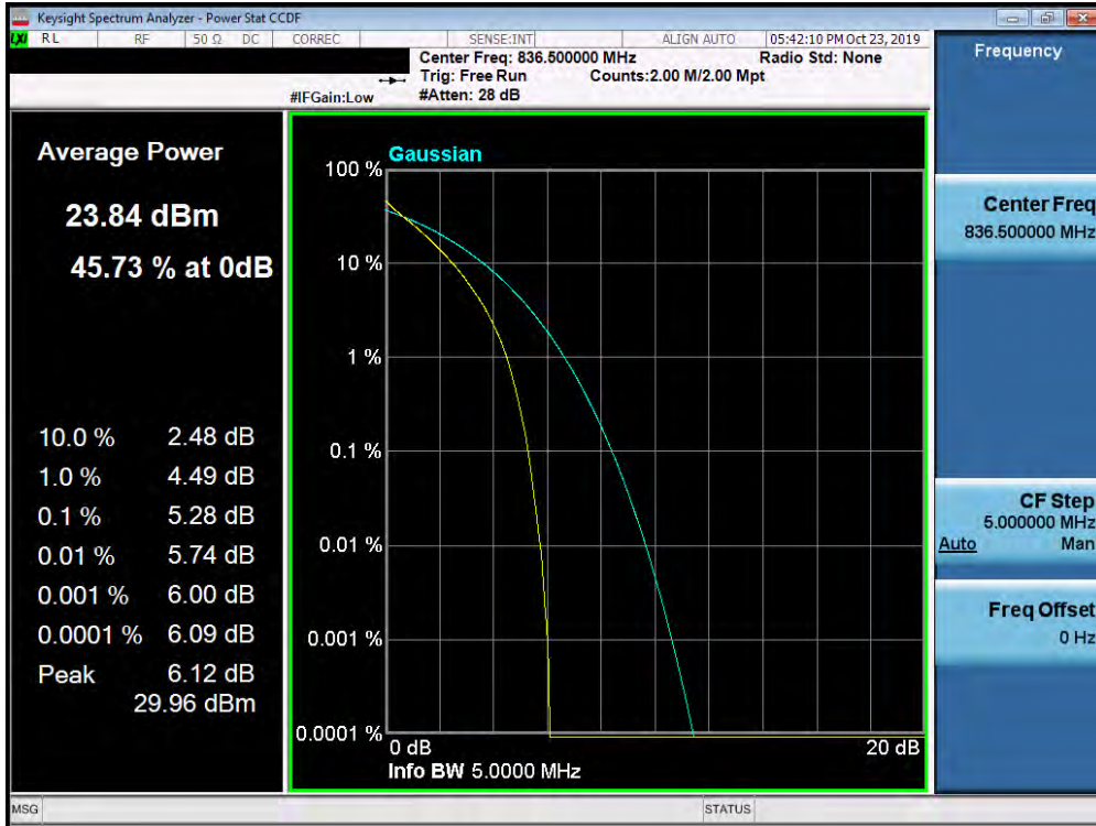
Plot 7-398. PAR Plot (Band 5 – 5.0MHz QPSK - Full RB Configuration)
