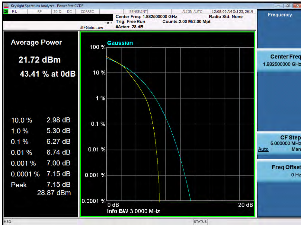
Plot 7-411. PAR Plot (Band 25/2 - 3.0MHz 16-QAM - Full RB Configuration)
