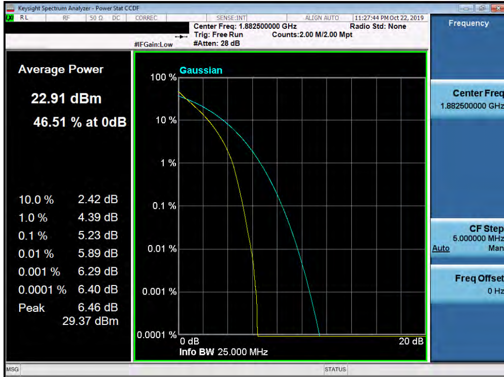
Plot 7-426. PAR Plot (Band 25/2 - 20.0MHz QPSK - Full RB Configuration)
