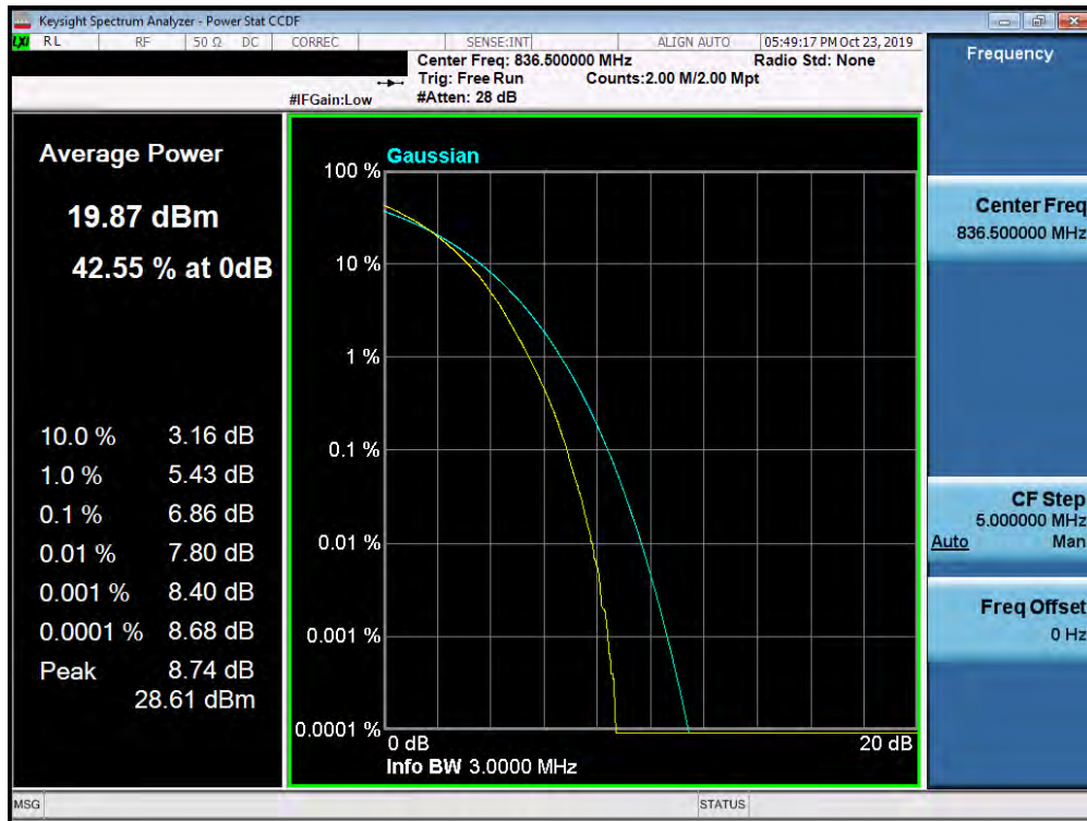
Plot 7-397. PAR Plot (Band 5 – 3.0MHz 256-QAM - Full RB Configuration)
