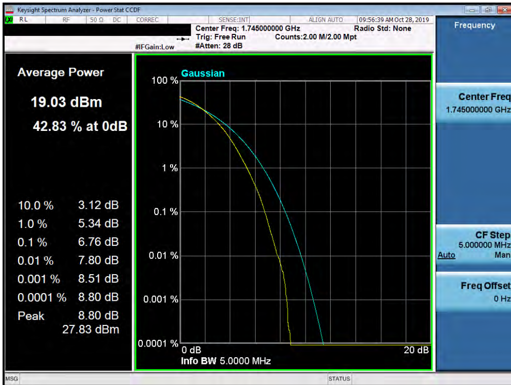
Plot 7-441. PAR Plot (Band 66/4 - 5.0MHz 256-QAM - Full RB Configuration)
