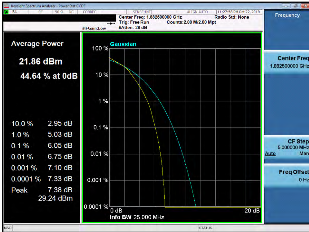
Plot 7-427. PAR Plot (Band 25/2 - 20.0MHz 16-QAM - Full RB Configuration)
