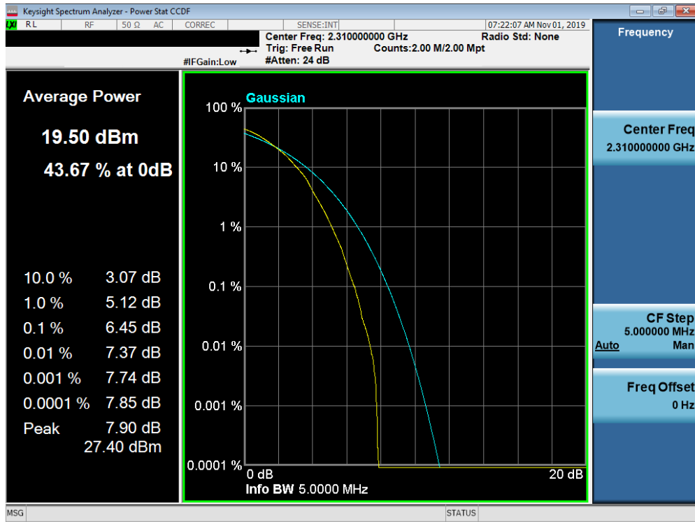
Plot 7-456. PAR Plot (Band 30 – 5.0MHz 64-QAM - Full RB Configuration)
