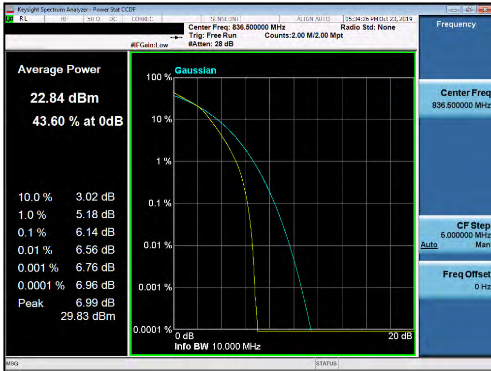
Plot 7-403. PAR Plot (Band 5 – 10.0MHz 16-QAM - Full RB Configuration)
