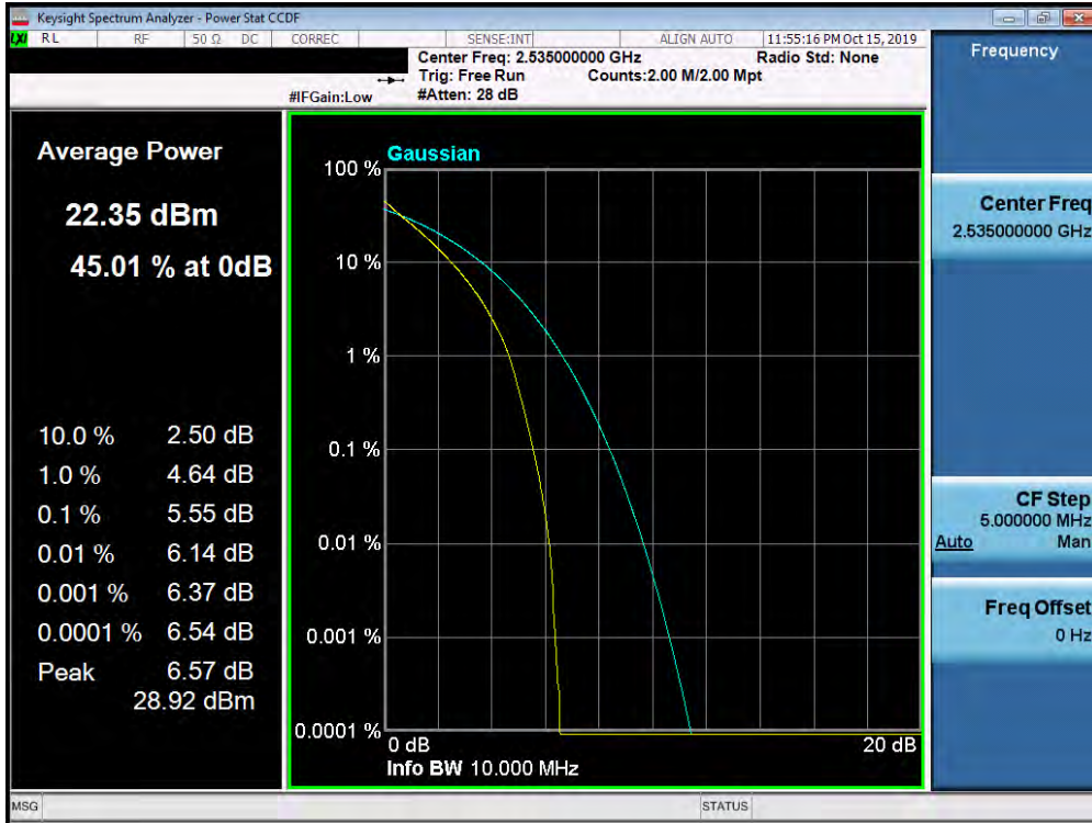
Plot 7-466. PAR Plot (Band 7 – 10.0MHz QPSK - Full RB Configuration)
