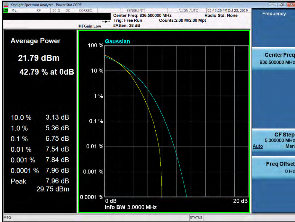
Plot 7-396. PAR Plot (Band 5 – 3.0MHz 64-QAM - Full RB Configuration)
