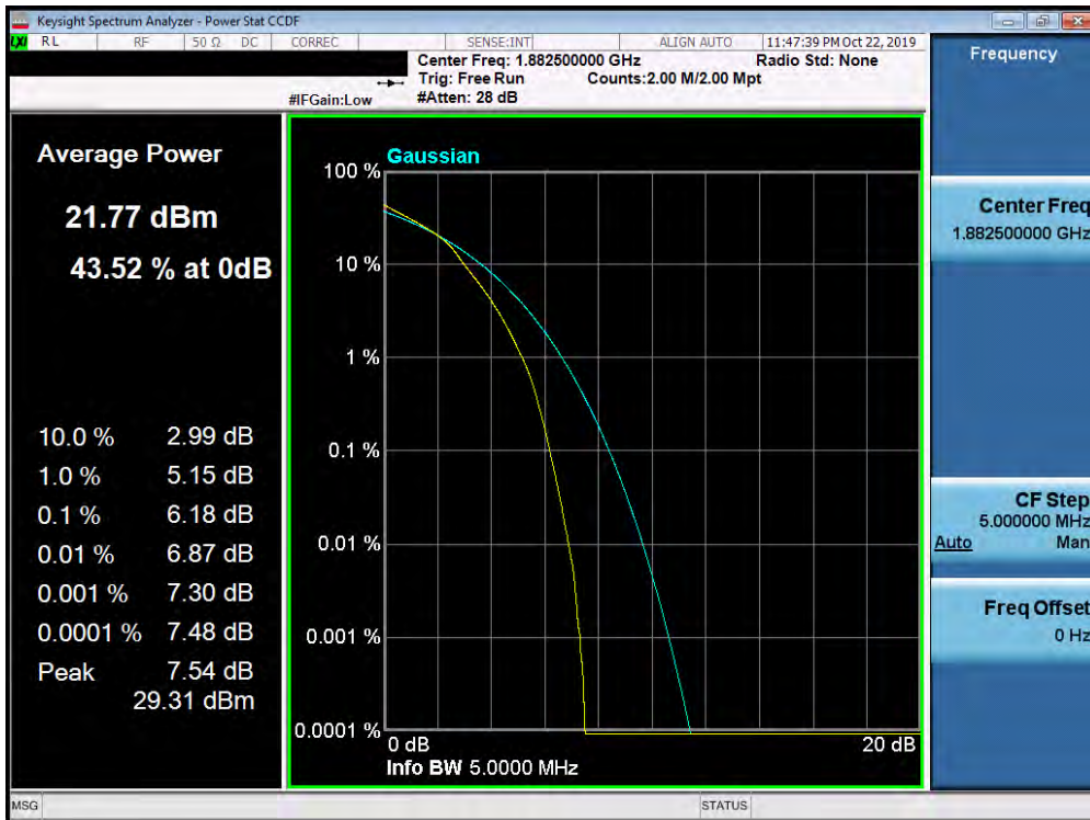
Plot 7-415. PAR Plot (Band 25/2 - 5.0MHz 16-QAM - Full RB Configuration)
