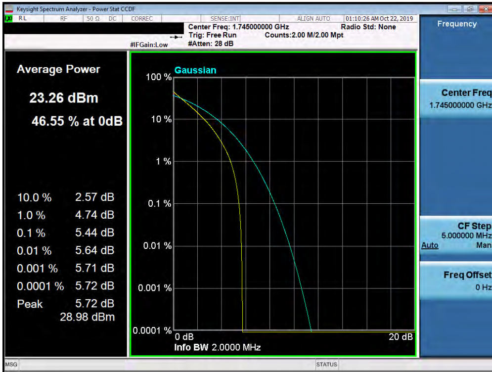
Plot 7-430. PAR Plot (Band 66/4 - 1.4MHz QPSK - Full RB Configuration)
