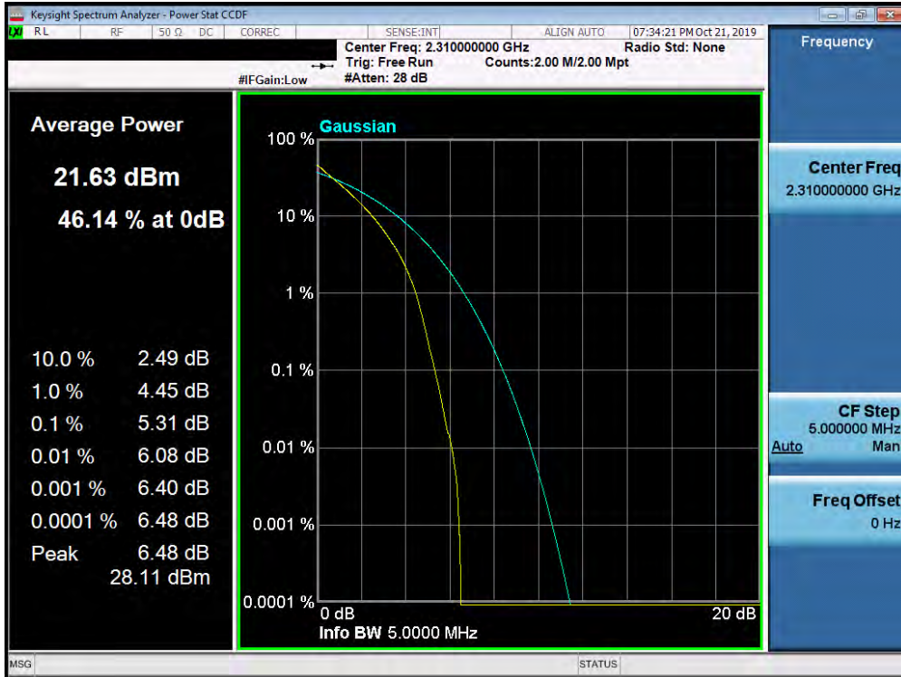
Plot 7-454. PAR Plot (Band 30 – 5.0MHz QPSK - Full RB Configuration)
