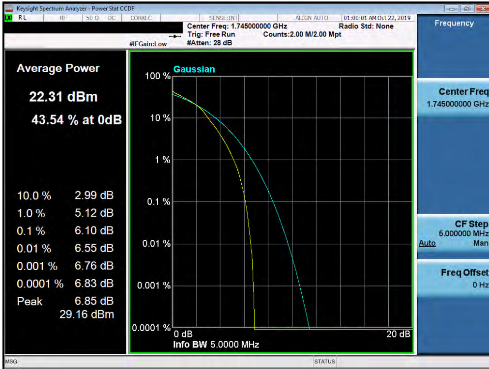
Plot 7-439. PAR Plot (Band 66/4 - 5.0MHz 16-QAM - Full RB Configuration)
