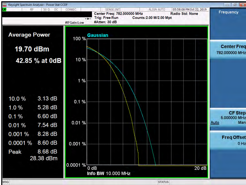
Plot 7-389. PAR Plot (Band 13 – 10.0MHz 256-QAM - Full RB Configuration)
