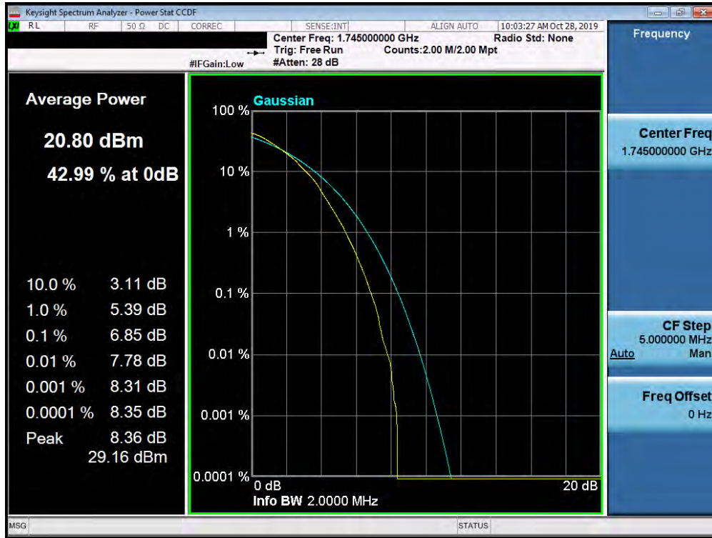
Plot 7-432. PAR Plot (Band 66/4 - 1.4MHz 64-QAM - Full RB Configuration)
