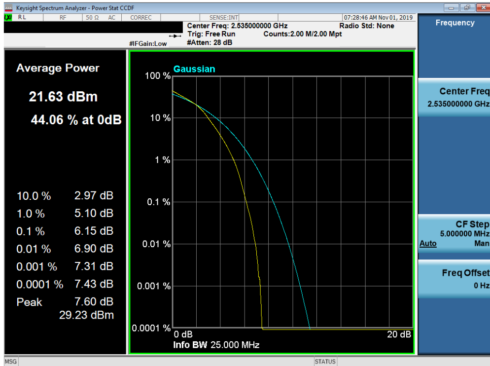
Plot 7-475. PAR Plot (Band 7 – 20.0MHz 16-QAM - Full RB Configuration)
