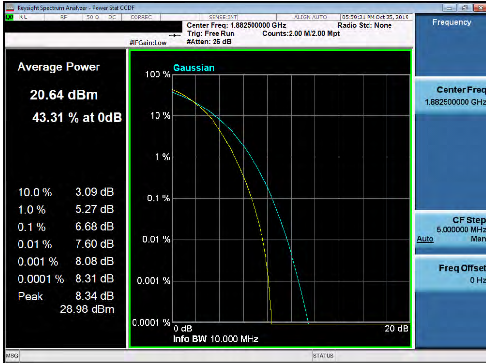
Plot 7-420. PAR Plot (Band 25/2 - 10.0MHz 64-QAM - Full RB Configuration)
