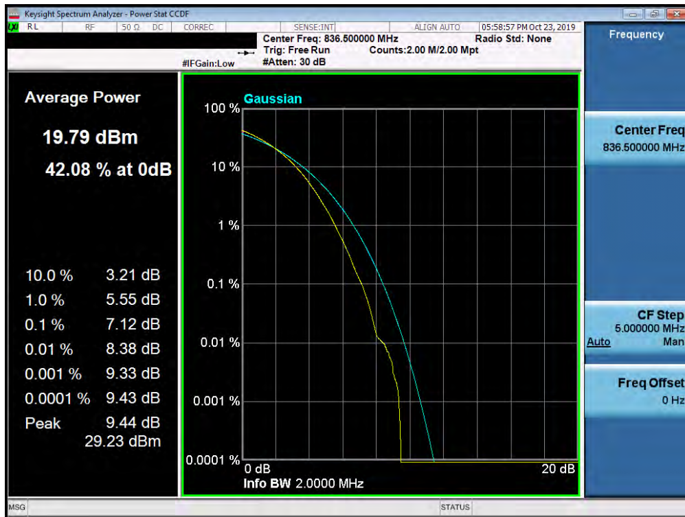
Plot 7-393. PAR Plot (Band 5 – 1.4MHz 256-QAM - Full RB Configuration)
