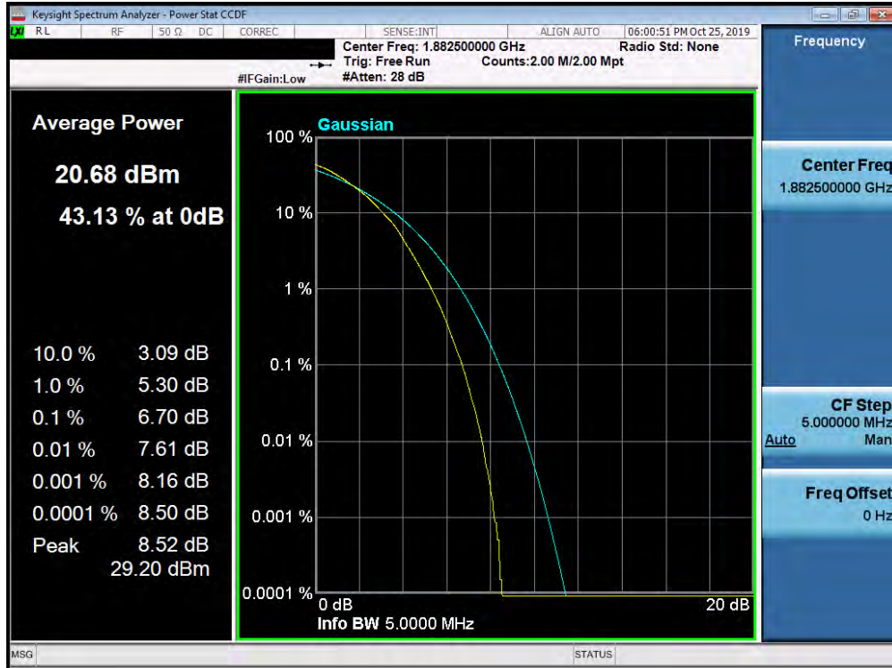
Plot 7-416. PAR Plot (Band 25/2 - 5.0MHz 64-QAM - Full RB Configuration)
