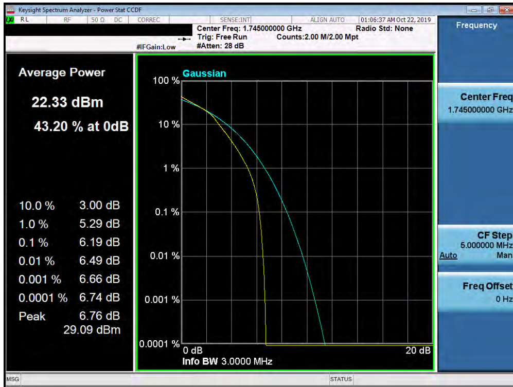
Plot 7-435. PAR Plot (Band 66/4 - 3.0MHz 16-QAM - Full RB Configuration)
