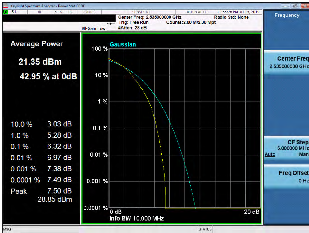
Plot 7-467. PAR Plot (Band 7 – 10.0MHz 16-QAM - Full RB Configuration)
