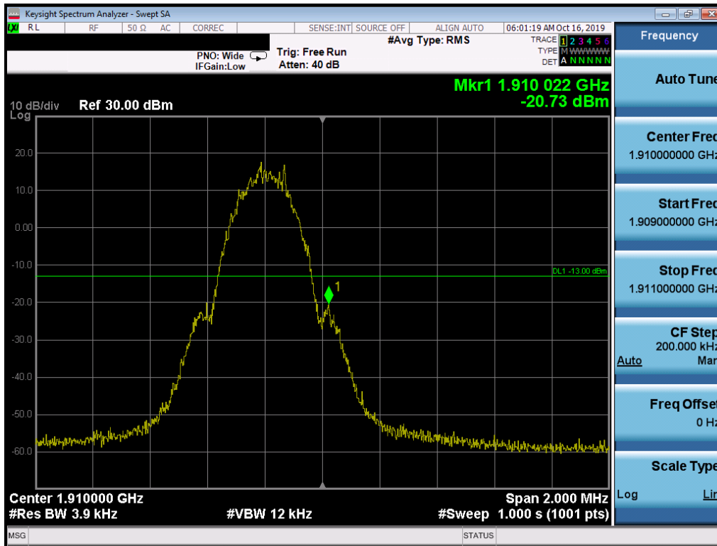
Plot 7-77. Band Edge Plot (PCS GSM Mode - High Channel)
