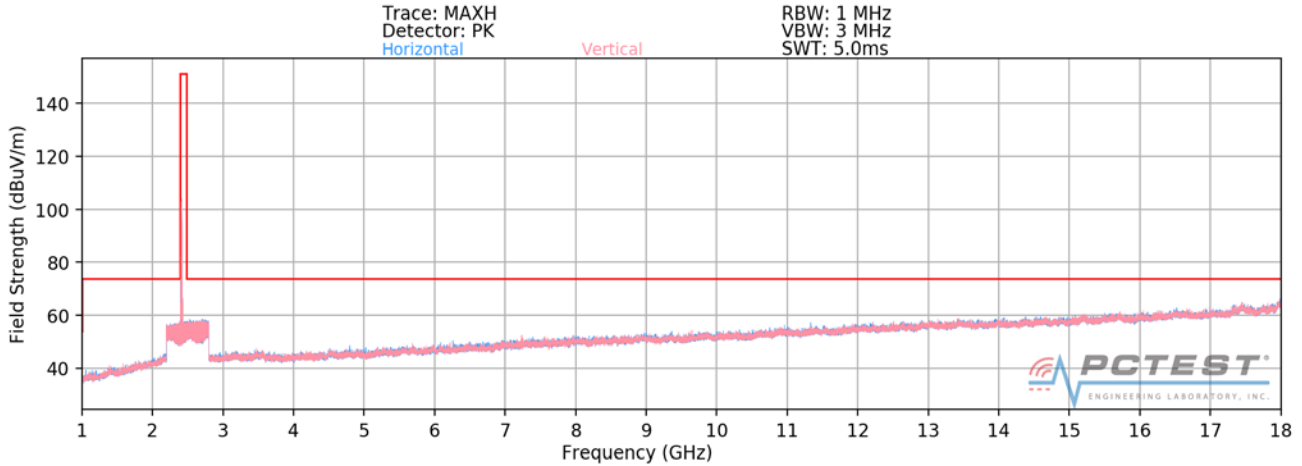
Plot 7-95. Radiated Spurious Plot above 1GHz SISO ANT2 (802.11b – Ch. 1)
