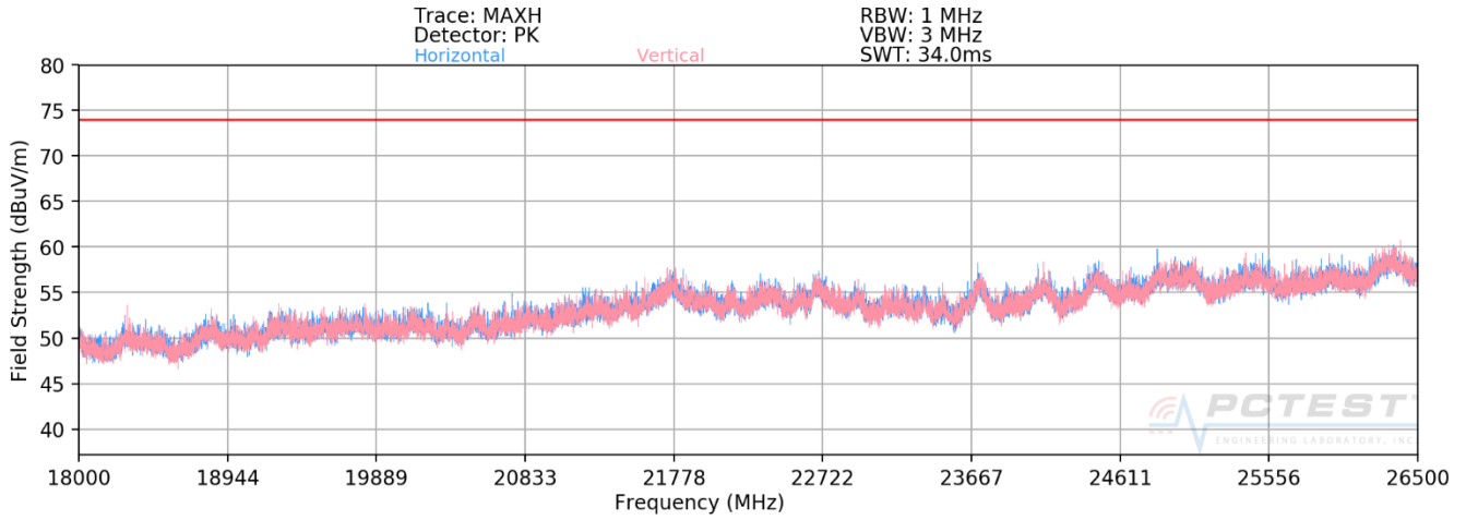
Plot 7-77. Radiated Spurious Plot above 18GHz SISO ANT1 (802.11ax OFDMA – 106 Tones)
