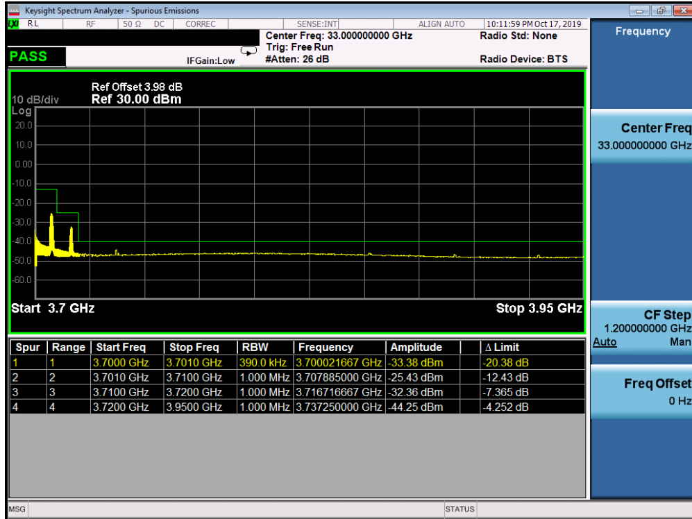
Plot 7-47. Conducted Spurious Plot (LTE Band 48 - 20.0MHz QPSK - RB Size 1, RB Offset 99 - High Channel)
