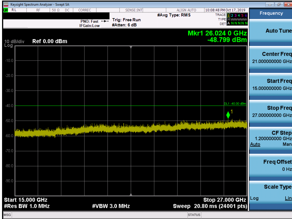
Plot 7-49. Conducted Spurious Plot (LTE Band 48 - 20.0MHz QPSK - RB Size 1, RB Offset 99- High Channel)
