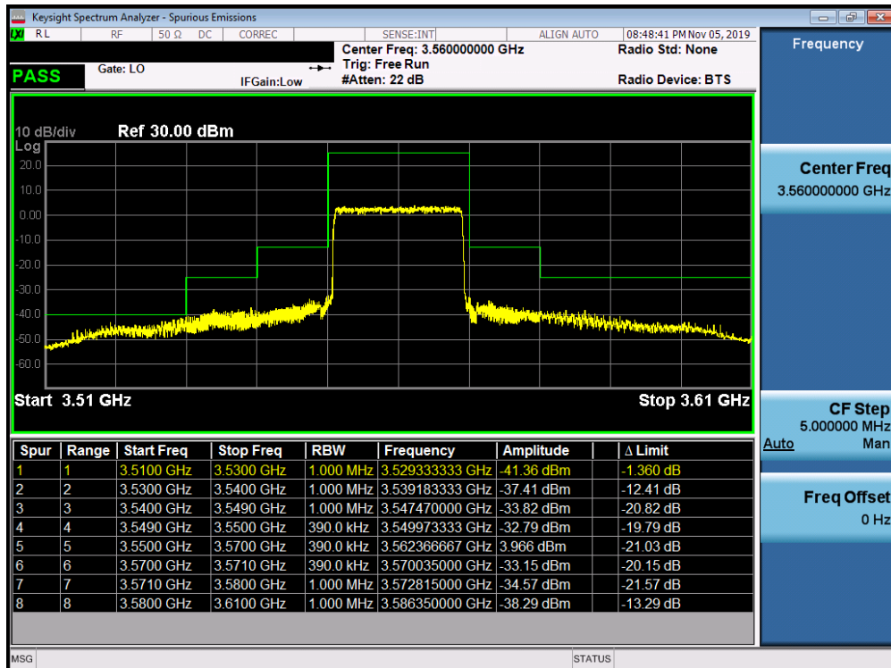
Plot 7-60. Lower ACP Plot (LTE Band 48 - 20.0MHz QPSK - Full RB Configuration)
