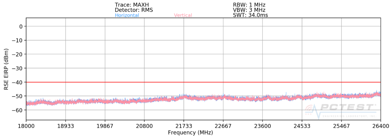
Plot 7-89. Radiated Spurious Plot 18GHz – 26.5GHz (ULCA Band 48)
