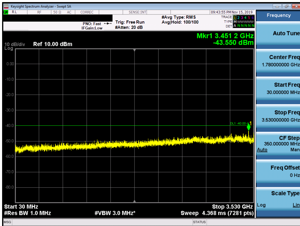
Plot 7-75. Conducted Spurious Plot (Band 48 – 20.0MHz QPSK – PCC 1/0 SCC 1/99 – High Channel)
