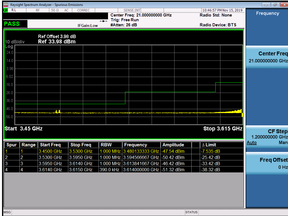
Plot 7-70. Conducted Spurious Plot (Band 48 – 20.0MHZ QPSK – PCC 1/99 SCC 1/0 – Mid Channel)
