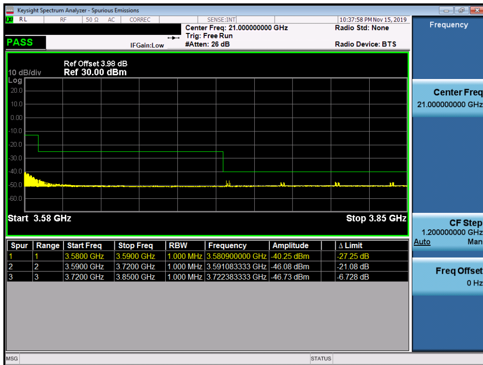
Plot 7-65. Conducted Spurious Plot (Band 48 – 20.0MHz QPSK – PCC 1/99 SCC 1/0 – Low Channel)
