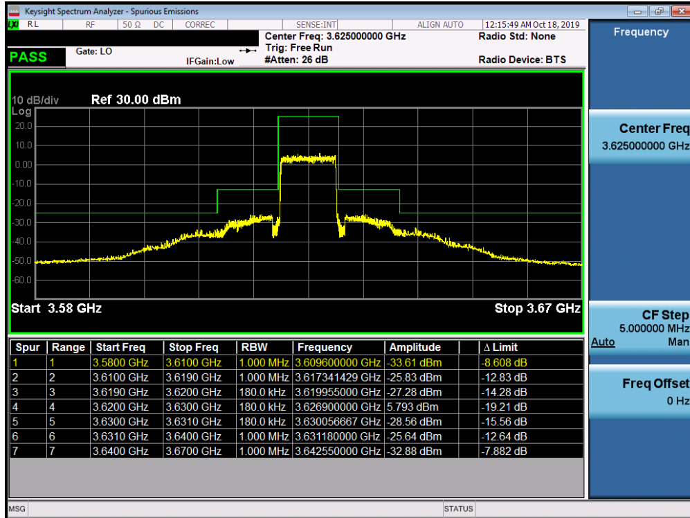
Plot 7-55. Mid ACP Plot (LTE Band 48 - 10.0MHz QPSK - Full RB Configuration)
