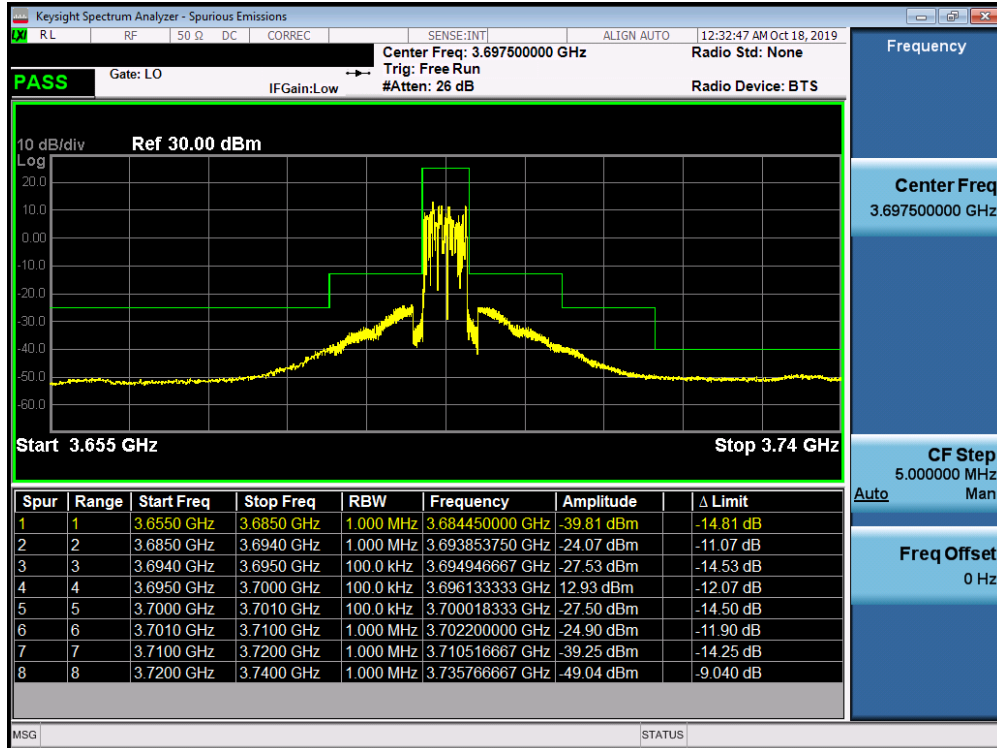
Plot 7-53. Upper ACP Plot (LTE Band 48 - 5.0MHz QPSK - Full RB Configuration)
