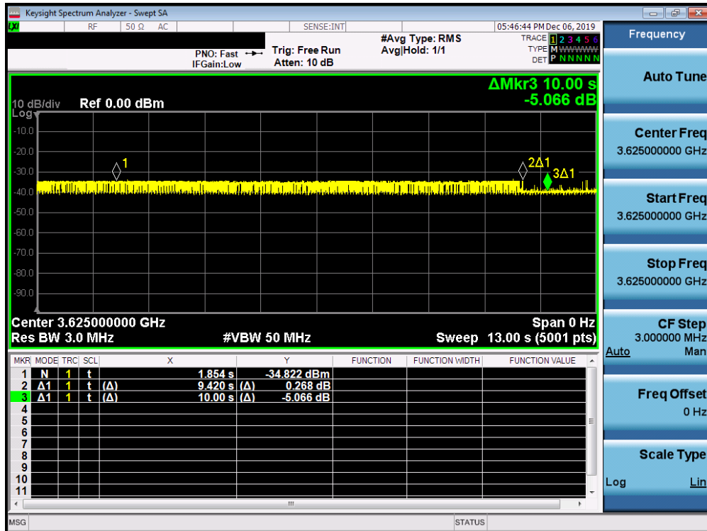
Plot 7-91. Run#1 End User Device Discontinues Operations within 10s
