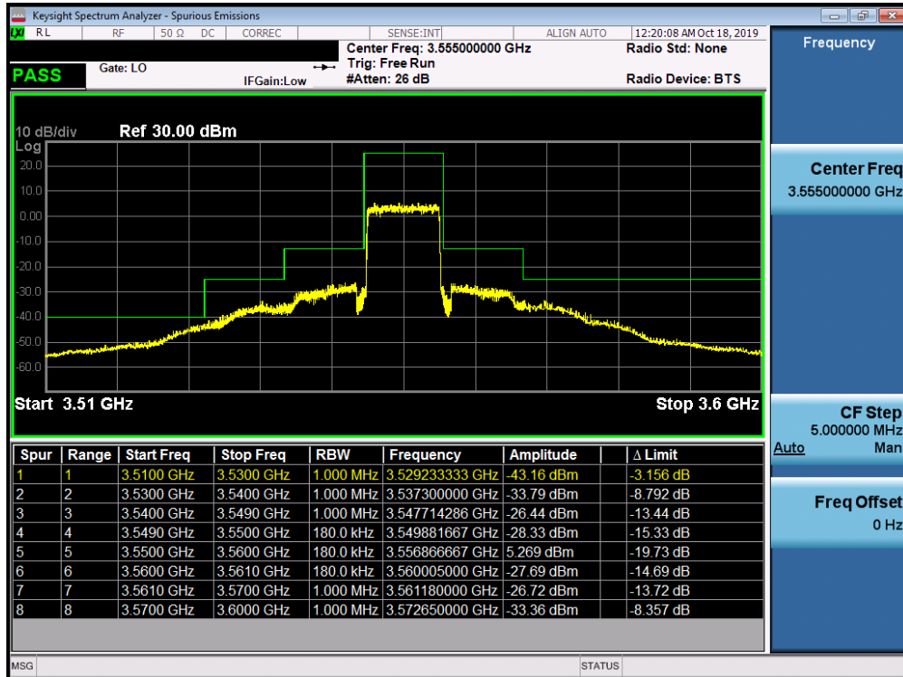
Plot 7-54. Lower ACP Plot (LTE Band 48 - 10.0MHz QPSK - Full RB Configuration)
