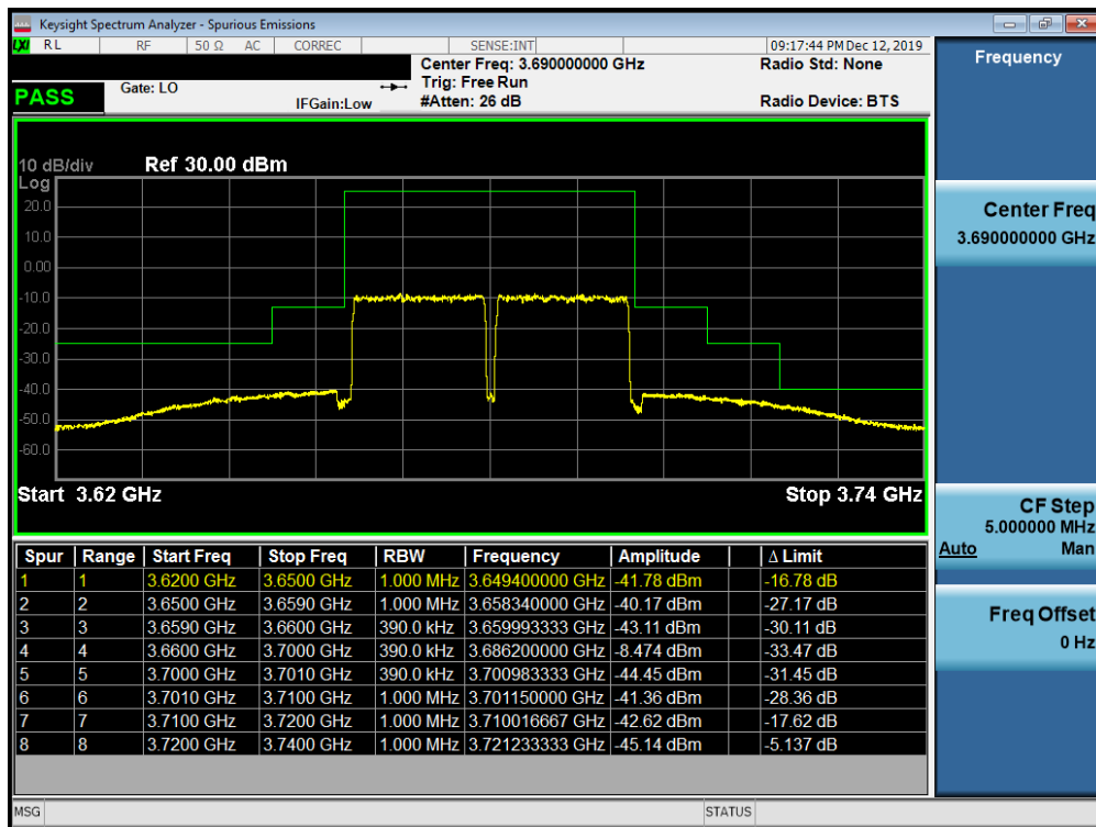
Plot 7-83. Upper Band Edge Plot (Band 48 QPSK – PCC:20 MHz SCC:20 MHz – Full RB)
