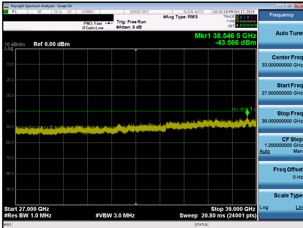
Plot 7-50. Conducted Spurious Plot (LTE Band 48 - 20.0MHz QPSK - RB Size 1, RB Offset 99 - High Channel)
