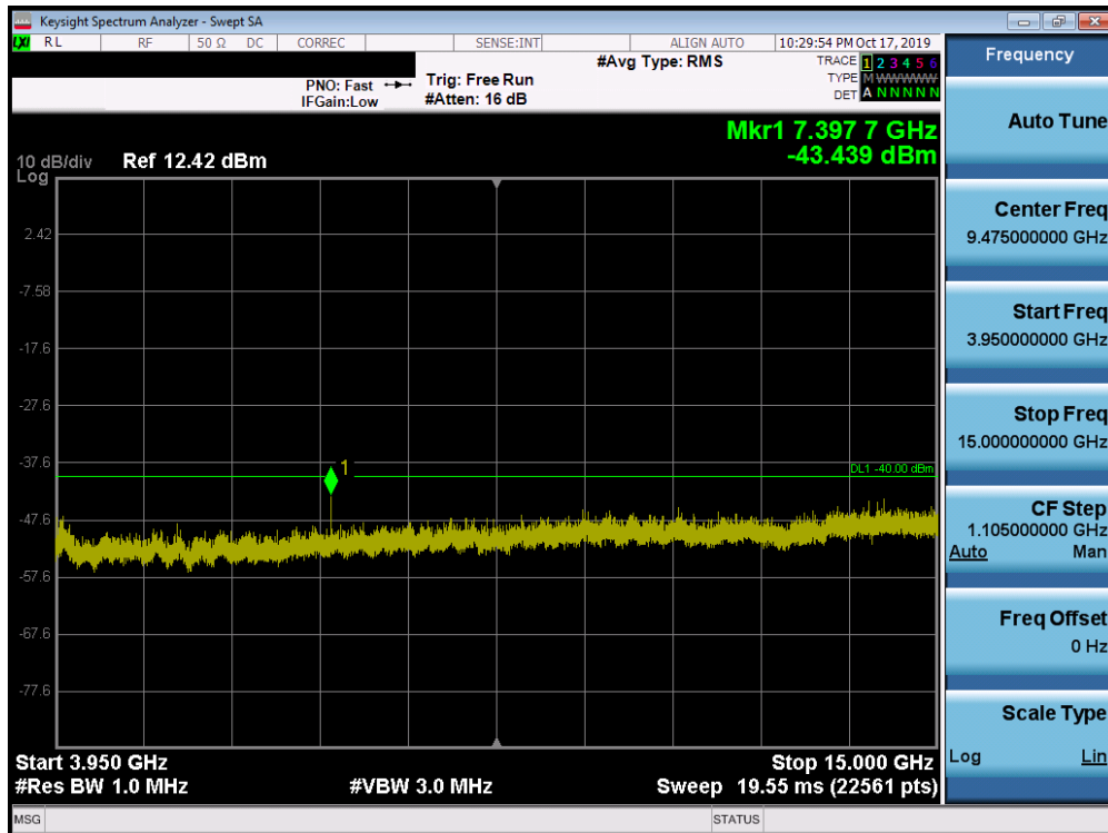
Plot 7-48. Conducted Spurious Plot (LTE Band 48 - 20.0MHz QPSK - RB Size 1, RB Offset 99- High Channel)
