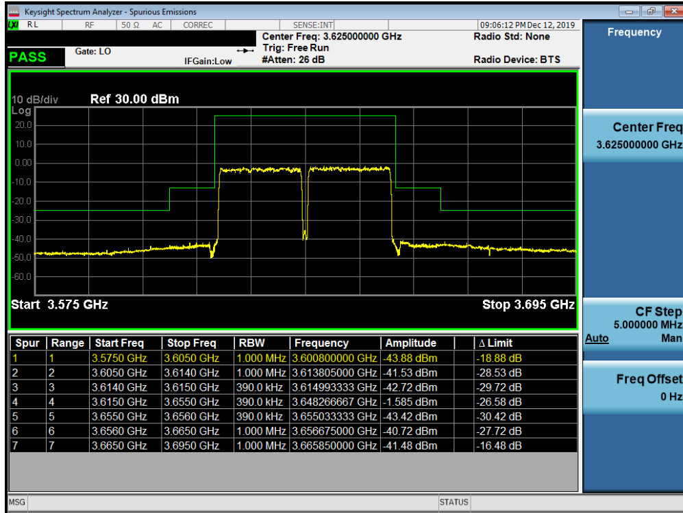
Plot 7-82. Mid Band Edge Plot (Band 48 QPSK – PCC:20 MHz SCC:20 MHz – Full RB)
