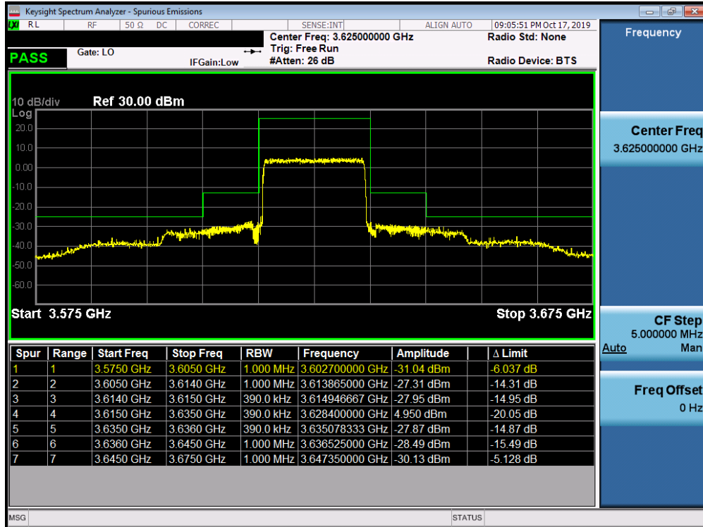
Plot 7-61. Mid ACP Plot (LTE Band 48 - 20.0MHz QPSK - Full RB Configuration)
