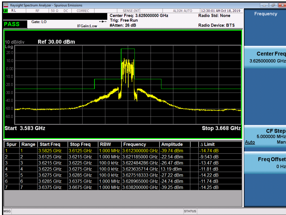
Plot 7-52. Mid ACP Plot (LTE Band 48 - 5.0MHz QPSK - Full RB Configuration)
