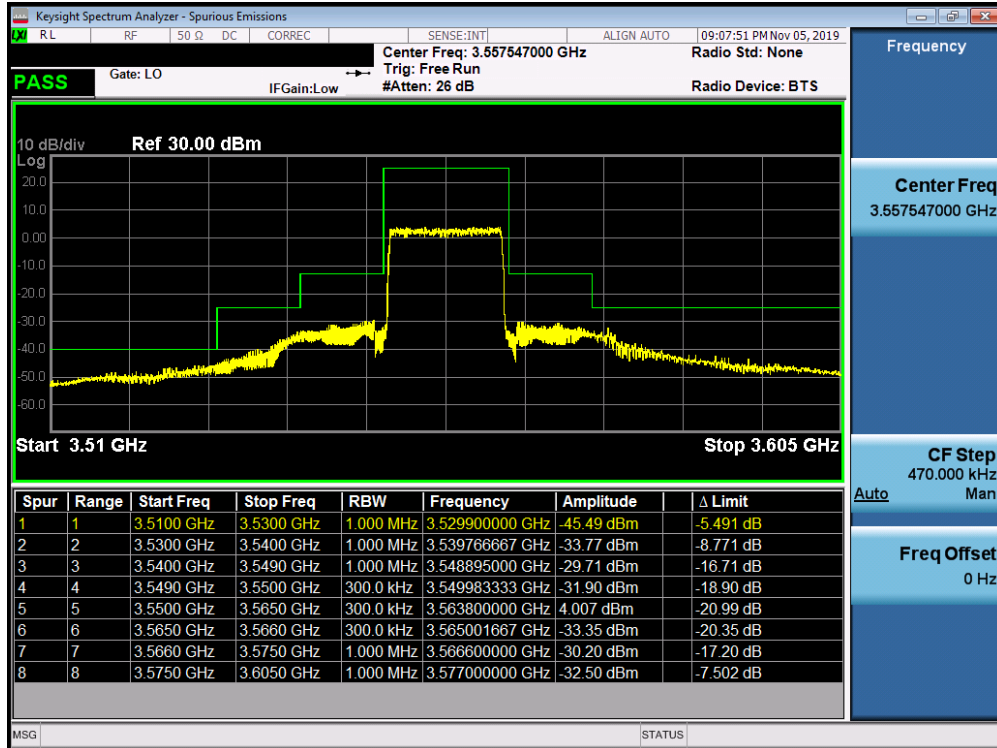
Plot 7-57. Lower ACP Plot (LTE Band 48 - 15.0MHz QPSK - Full RB Configuration)
