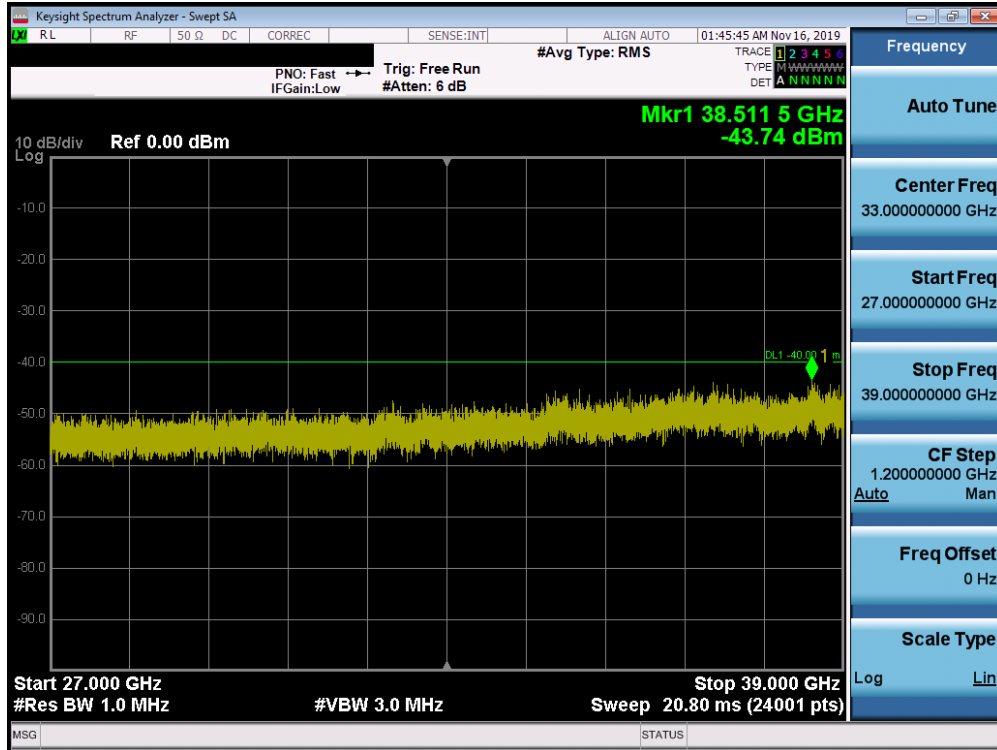
Plot 7-80. Conducted Spurious Plot (Band 48 – 20.0MHz QPSK – PCC 1/0 SCC 1/99 – High Channel)
