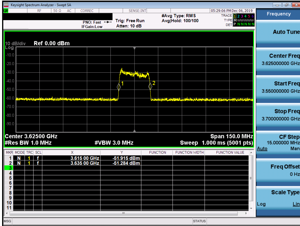
Plot 7-90. Run#1 End User Device Frequency of Operations
