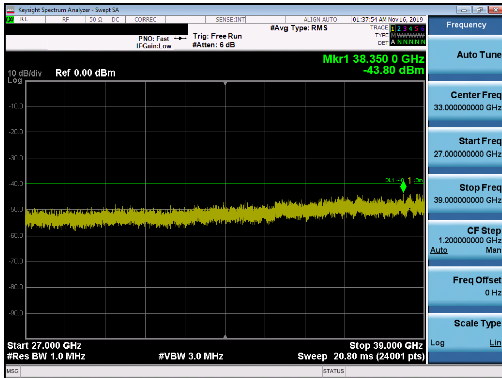
Plot 7-74. Conducted Spurious Plot (Band 48 – 20.0MHz QPSK – PCC 1/99 SCC 1/0 – Mid Channel)
