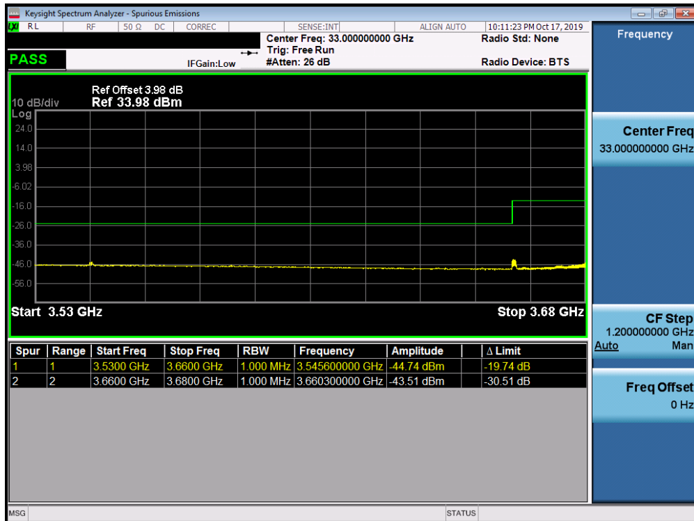
Plot 7-46. Conducted Spurious Plot (LTE Band 48 - 20.0MHz QPSK - RB Size 1, RB Offset 99- High Channel)
