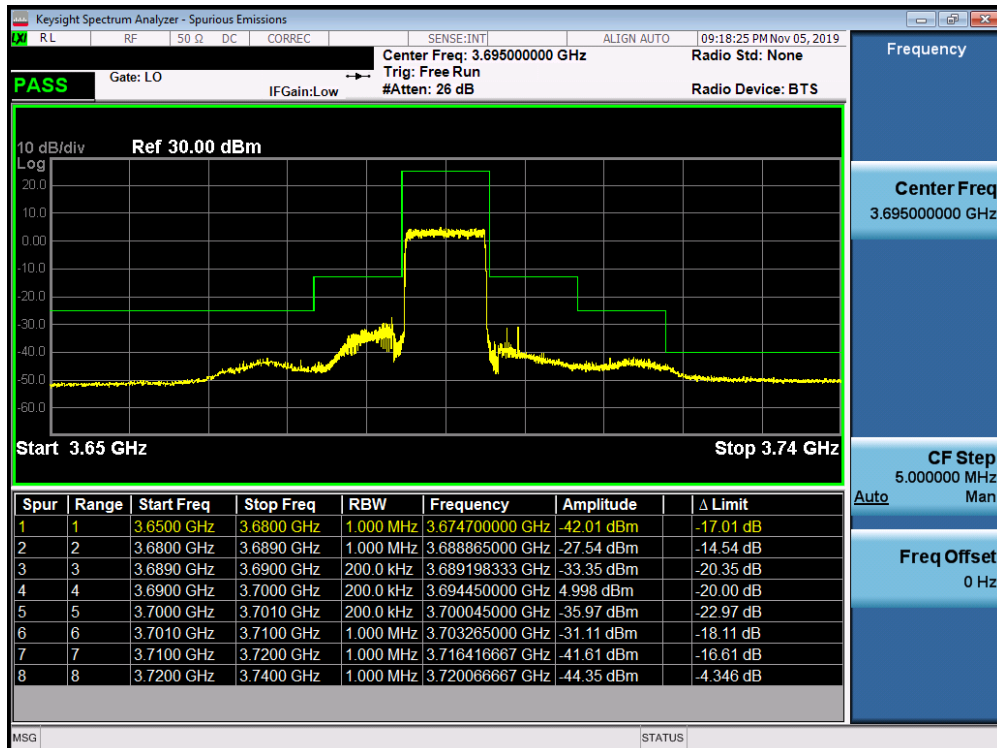
Plot 7-56. Upper ACP Plot (LTE Band 48 - 10.0MHz QPSK - Full RB Configuration)
