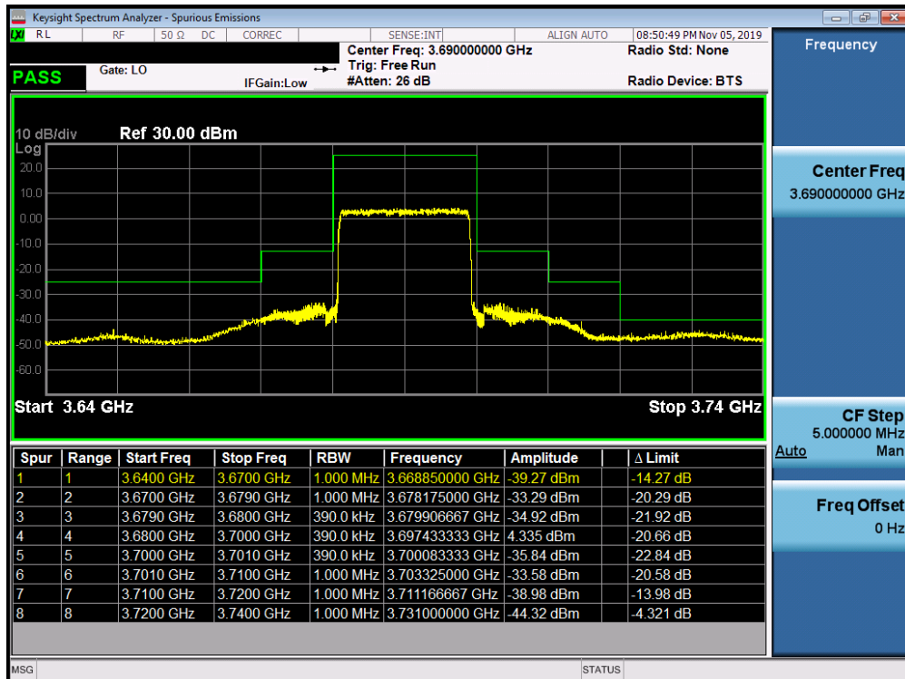
Plot 7-62. Upper ACP Plot (LTE Band 48 - 20.0MHz QPSK - Full RB Configuration)
