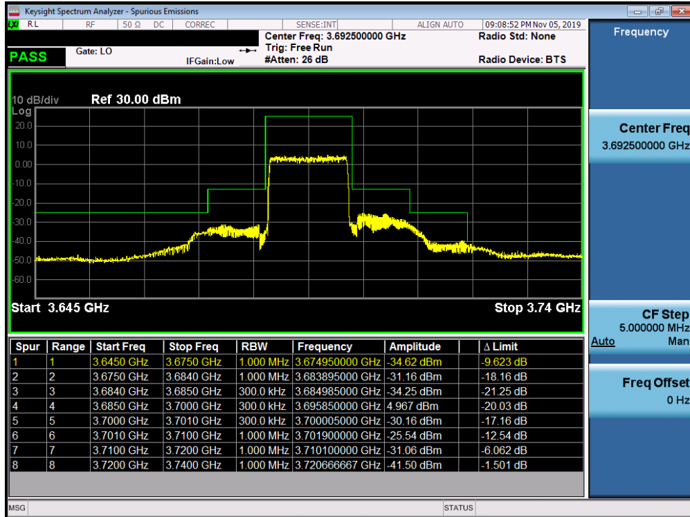
Plot 7-59. Upper ACP Plot (LTE Band 48 - 15.0MHz QPSK - Full RB Configuration)
