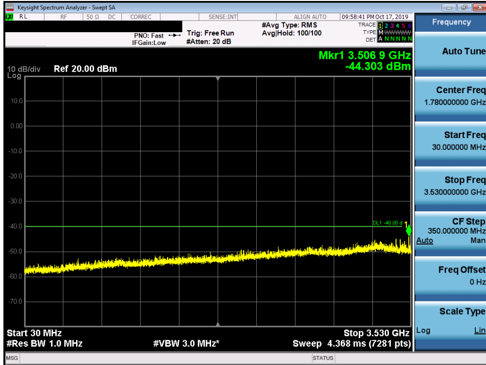
Plot 7-45. Conducted Spurious Plot (LTE Band 48 - 20.0MHz QPSK - RB Size 1, RB Offset 99- High Channel)
