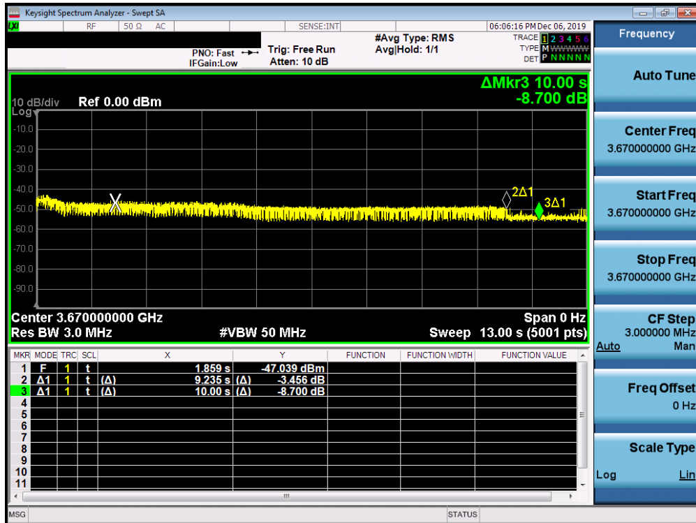
Plot 7-93. Run#2 End User Device Discontinues Operations within 10s
