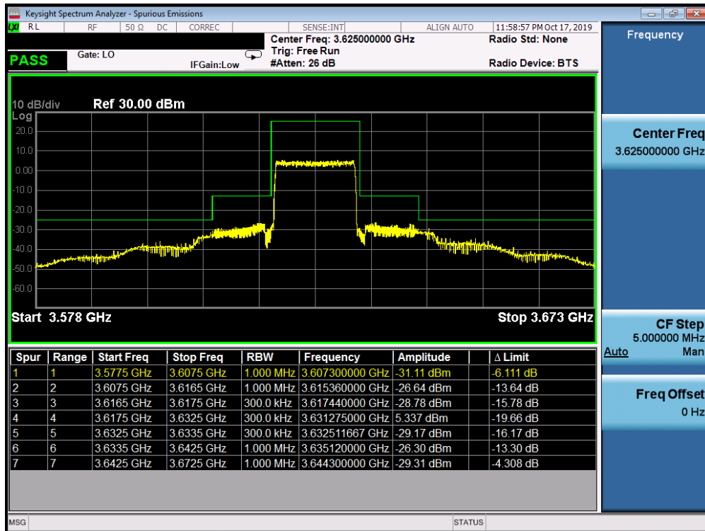
Plot 7-58. Mid ACP Plot (LTE Band 48 - 15.0MHz QPSK - Full RB Configuration)
