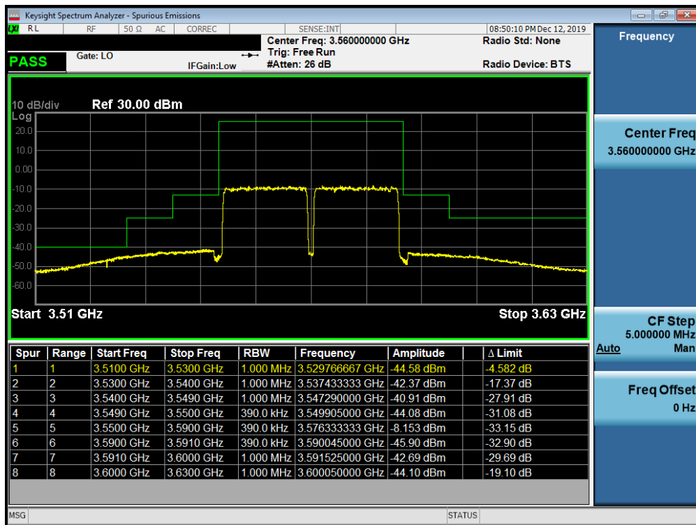
Plot 7-81. Lower Band Edge Plot (Band 48 QPSK – PCC:20 MHz SCC:20 MHz – Full RB)
