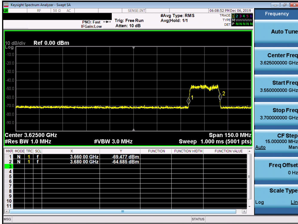
Plot 7-92. Run#2 End User Device Frequency of Operations
