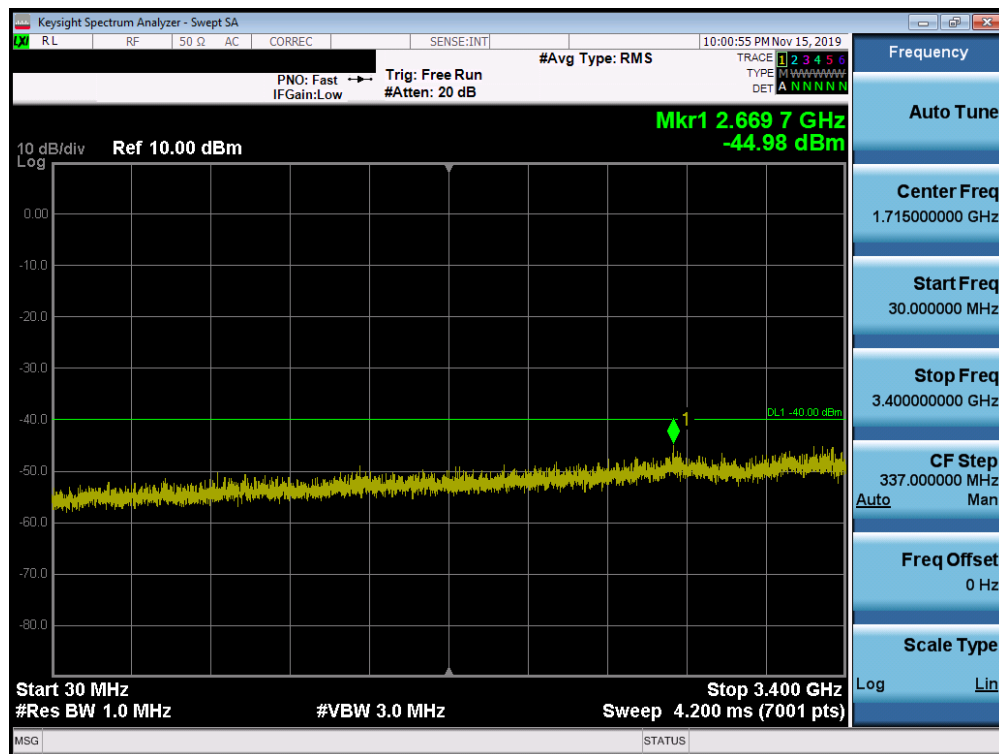
Plot 7-63. Conducted Spurious Plot (Band 48 – 20.0MHz QPSK – PCC 1/99 SCC 1/0 – Low Channel)
