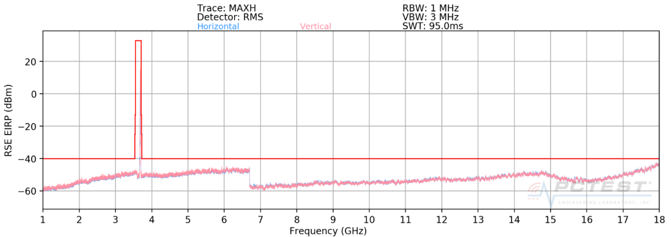
Plot 7-88. Radiated Spurious Plot 1GHz - 18GHz (ULCA Band 48) High Channel – PCC/SCC: 1RB)
