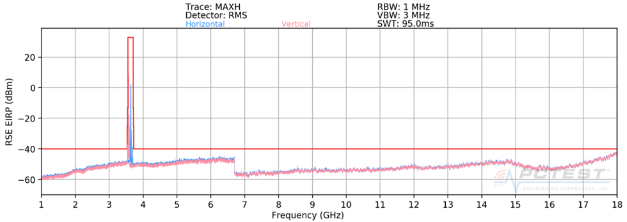
Plot 7-86. Radiated Spurious Plot 1GHz - 18GHz (ULCA Band 48) Low Channel – PCC/SCC: 1RB)
