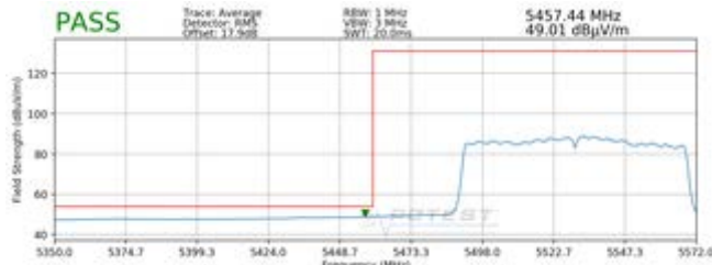
Plot 7-353. Radiated Band Edge Plot MIMO (Average – WCP)
