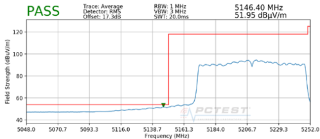
Plot 7-346. Radiated Lower Band Edge Plot MIMO (Average – UNII Band 1)
