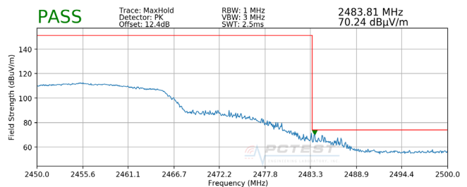
Plot 7-128. Radiated Restricted Upper Band Edge Measurement MIMO (Peak)
