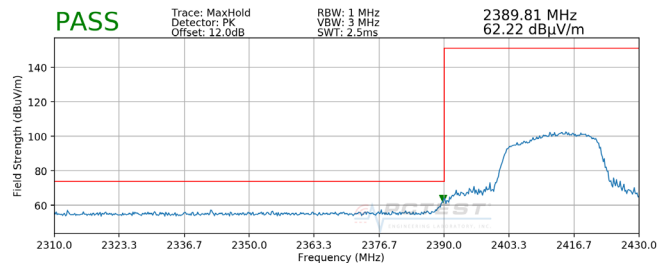
Plot 7-116. Radiated Restricted Lower Band Edge Measurement SISO ANT2 (Peak)
