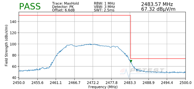
Plot 7-134. Radiated Restricted Upper Band Edge Measurement MIMO (Peak)
