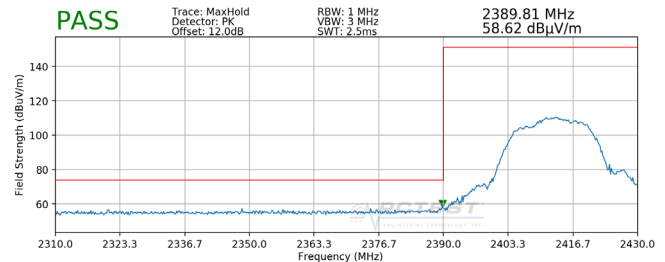
Plot 7-106. Radiated Restricted Lower Band Edge Measurement SISO ANT1 (Peak)
