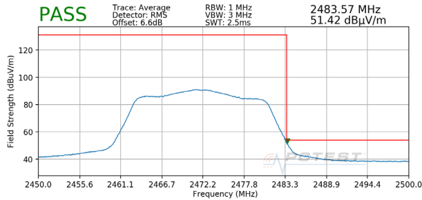
Plot 7-113. Radiated Restricted Upper Band Edge Measurement SISO ANT1 (Average)
