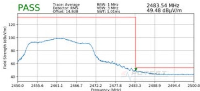
Plot 7-135. Radiated Restricted Band Edge Measurement MIMO with WCP (Average)
