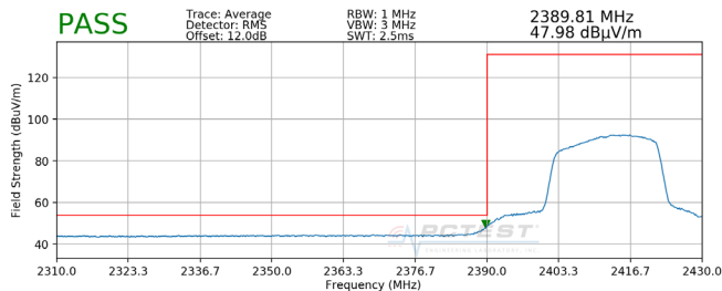
Plot 7-115. Radiated Restricted Lower Band Edge Measurement SISO ANT2 (Average)
