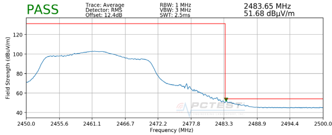
Plot 7-129. Radiated Restricted Upper Band Edge Measurement MIMO (Average)
