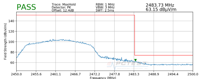
Plot 7-120. Radiated Restricted Upper Band Edge Measurement SISO ANT2 (Peak)
