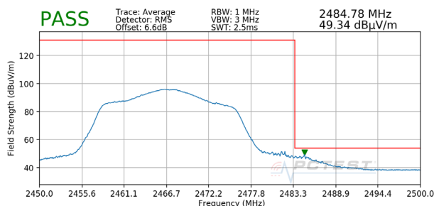
Plot 7-121. Radiated Restricted Upper Band Edge Measurement SISO ANT2 (Average)
