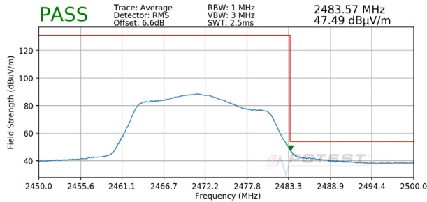
Plot 7-123. Radiated Restricted Upper Band Edge Measurement SISO ANT2 (Average)
