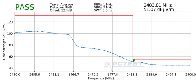
Plot 7-127. Radiated Restricted Upper Band Edge Measurement MIMO (Average)
