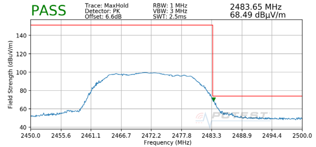
Plot 7-114. Radiated Restricted Upper Band Edge Measurement SISO ANT1 (Peak)
