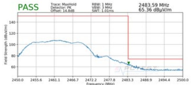
Plot 7-136. Radiated Restricted Band Edge Measurement MIMO with WCP (Peak)
