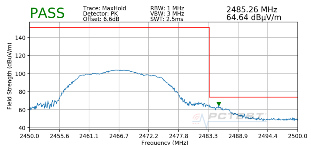
Plot 7-122. Radiated Restricted Upper Band Edge Measurement SISO ANT2 (Peak)
