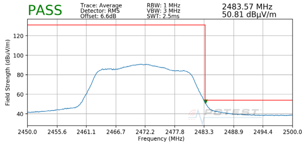
Plot 7-133. Radiated Restricted Upper Band Edge Measurement MIMO (Average)
