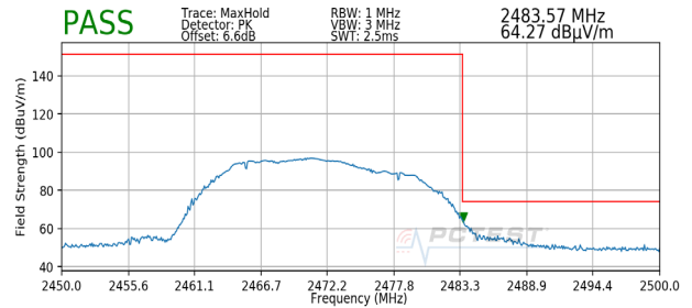
Plot 7-124. Radiated Restricted Upper Band Edge Measurement SISO ANT2 (Peak)
