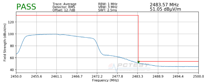
Plot 7-109. Radiated Restricted Upper Band Edge Measurement SISO ANT1 (Average)
