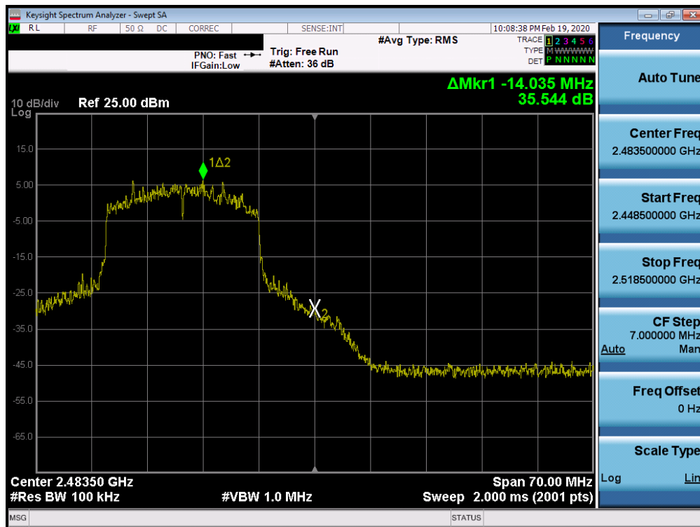
Plot 7-61. Band Edge Plot SISO ANT1 (802.11ax (2.4GHz) – Ch. 12)
