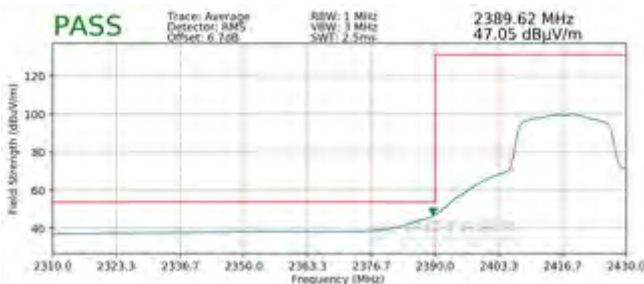
Plot 7-101. Radiated Restricted Lower Band Edge Measurement MIMO (Average)
