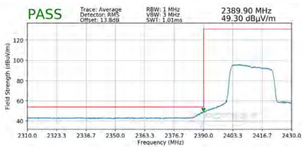
Plot 7-91. Radiated Restricted Lower Band Edge Measurement SISO ANT2 (Average)
