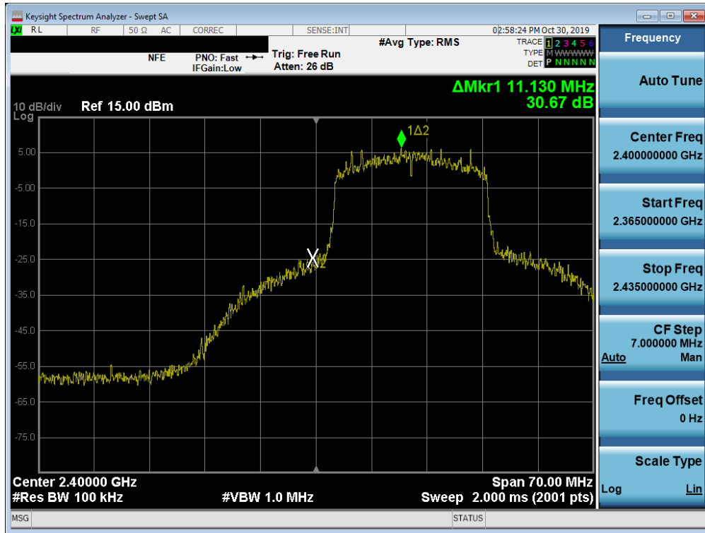
Plot 7-57. Band Edge Plot SISO ANT2 (802.11ax (2.4GHz) – Ch. 1)
