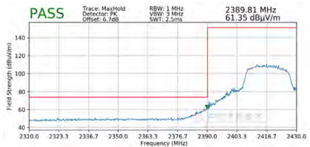
Plot 7-86. Radiated Restricted Lower Band Edge Measurement SISO ANT1 (Peak)
