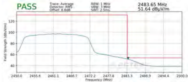
Plot 7-105. Radiated Restricted Upper Band Edge Measurement MIMO (Average)
