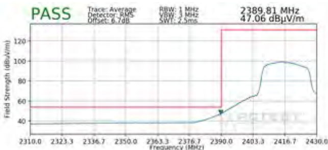
Plot 7-85. Radiated Restricted Lower Band Edge Measurement SISO ANT1 (Average)
