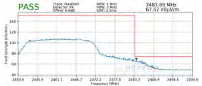
Plot 7-106. Radiated Restricted Upper Band Edge Measurement MIMO (Peak)
