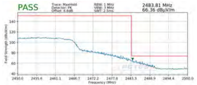
Plot 7-104. Radiated Restricted Upper Band Edge Measurement MIMO (Peak)
