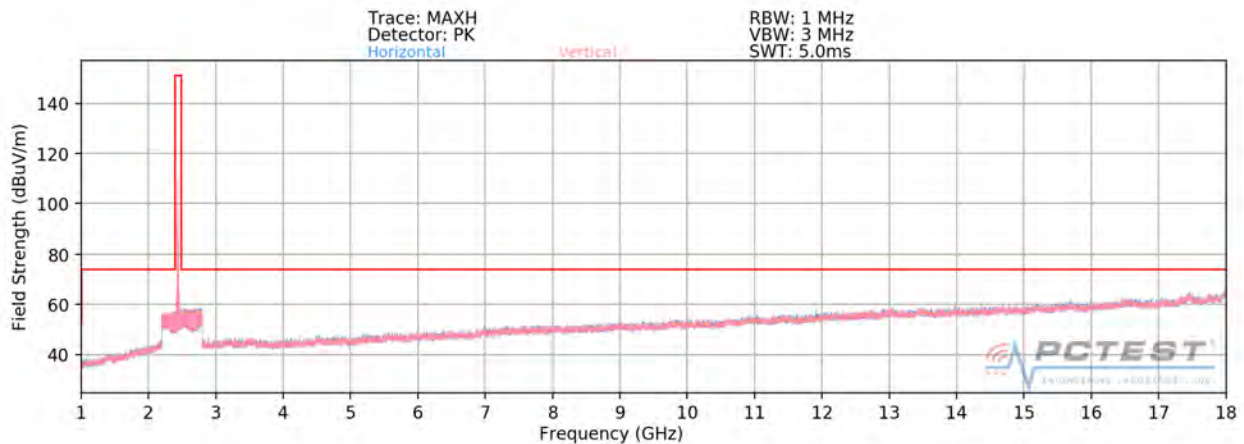
Plot 7-72. Radiated Spurious Plot above 1GHz SISO ANT1 (802.11b – Ch. 6)
