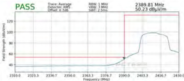
Plot 7-99. Radiated Restricted Lower Band Edge Measurement MIMO (Average)
