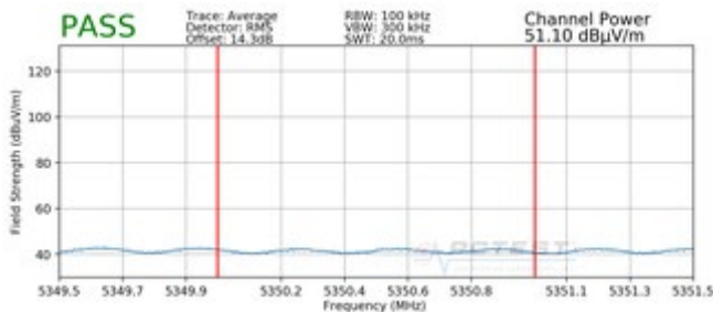
Plot 7-354. Radiated Upper Band Edge Plot MIMO (Average – UNII Band 2A)
