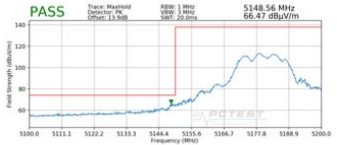
Plot 7-335. Radiated Lower Band Edge Plot MIMO (Peak – UNII Band 1)
