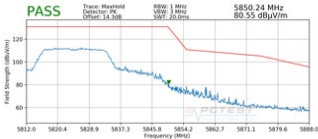
Plot 7-340. Radiated Upper Band Edge Plot MIMO (Peak – UNII Band 3)
