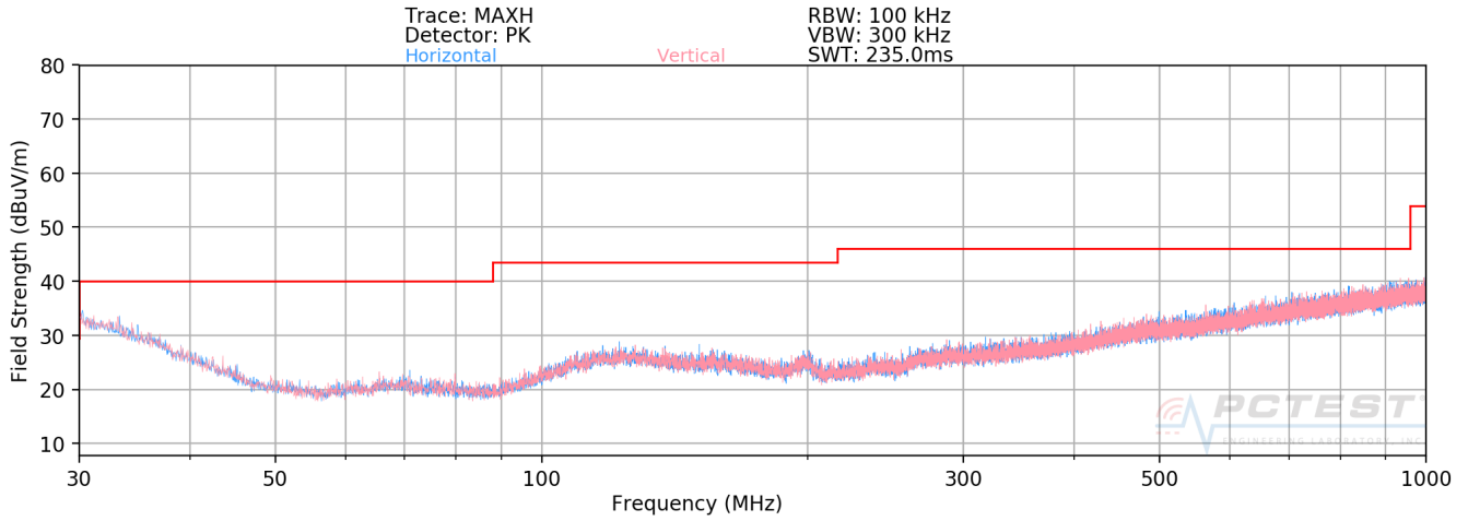
Plot 7-361. Radiated Spurious Plot below 1GHz SISO ANT1 (802.11a – U3 Ch. 157)
