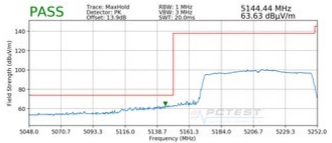
Plot 7-328. Radiated Lower Band Edge Plot SISO ANT2 (Peak – UNII Band 1)
