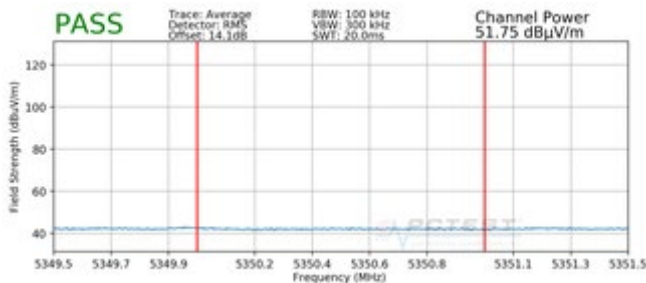
Plot 7-308. Radiated Upper Band Edge Plot SISO ANT1 (Average – UNII Band 2A)
