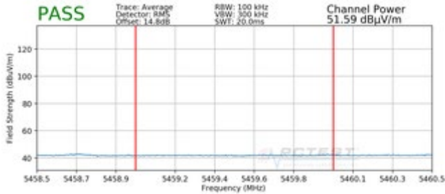
Plot 7-331. Radiated Lower Band Edge Plot SISO ANT2 (Average – UNII Band 2C)
