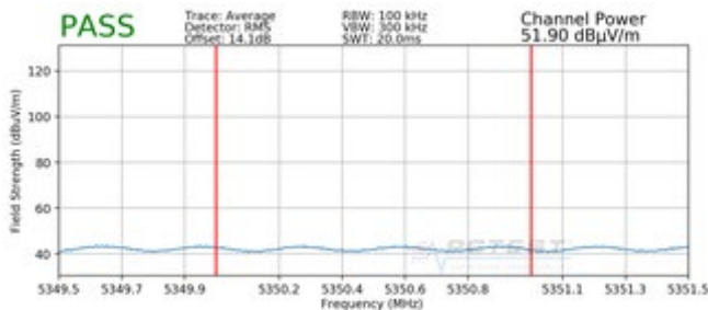
Plot 7-329. Radiated Upper Band Edge Plot SISO ANT2 (Average – UNII Band 2A)
