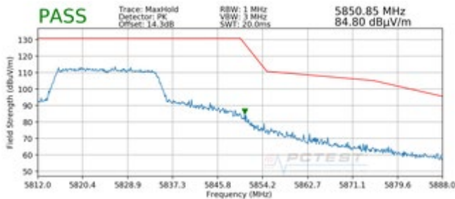
Plot 7-319. Radiated Upper Band Edge Plot SISO ANT2 (Peak – UNII Band 3)
