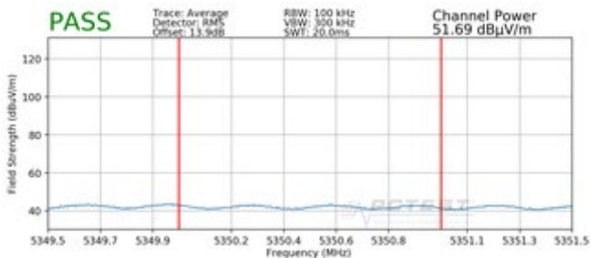
Plot 7-322. Radiated Upper Band Edge Plot SISO ANT2 (Average – UNII Band 2A)
