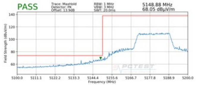
Plot 7-314. Radiated Lower Band Edge Plot SISO ANT2 (Peak – UNII Band 1)
