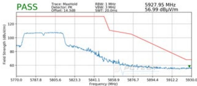
Plot 7-349. Radiated Upper Band Edge Plot MIMO (Peak – UNII Band 3)
