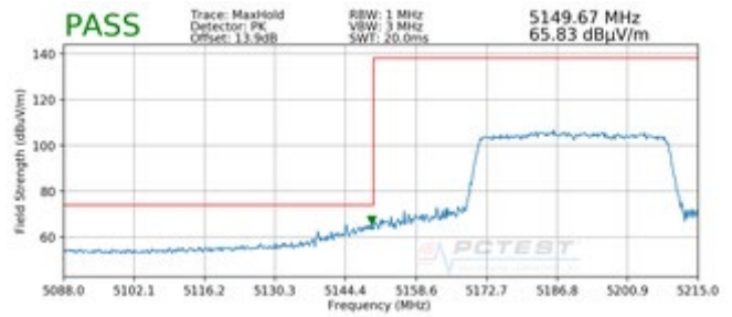
Plot 7-344. Radiated Lower Band Edge Plot MIMO (Peak – UNII Band 1)
