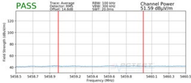
Plot 7-347. Radiated Lower Band Edge Plot MIMO (Average – UNII Band 2C)
