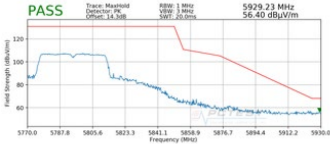
Plot 7-326. Radiated Upper Band Edge Plot SISO ANT2 (Peak – UNII Band 3)
