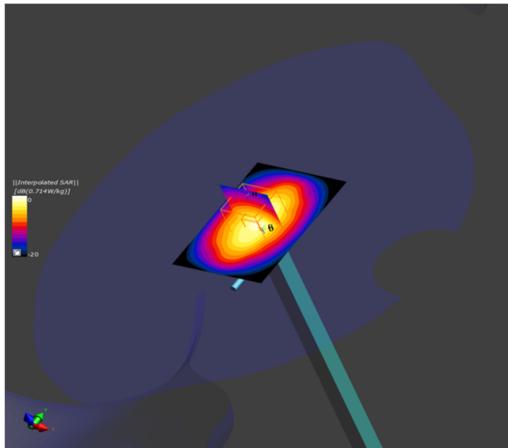
Figure C-4 SAR measurement system verification plot for 1800MHz performed on 12/5/2019. Input power = 10.0mW.
