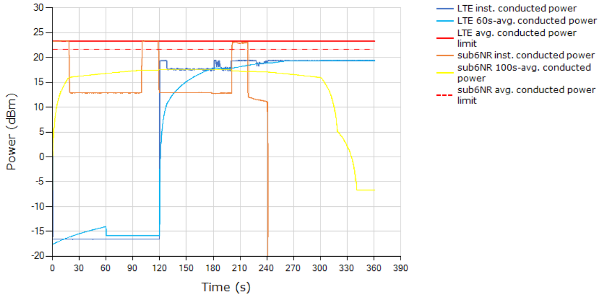
LTE and sub6NR Instantaneous and Time-averaged TX Power Tech: LTE, Band 48 / Tech: NR5G SUB6, Band n66
