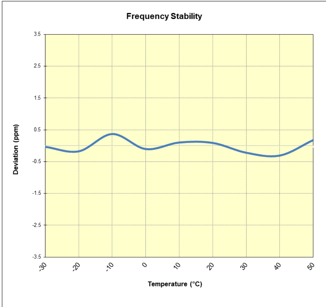
Figure 7-6. CDMA BC10 Frequency Stability Chart
