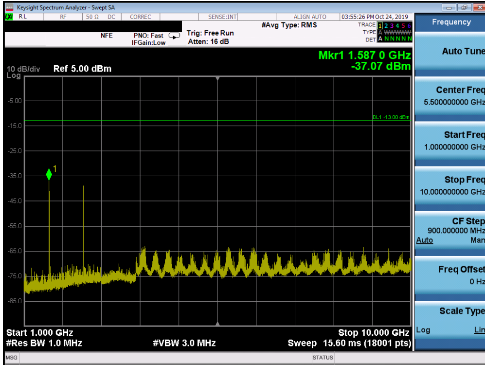
Plot 7-48. Conducted Spurious Plot (LTE Band 14, 5.0 MHz QPSK – RB Size 1, RB Offset 0 – High Channel)
