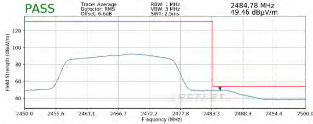
Plot 7-125. Radiated Restricted Upper Band Edge Measurement MIMO (Average – 242 Tones)
