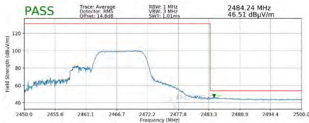
Plot 7-83. Radiated Restricted Upper Band Edge Measurement SISO ANT1 (Average – 106 Tones)
