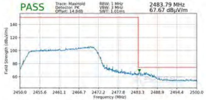
Plot 7-110. Radiated Restricted Upper Band Edge Measurement SISO ANT2 (Peak – 242 Tones)
