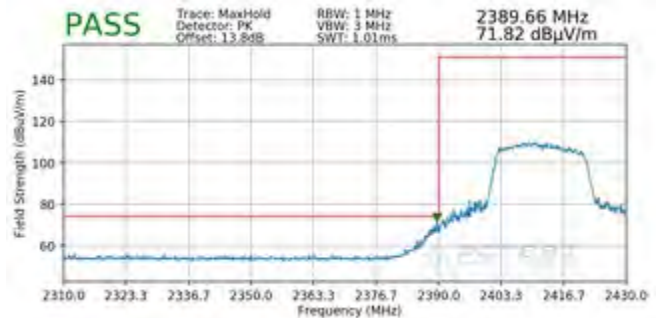
Plot 7-90. Radiated Restricted Lower Band Edge Measurement SISO ANT1 (Peak – 242 Tones)
