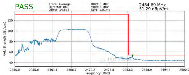
Plot 7-115. Radiated Restricted Upper Band Edge Measurement MIMO (Average – 106 Tones)
