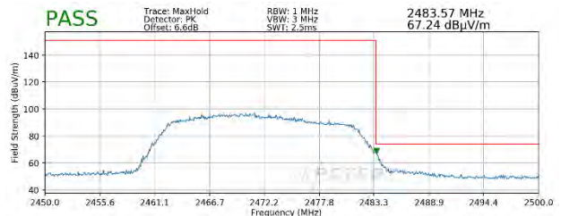
Plot 7-128. Radiated Restricted Upper Band Edge Measurement MIMO (Peak – 242 Tones)
