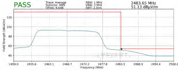
Plot 7-93. Radiated Restricted Upper Band Edge Measurement SISO ANT1 (Average – 242 Tones)
