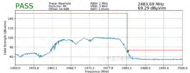
Plot 7-120. Radiated Restricted Upper Band Edge Measurement MIMO (Peak – 106 Tones)
