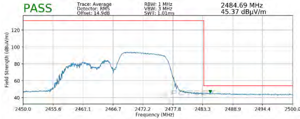
Plot 7-117. Radiated Restricted Upper Band Edge Measurement MIMO (Average – 106 Tones)
