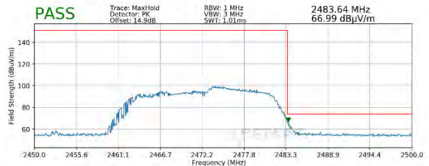
Plot 7-104. Radiated Restricted Upper Band Edge Measurement SISO ANT2 (Peak – 106 Tones)
