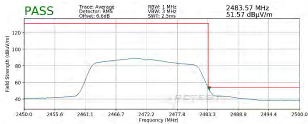
Plot 7-111. Radiated Restricted Upper Band Edge Measurement SISO ANT2 (Average – 242 Tones)
