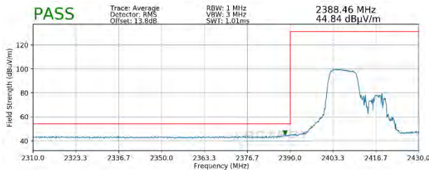
Plot 7-97. Radiated Restricted Lower Band Edge Measurement SISO ANT2 (Average – 106 Tones)
