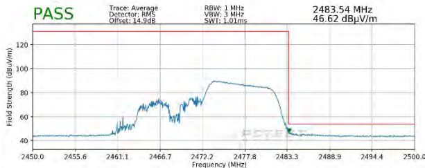
Plot 7-103. Radiated Restricted Upper Band Edge Measurement SISO ANT2 (Average – 106 Tones)
