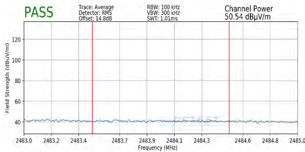
Plot 7-91. Radiated Restricted Upper Band Edge Measurement SISO ANT1 (Average – 242 Tones)
