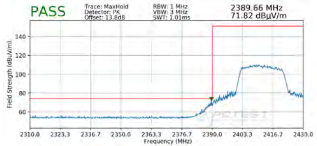
Plot 7-100. Radiated Restricted Lower Band Edge Measurement SISO ANT1 (Peak)
