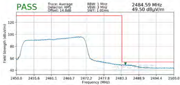
Plot 7-117. Radiated Restricted Upper Band Edge Measurement SISO ANT2 (Average)
