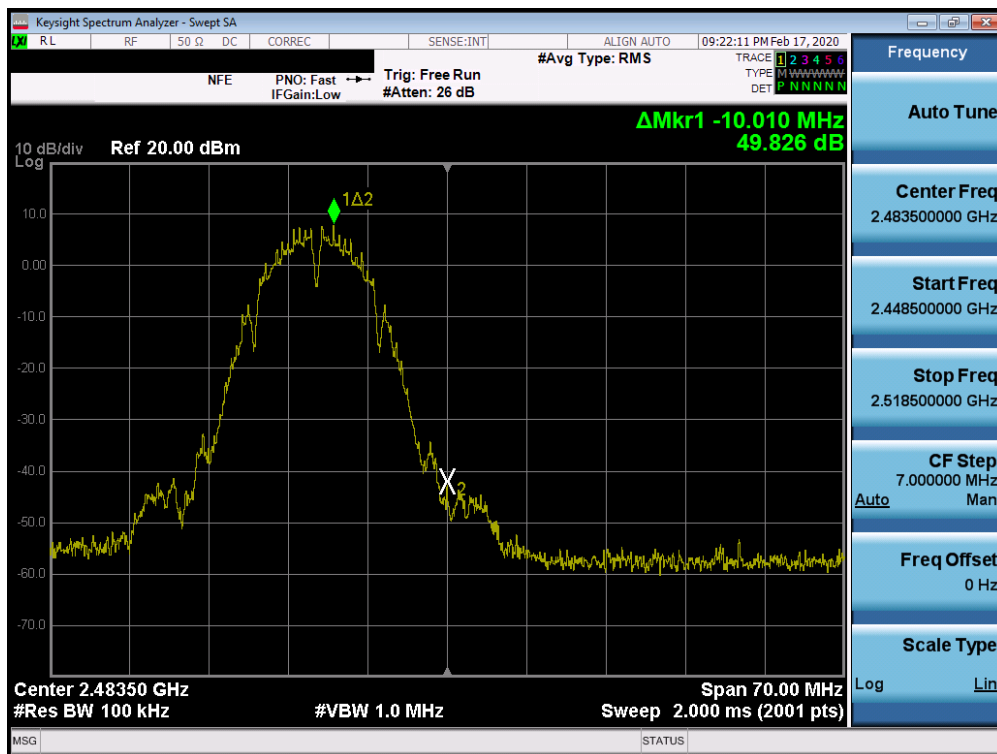
Plot 7-62. Band Edge Plot SISO ANT2 (802.11b – Ch. 13)
