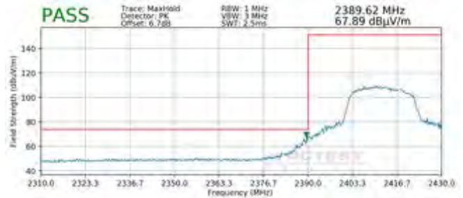
Plot 7-124. Radiated Restricted Lower Band Edge Measurement MIMO (Peak)
