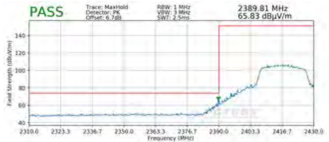
Plot 7-114. Radiated Restricted Lower Band Edge Measurement SISO ANT2 (Peak)
