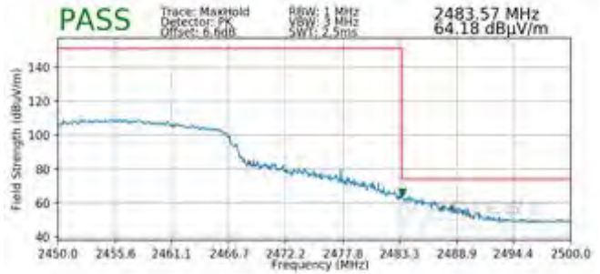
Plot 7-104. Radiated Restricted Upper Band Edge Measurement SISO ANT1 (Peak)
