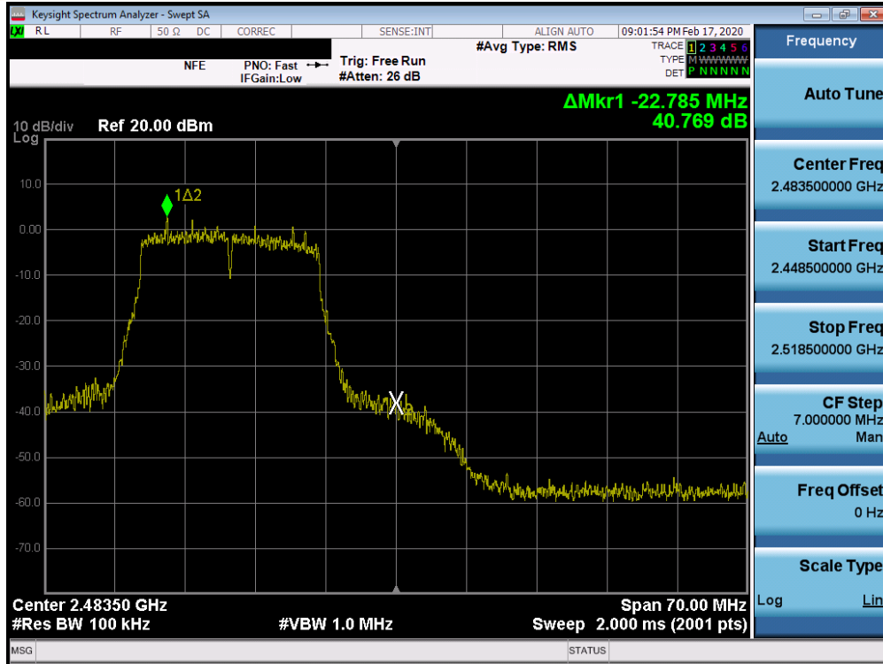
Plot 7-53. Band Edge Plot SISO ANT1 (802.11n – Ch. 12)
