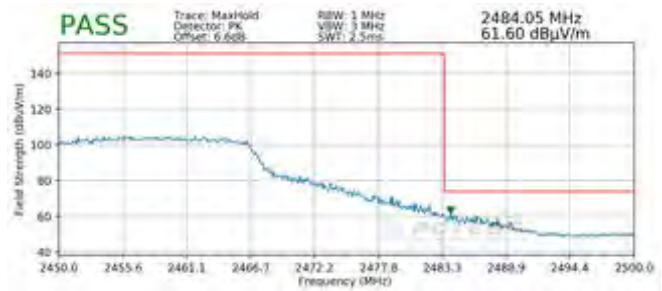
Plot 7-116. Radiated Restricted Upper Band Edge Measurement SISO ANT2 (Peak)
