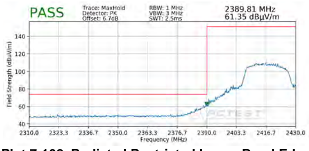
Plot 7-102. Radiated Restricted Lower Band Edge Measurement SISO ANT1 (Peak)
