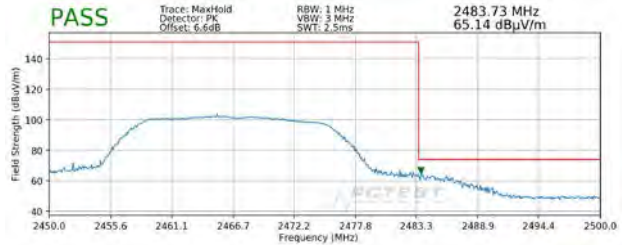
Plot 7-108. Radiated Restricted Upper Band Edge Measurement SISO ANT1 (Peak)
