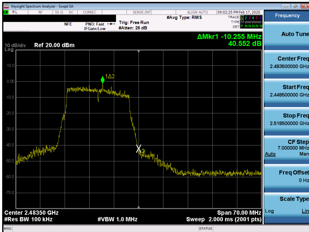
Plot 7-54. Band Edge Plot SISO ANT1 (802.11n – Ch. 13)
