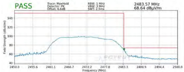
Plot 7-110. Radiated Restricted Upper Band Edge Measurement SISO ANT1 (Peak)
