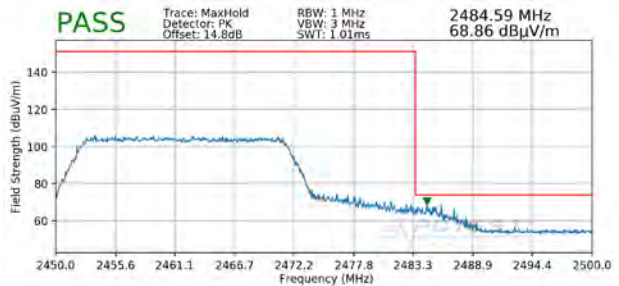
Plot 7-106. Radiated Restricted Upper Band Edge Measurement SISO ANT1 (Peak)
