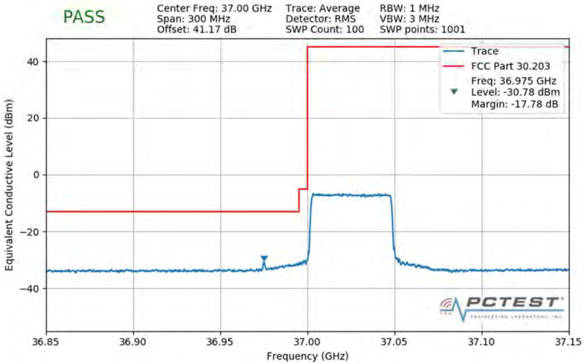
Plot 7-465. Lower Band Edge Plot (1CC 50MHz QPSK Full RB)
