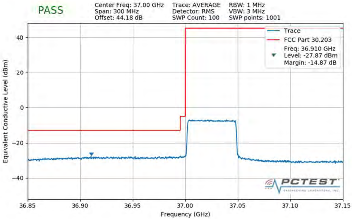
Plot 7-369. Lower Band Edge Plot (1CC 50MHz QPSK Full RB)
