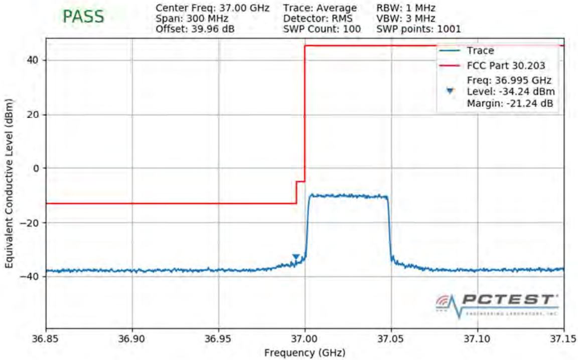
Plot 7-497. Lower Band Edge Plot (1CC 50MHz QPSK Full RB)
