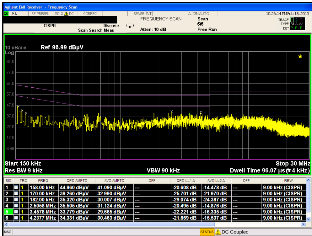
Plot 7-56. Line Conducted Plot with Bluetooth LE (N) with Travel Adapter
