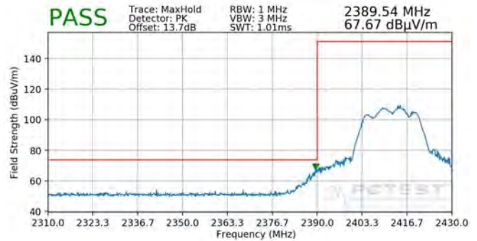
Plot 7-102. Radiated Restricted Lower Band Edge Measurement CDD (Peak)
