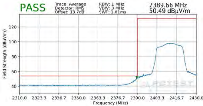
Plot 7-107. Radiated Restricted Lower Band Edge Measurement MIMO (Average)
