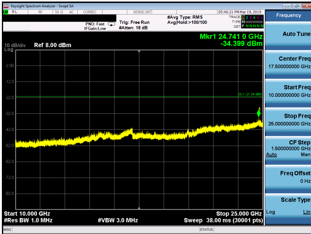
Plot 7-42. Conducted Spurious Plot SISO ANT2 (802.11ax OFDMA– 26 Tones – Ch. 6)
