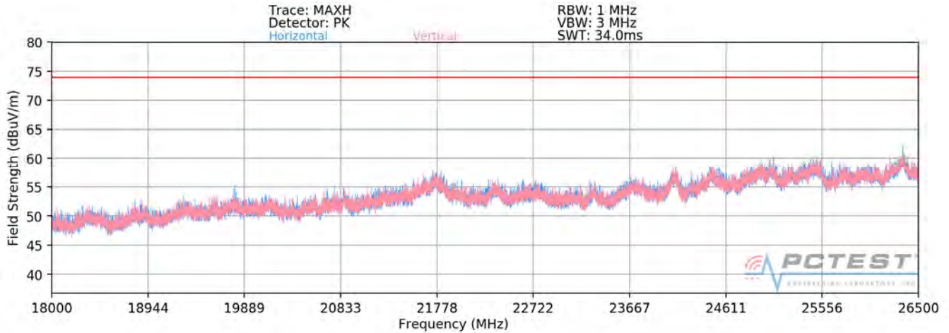
Plot 7-57. Radiated Spurious Plot above 18GHz SISO ANT1 (802.11ax OFDMA – 106 Tones)
