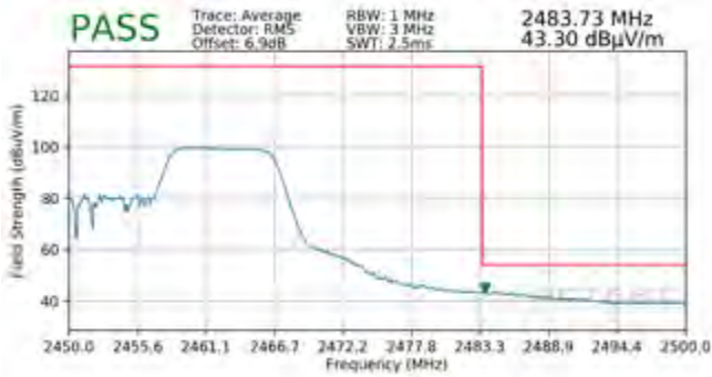
Plot 7-79. Radiated Restricted Upper Band Edge Measurement SISO ANT1 (Average – 106 Tones)
