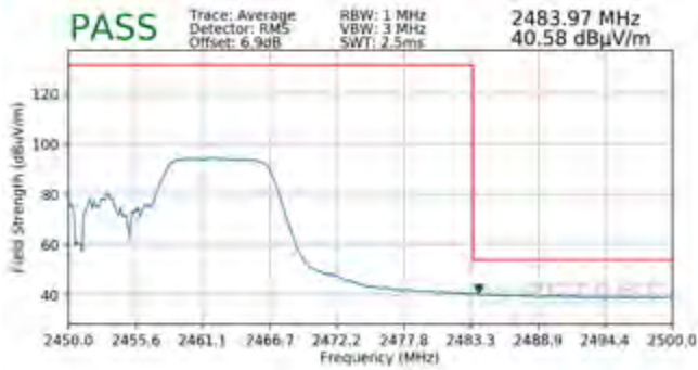
Plot 7-115. Radiated Restricted Upper Band Edge Measurement MIMO (Average – 106 Tones)
