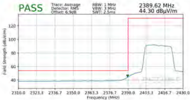
Plot 7-119. Radiated Restricted Lower Band Edge Measurement MIMO (Average – 242 Tones)
