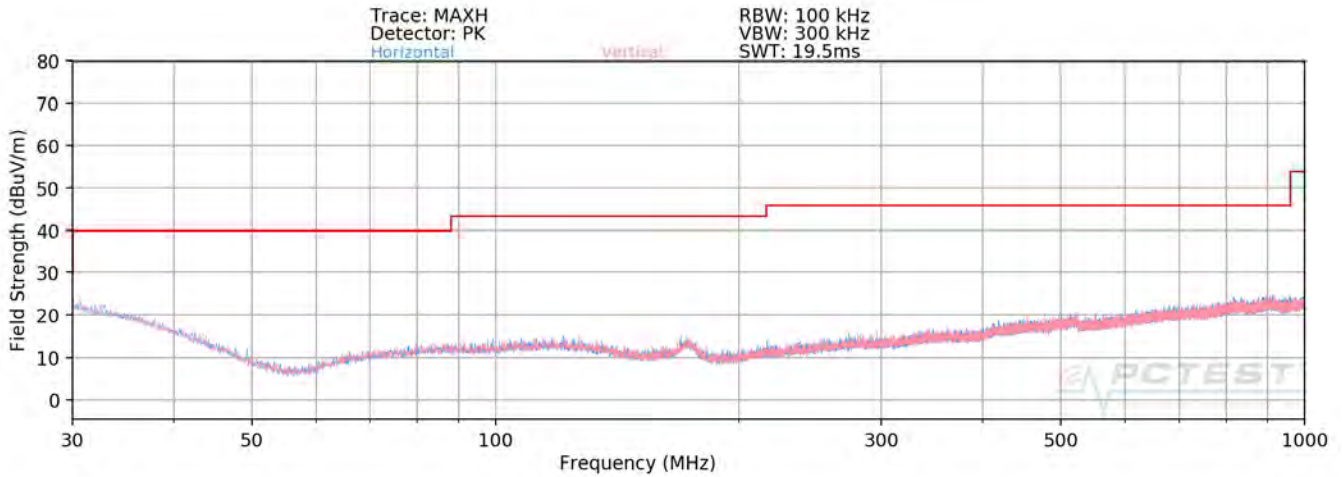
Plot 7-130. Radiated Spurious Plot below 1GHz SISO ANT1 (242 Tones)
