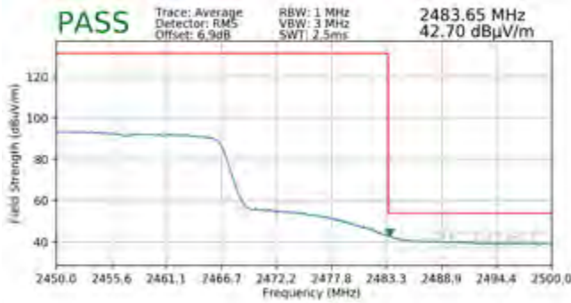
Plot 7-123. Radiated Restricted Upper Band Edge Measurement MIMO (Average – 242 Tones)
