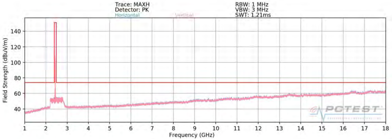
Plot 7-68. Radiated Spurious Plot above 1GHz MIMO (802.11ax OFDMA – 106 Tones – Ch. 6)
