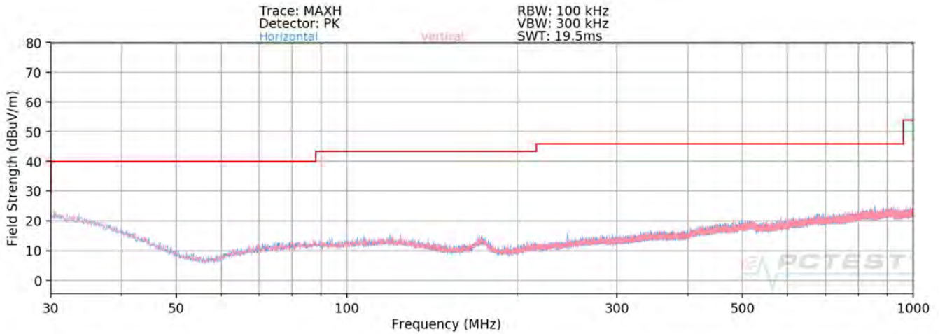
Plot 7-132. Radiated Spurious Plot below 1GHz SISO ANT2 (242 Tones)
