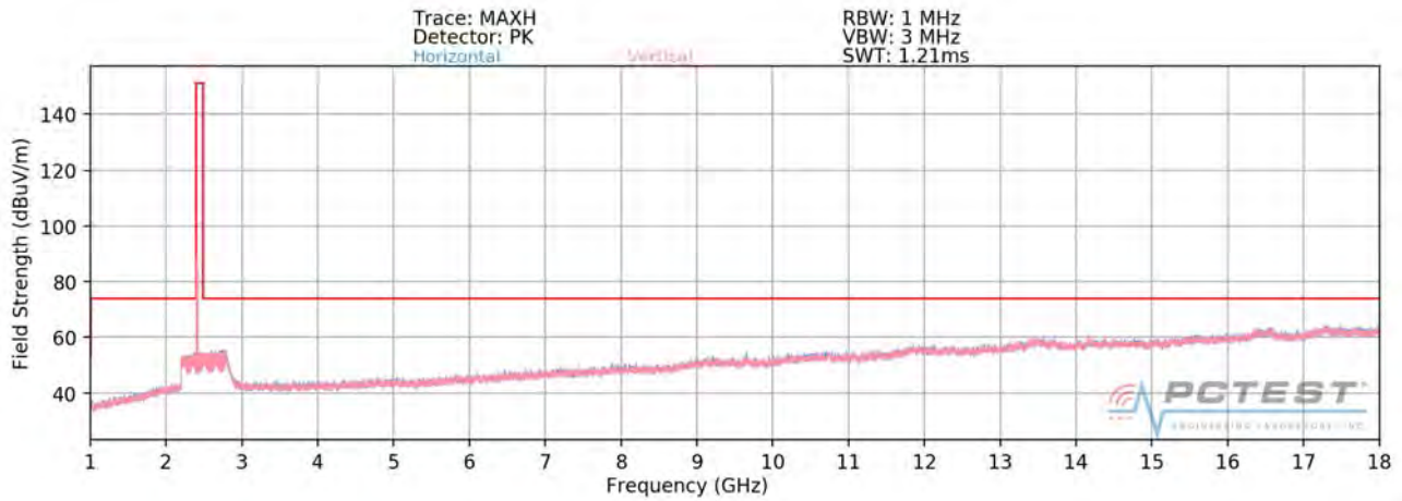
Plot 7-59. Radiated Spurious Plot above 1GHz SISO ANT2 (802.11ax OFDMA – 106 Tones – Ch. 1)
