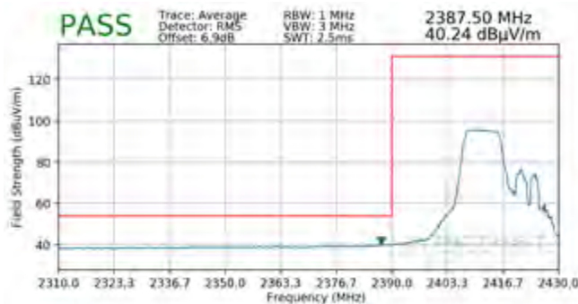
Plot 7-95. Radiated Restricted Lower Band Edge Measurement SISO ANT2 (Average – 106 Tones)
