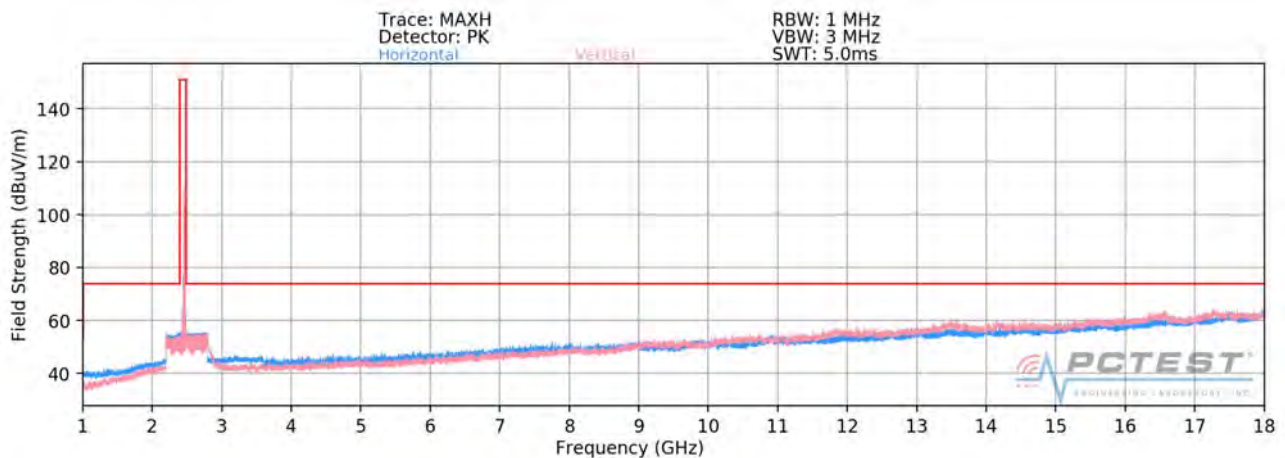
Plot 7-53. Radiated Spurious Plot above 1GHz SISO ANT1 (802.11ax OFDMA – 106 Tones – Ch. 11)
