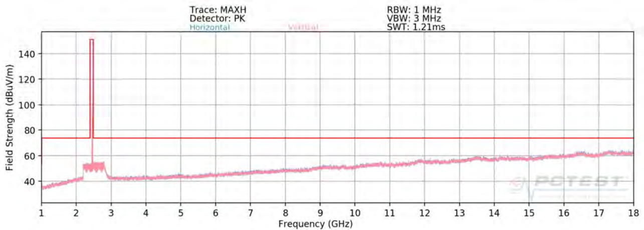
Plot 7-61. Radiated Spurious Plot above 1GHz SISO ANT2 (802.11ax OFDMA – 106 Tones – Ch. 11)
