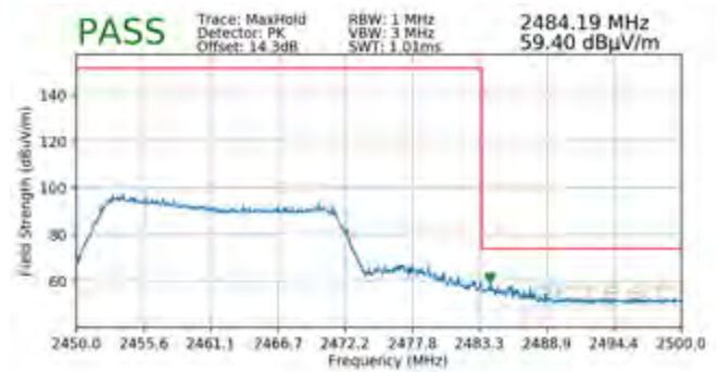
Plot 7-110. Radiated Restricted Band Edge Measurement SISO ANT2 with WCP (Peak – 242 Tones)
