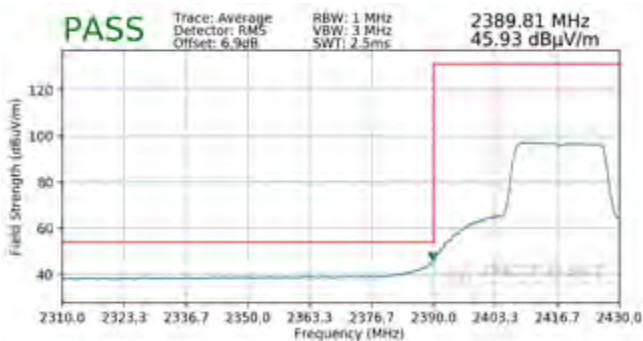
Plot 7-85. Radiated Restricted Lower Band Edge Measurement SISO ANT1 (Average – 242 Tones)
