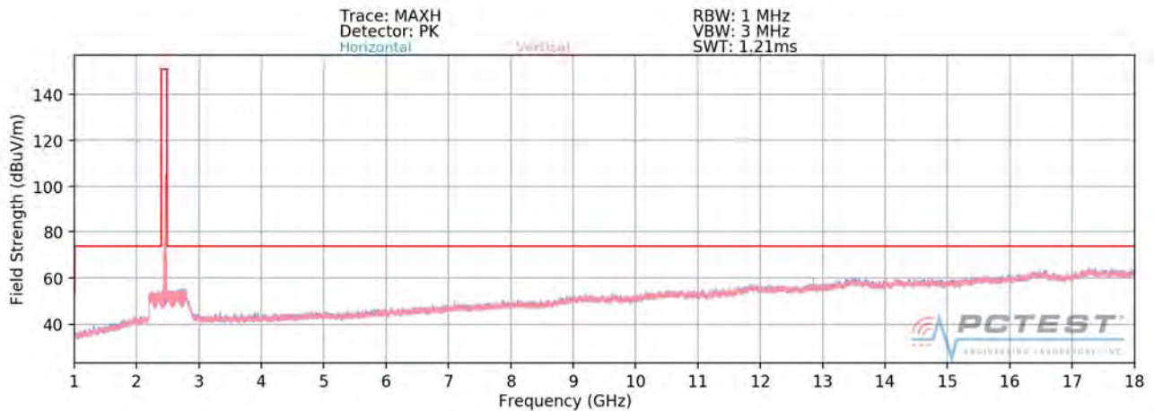
Plot 7-56. Radiated Spurious Plot above 1GHz SISO ANT1 (802.11ax OFDMA – 242 Tones – Ch. 11)
