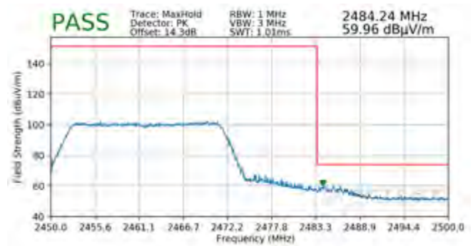
Plot 7-128. Radiated Restricted Band Edge Measurement MIMO with WCP (Peak – 242 Tones)
