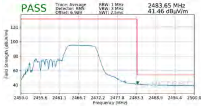
Plot 7-99. Radiated Restricted Upper Band Edge Measurement SISO ANT2 (Average – 106 Tones)
