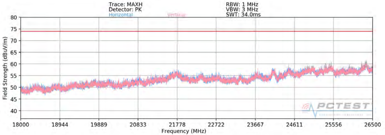
Plot 7-65. Radiated Spurious Plot above 18GHz SISO ANT2 (802.11ax OFDMA – 106 Tones)
