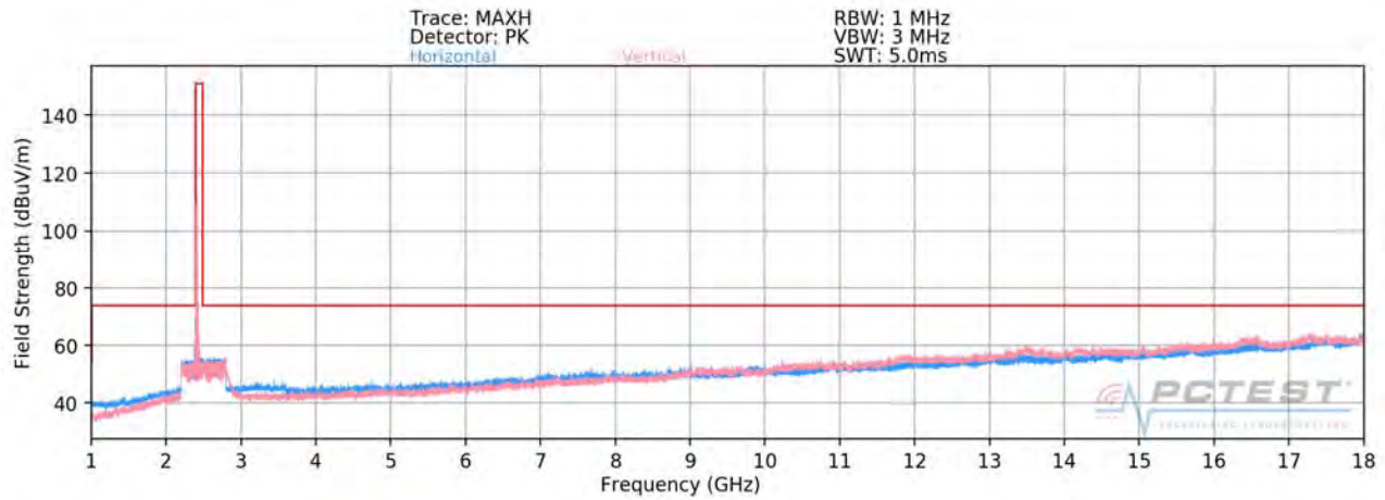
Plot 7-51. Radiated Spurious Plot above 1GHz SISO ANT1 (802.11ax OFDMA – 106 Tones – Ch. 1)
