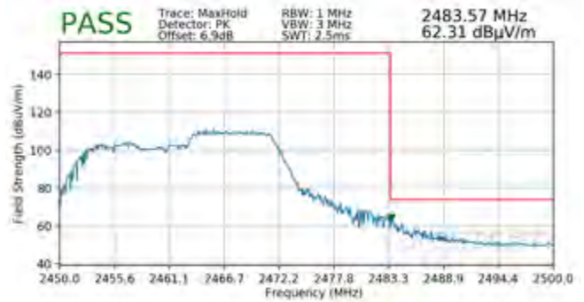
Plot 7-82. Radiated Restricted Upper Band Edge Measurement SISO ANT1 (Peak – 106 Tones)
