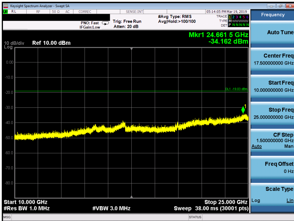
Plot 7-28. Conducted Spurious Plot SISO ANT1 (802.11ax OFDMA– 26 Tones – Ch. 1)
