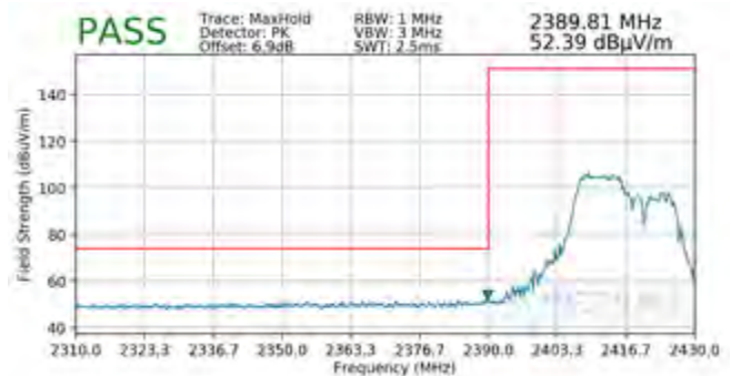
Plot 7-96. Radiated Restricted Lower Band Edge Measurement SISO ANT2 (Peak – 106 Tones)
