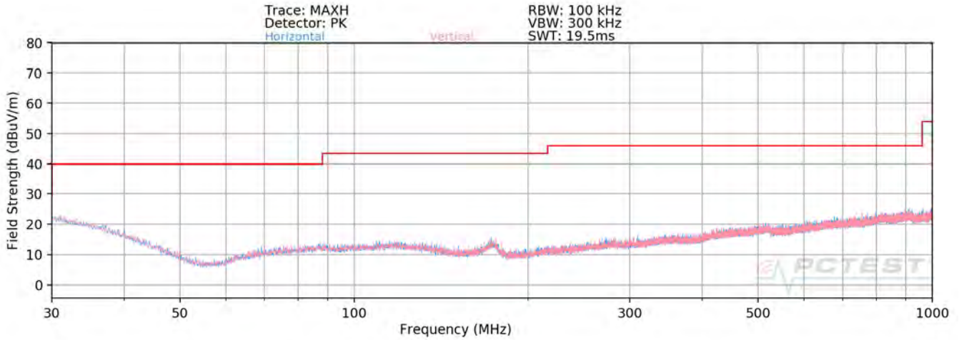
Plot 7-129. Radiated Spurious Plot below 1GHz SISO ANT1 (106 Tones)
