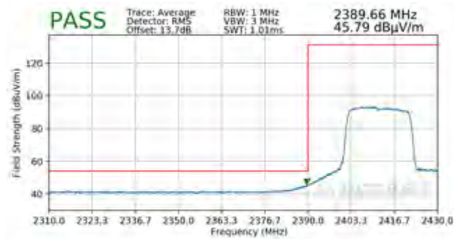
Plot 7-91. Radiated Restricted Band Edge Measurement SISO ANT1 with WCP (Average – 242 Tones)
