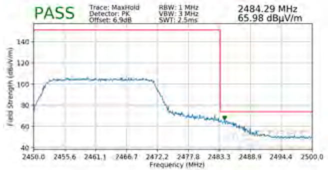
Plot 7-90. Radiated Restricted Upper Band Edge Measurement SISO ANT1 (Peak – 242 Tones)
