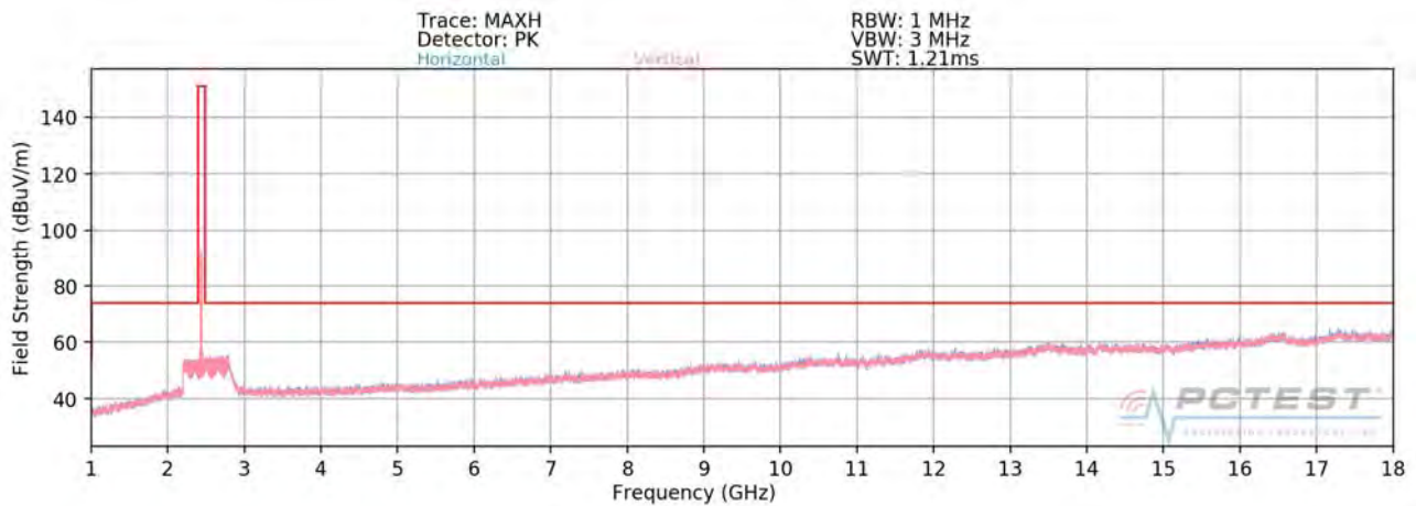
Plot 7-60. Radiated Spurious Plot above 1GHz SISO ANT2 (802.11ax OFDMA – 106 Tones – Ch. 6)
