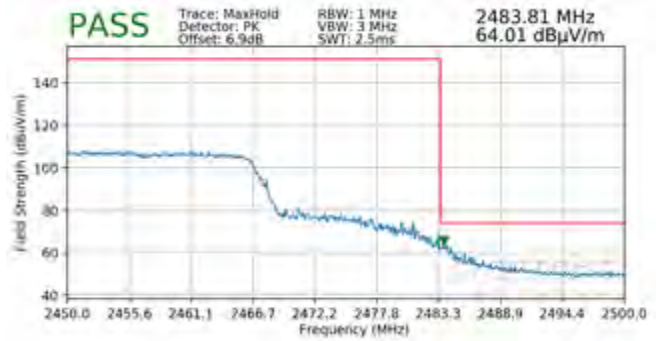
Plot 7-88. Radiated Restricted Upper Band Edge Measurement SISO ANT1 (Peak – 242 Tones)
