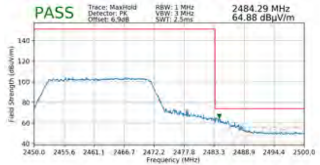
Plot 7-126. Radiated Restricted Upper Band Edge Measurement MIMO (Peak – 242 Tones)
