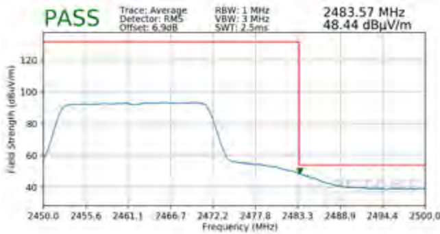
Plot 7-125. Radiated Restricted Upper Band Edge Measurement MIMO (Average – 242 Tones)
