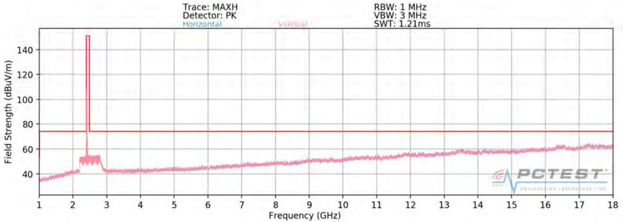
Plot 7-67. Radiated Spurious Plot above 1GHz MIMO (802.11ax OFDMA – 106 Tones – Ch. 1)
