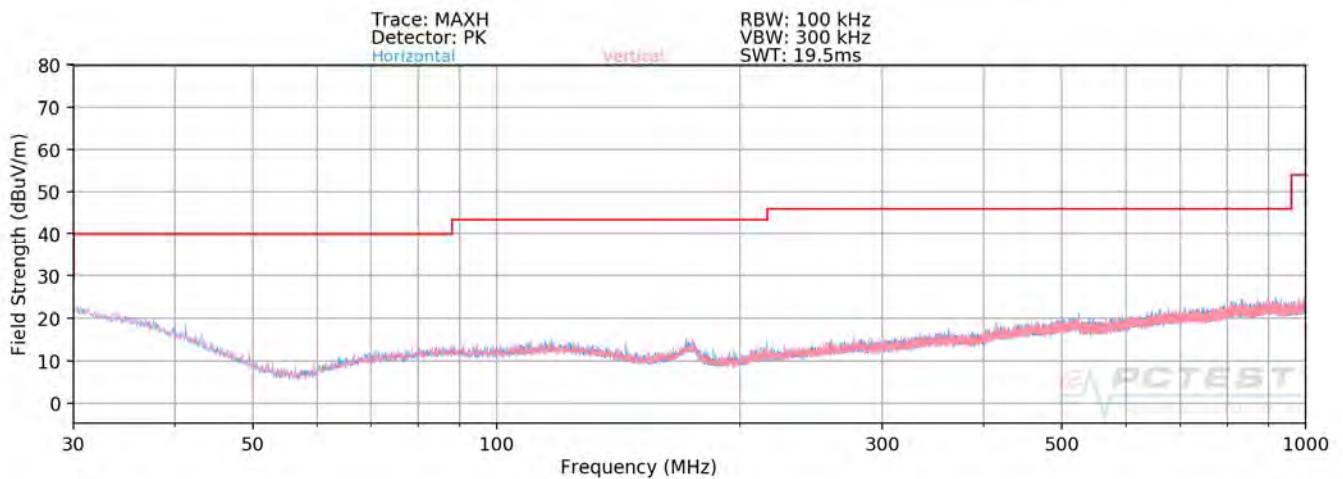
Plot 7-134. Radiated Spurious Plot below 1GHz MIMO (242 Tones)
