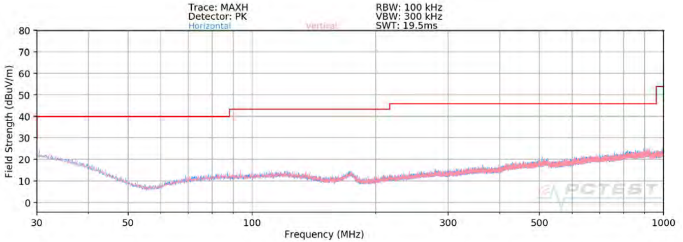
Plot 7-131. Radiated Spurious Plot below 1GHz SISO ANT2 (106 Tones)
