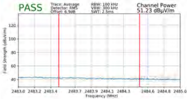
Plot 7-107. Radiated Restricted Upper Band Edge Measurement SISO ANT2 (Average – 242 Tones)
