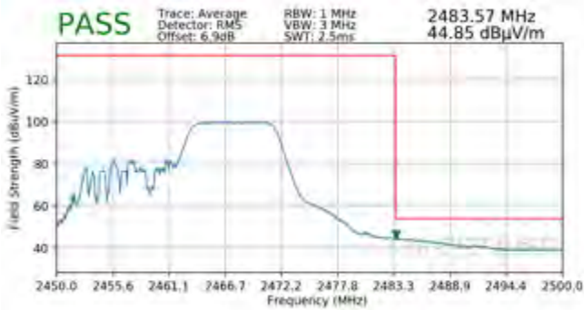
Plot 7-81. Radiated Restricted Upper Band Edge Measurement SISO ANT1 (Average – 106 Tones)
