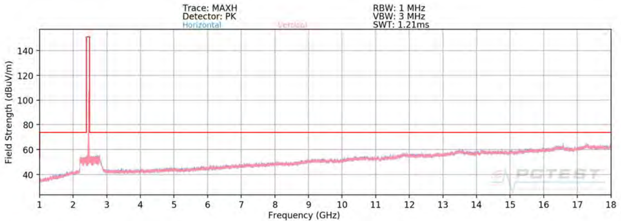
Plot 7-69. Radiated Spurious Plot above 1GHz MIMO (802.11ax OFDMA – 106 Tones – Ch. 11)
