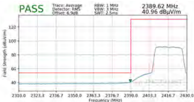
Plot 7-121. Radiated Restricted Lower Band Edge Measurement MIMO (Average – 242 Tones)
