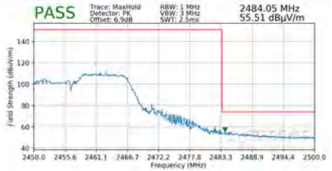
Plot 7-80. Radiated Restricted Upper Band Edge Measurement SISO ANT1 (Peak – 106 Tones)
