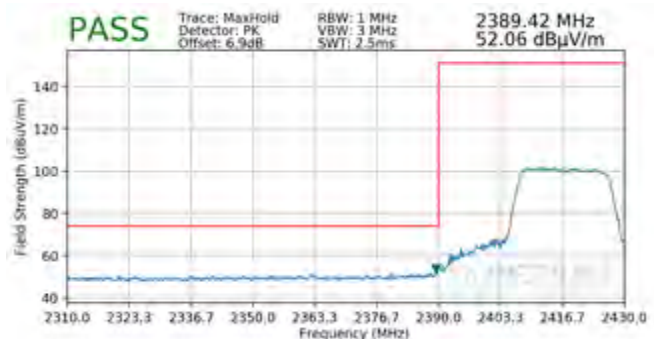
Plot 7-122. Radiated Restricted Lower Band Edge Measurement MIMO (Peak – 242 Tones)
