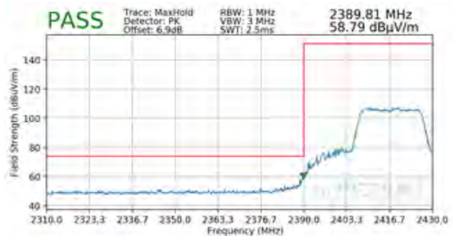
Plot 7-86. Radiated Restricted Lower Band Edge Measurement SISO ANT1 (Peak – 242 Tones)
