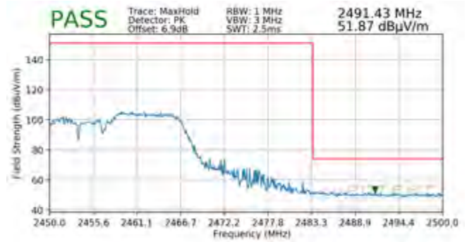
Plot 7-98. Radiated Restricted Upper Band Edge Measurement SISO ANT2 (Peak – 106 Tones)
