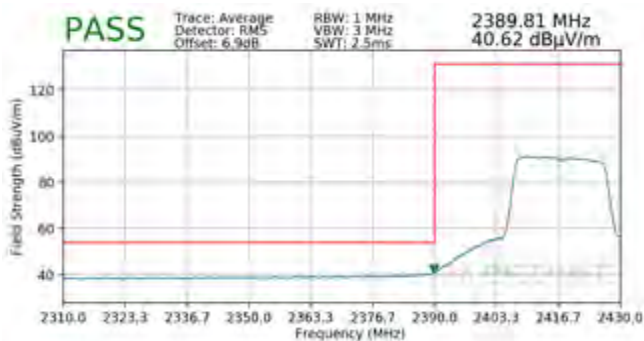
Plot 7-103. Radiated Restricted Lower Band Edge Measurement SISO ANT2 (Average – 242 Tones)
