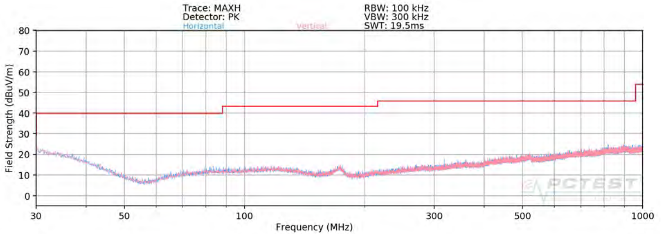
Plot 7-133. Radiated Spurious Plot below 1GHz MIMO (106 Tones)
