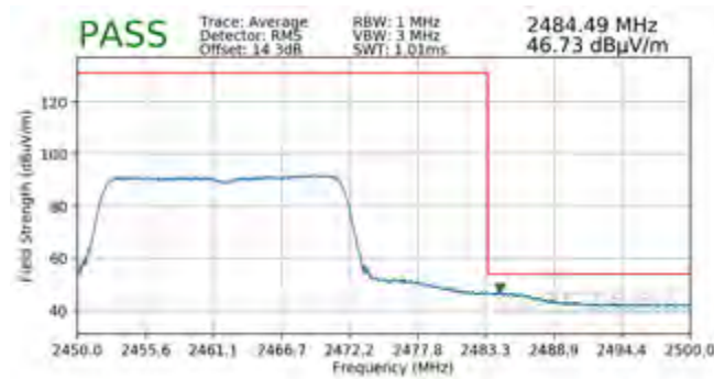
Plot 7-127. Radiated Restricted Band Edge Measurement MIMO with WCP (Average – 242 Tones)
