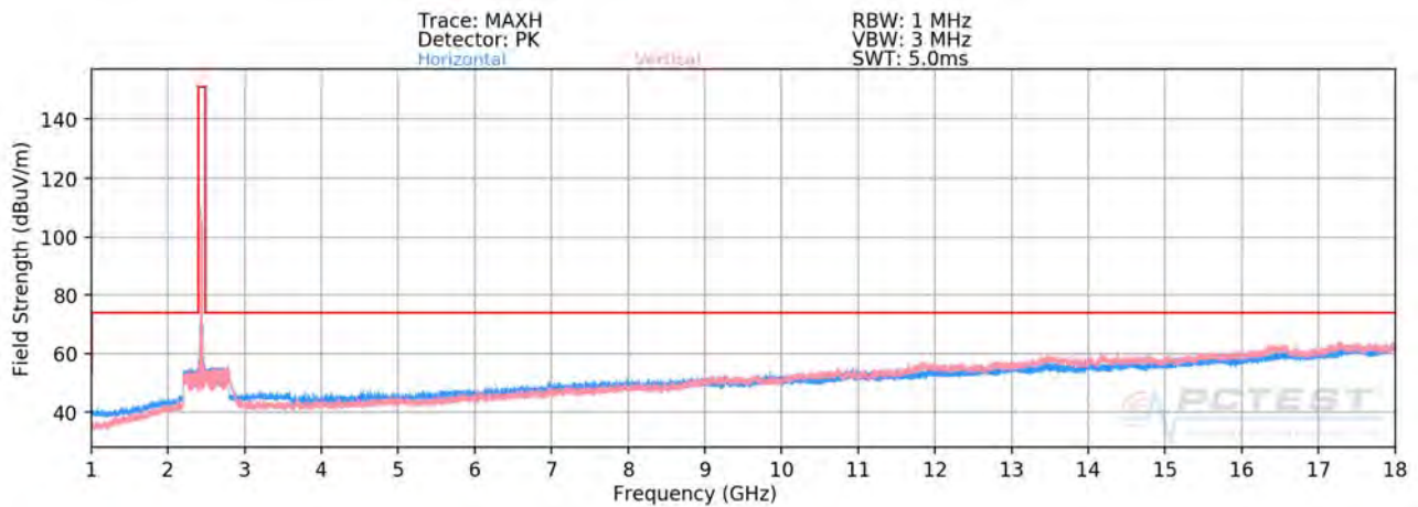
Plot 7-52. Radiated Spurious Plot above 1GHz SISO ANT1 (802.11ax OFDMA – 106 Tones – Ch. 6)
