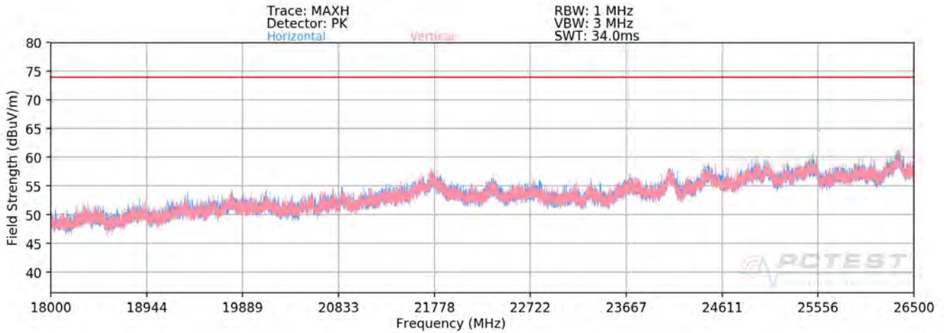
Plot 7-73. Radiated Spurious Plot above 18GHz MIMO (802.11ax OFDMA – 106 Tones)
