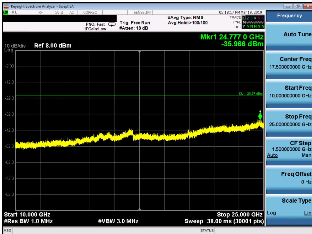
Plot 7-32. Conducted Spurious Plot SISO ANT1 (802.11ax OFDMA– 26 Tones – Ch. 11)
