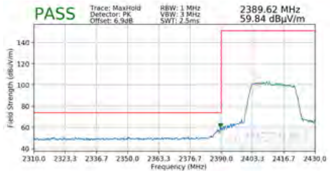
Plot 7-120. Radiated Restricted Lower Band Edge Measurement MIMO (Peak – 242 Tones)
