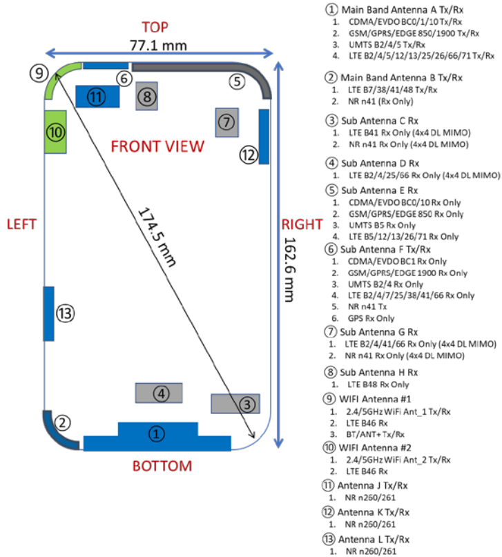
Figure E-1 DUT Antenna Locations
