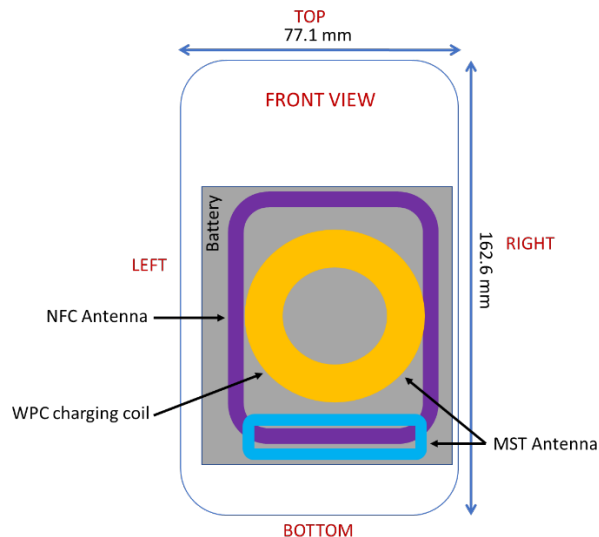
Figure E-2 NFC/MST Antenna and WPC Locations
