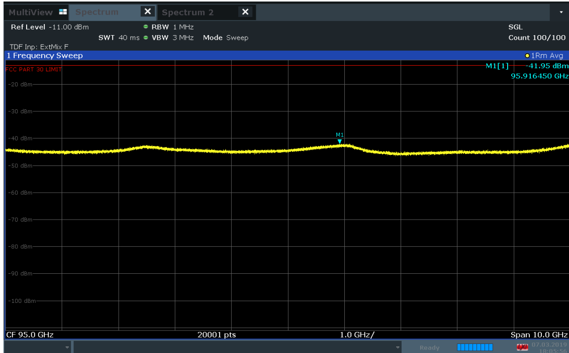
Plot 7-147. K Patch Radiated Spurious Plot 90-100 GHz (1CC QPSK High Channel H Beam)
