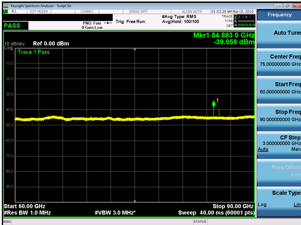
Plot 7-144. K Patch Radiated Spurious Plot 60-90 GHz (1CC QPSK High Channel V Beam)
