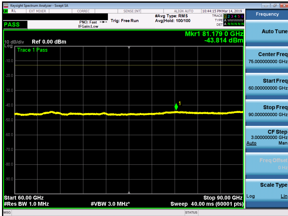
Plot 7-106. J Patch Radiated Spurious Plot 60-90 GHz (1CC 16QAM Mid Channel H Beam)
