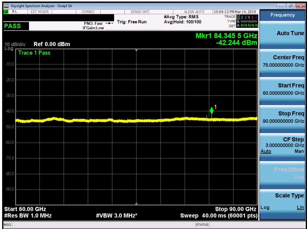
Plot 7-75. J Dipole Radiated Spurious Plot 60-90 GHz (1CC 16QAM Mid Channel V Beam)
