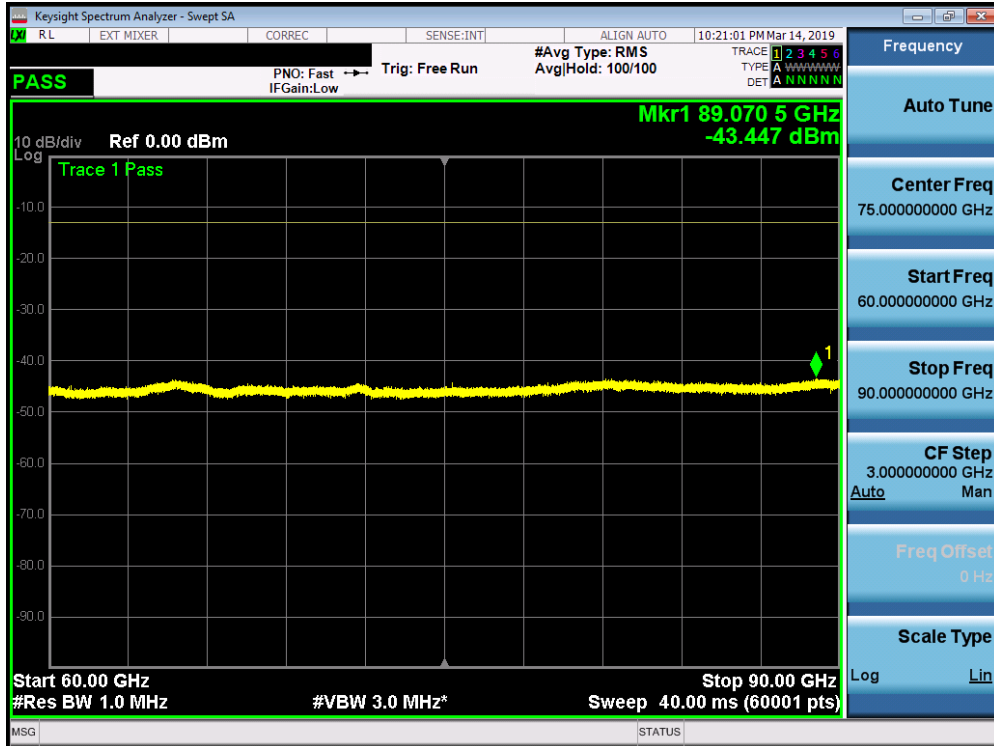
Plot 7-109. J Patch Radiated Spurious Plot 60-90 GHz (1CC 16QAM Mid Channel V Beam)
