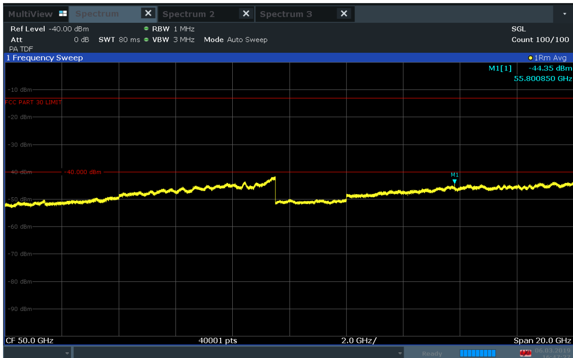
Plot 7-66. J Dipole Radiated Spurious Plot 40-60 GHz (1CC 16QAM Mid Channel H Beam)
