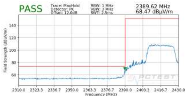
Plot 7-82. Radiated Restricted Lower Band Edge Measurement SISO ANT1 (Peak – 242 Tones)
