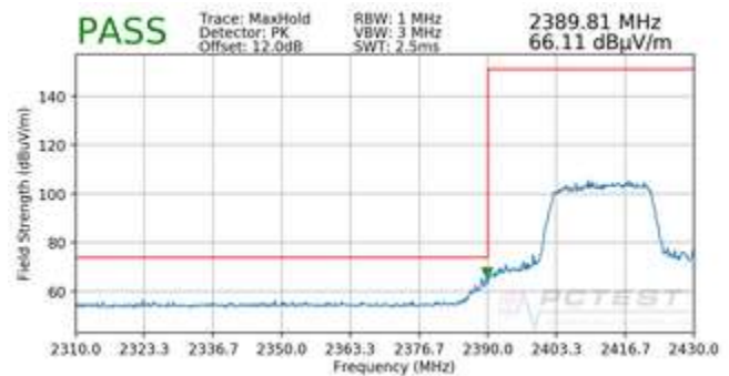
Plot 7-88. Radiated Restricted Band Edge Measurement SISO ANT1 with WCP (Peak – 242 Tones)
