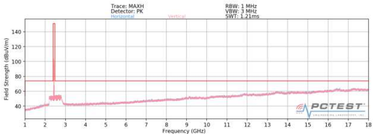
Plot 7-60. Radiated Spurious Plot above 1GHz SISO ANT2 (802.11ax OFDMA – 26 Tones – Ch. 6)
