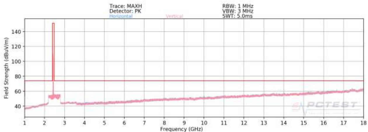
Plot 7-52. Radiated Spurious Plot above 1GHz SISO ANT1 (802.11ax OFDMA – 26 Tones – Ch. 6)
