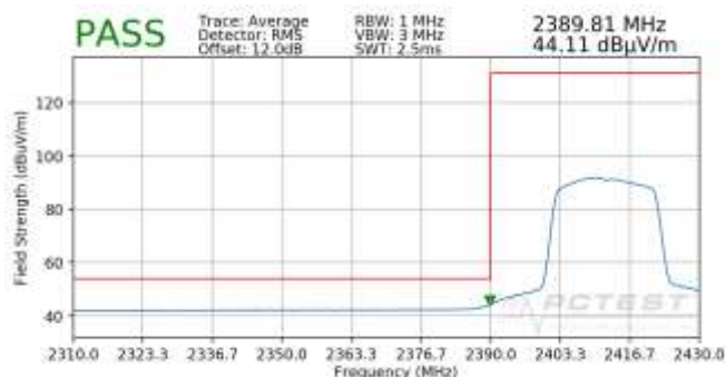
Plot 7-93. Radiated Restricted Lower Band Edge Measurement SISO ANT2 (Average – 242 Tones)
