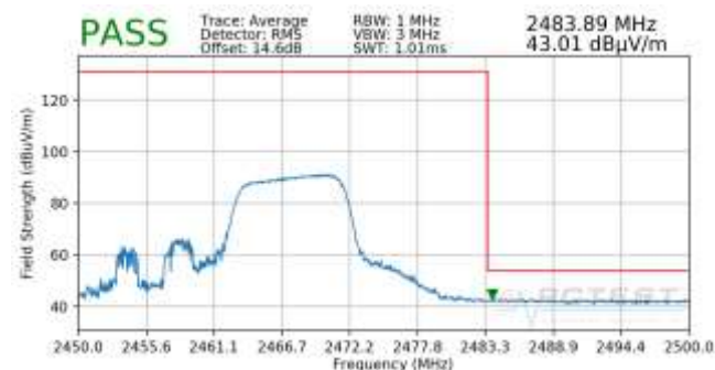
Plot 7-77. Radiated Restricted Upper Band Edge Measurement SISO ANT1 (Average – 106 Tones)
