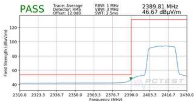
Plot 7-107. Radiated Restricted Lower Band Edge Measurement MIMO (Average – 242 Tones)
