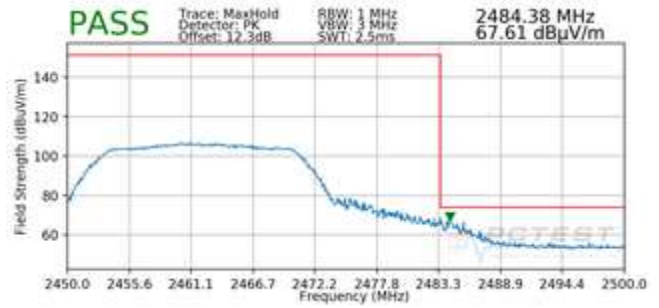
Plot 7-112. Radiated Restricted Band Edge Measurement MIMO with WCP (Peak)
