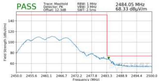
Plot 7-104. Radiated Restricted Upper Band Edge Measurement CDD (Peak)
