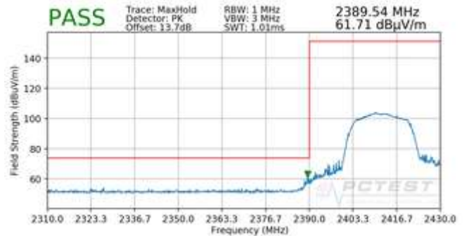
Plot 7-96. Radiated Restricted Lower Band Edge Measurement SISO ANT2 (Peak)
