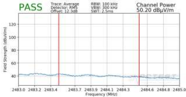
Plot 7-105. Radiated Restricted Band Edge Measurement CDD with WCP (Average)
