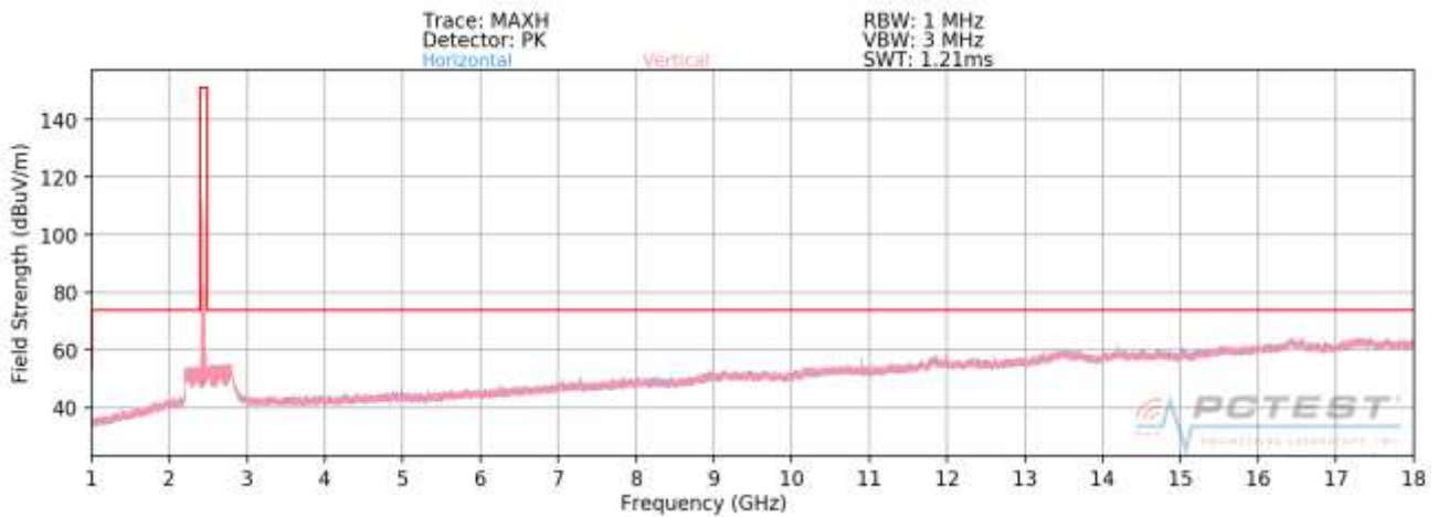
Plot 7-86. Radiated Spurious Plot above 1GHz MIMO/CDD (802.11g – Ch. 6)
