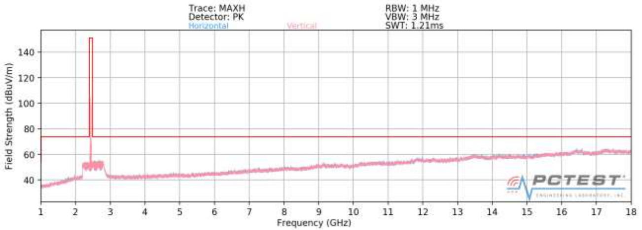
Plot 7-82. Radiated Spurious Plot above 1GHz SISO ANT2 (802.11b – Ch. 6)
