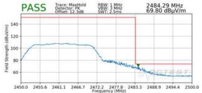
Plot 7-110. Radiated Restricted Upper Band Edge Measurement MIMO (Peak)
