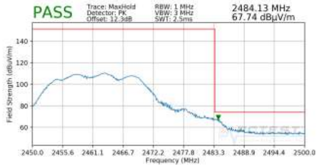
Plot 7-106. Radiated Restricted Band Edge Measurement CDD with WCP (Peak)
