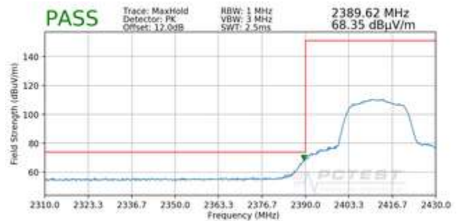
Plot 7-108. Radiated Restricted Lower Band Edge Measurement MIMO (Peak)
