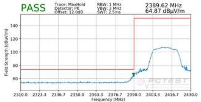
Plot 7-90. Radiated Restricted Lower Band Edge Measurement SISO ANT1 (Peak)
