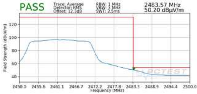
Plot 7-111. Radiated Restricted Band Edge Measurement MIMO with WCP (Average)
