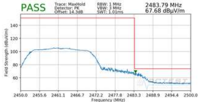
Plot 7-98. Radiated Restricted Upper Band Edge Measurement SISO ANT2 (Peak)
