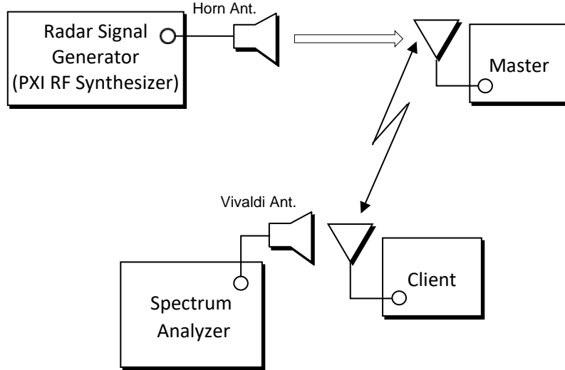
Figure 8-1. Radiated Test Setup
