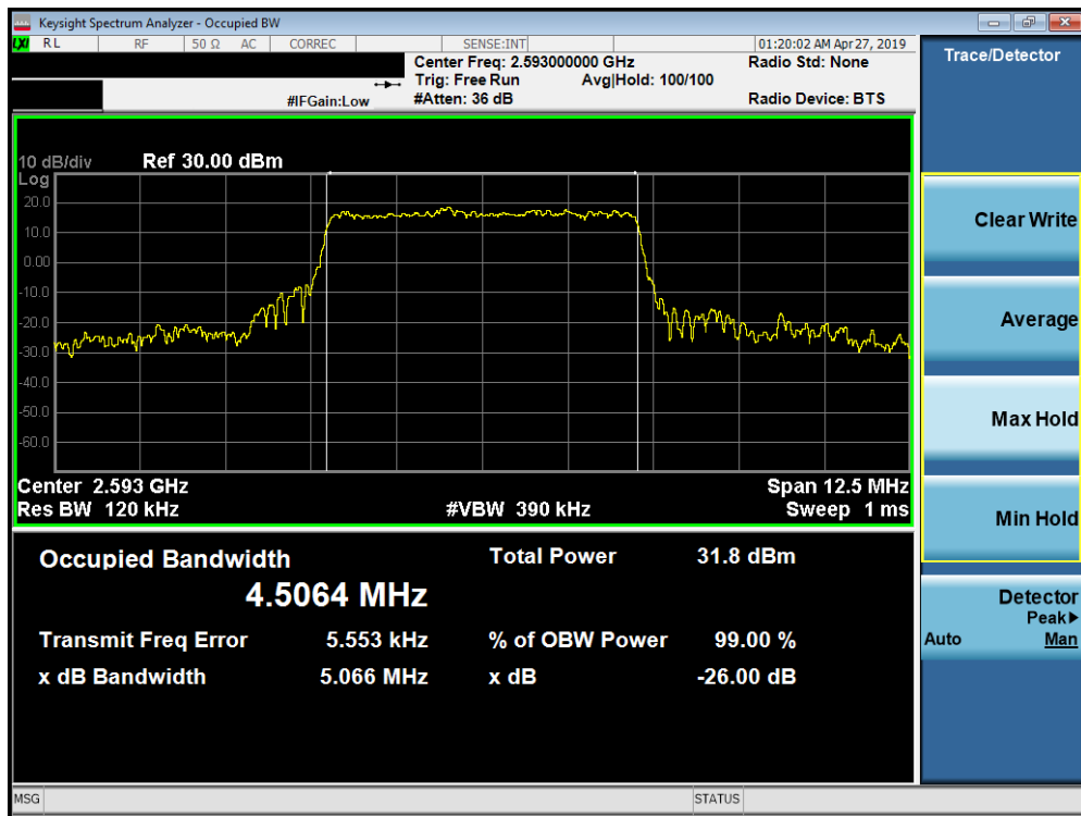
Plot 7-144. Occupied Bandwidth Plot (Band 41 PC2 – 5.0MHz 256-QAM - Full RB Configuration)
