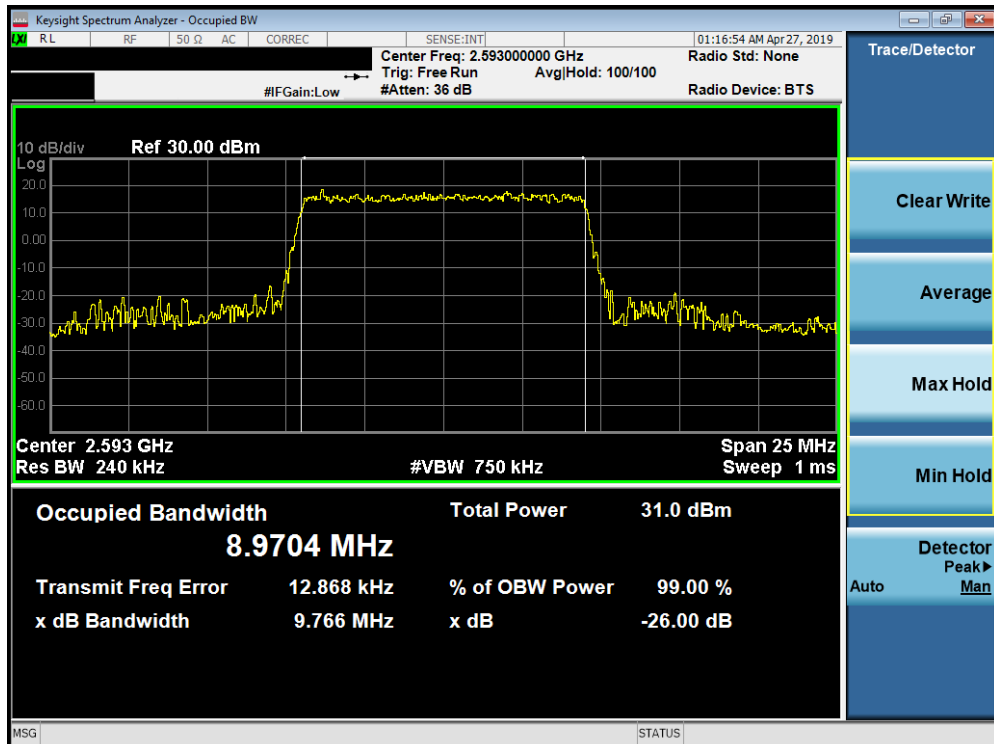
Plot 7-148. Occupied Bandwidth Plot (Band 41 PC2 - 10.0MHz 256-QAM - Full RB Configuration)
