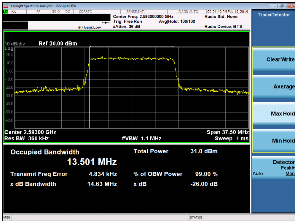
Plot 7-134. Occupied Bandwidth Plot (Band 41 PC3 / Band 38 - 15.0MHz 16-QAM - Full RB Configuration)
