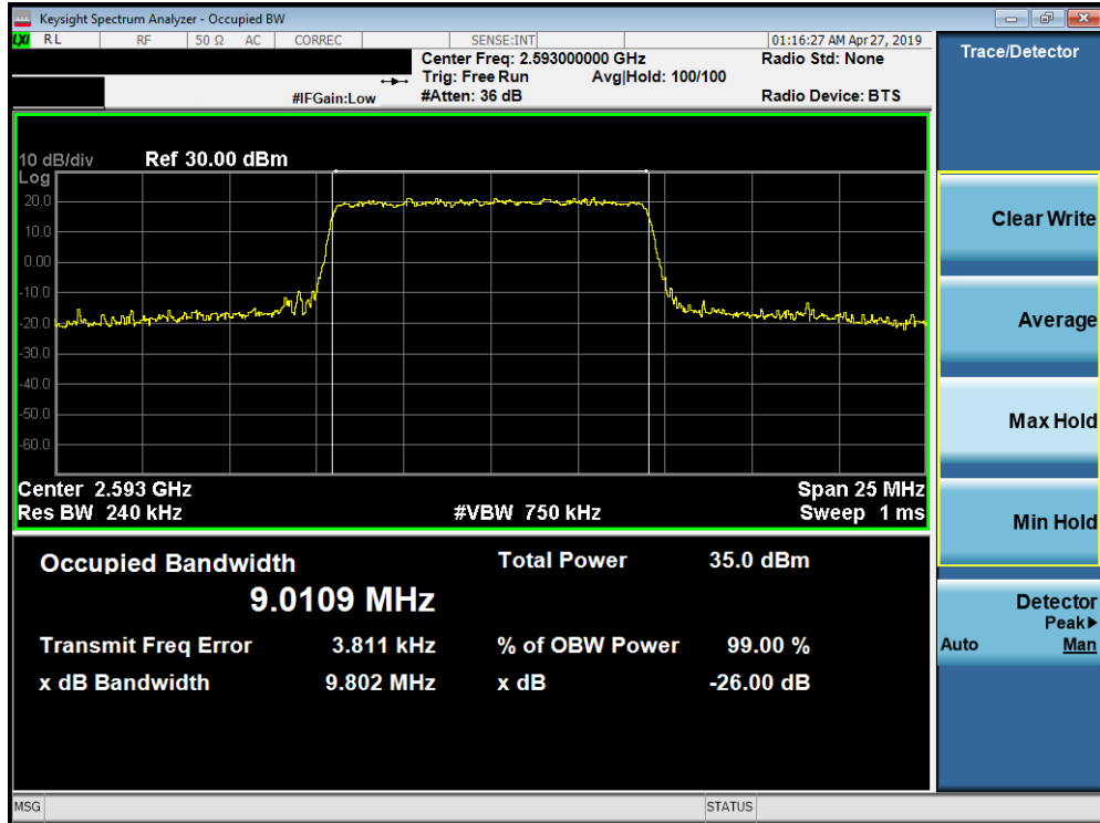
Plot 7-145. Occupied Bandwidth Plot (Band 41 PC2 - 10.0MHz QPSK - Full RB Configuration)
