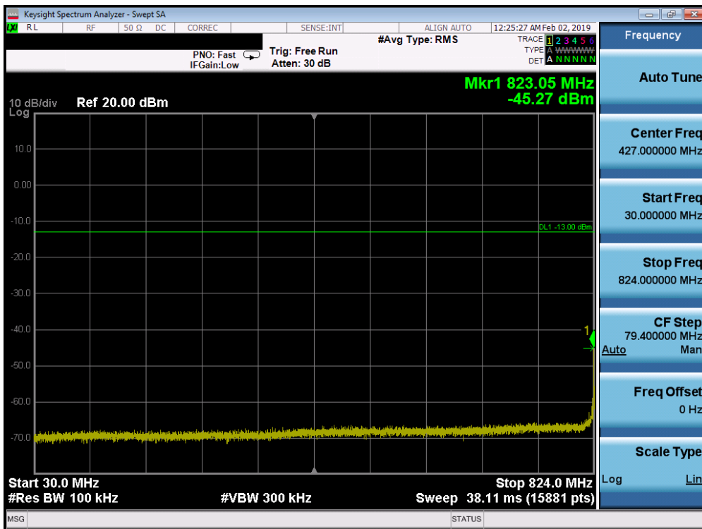
Plot 7-181. Conducted Spurious Plot (Band 26/5 - 10.0MHz QPSK - RB Size 1, RB Offset 0 - Mid Channel)
