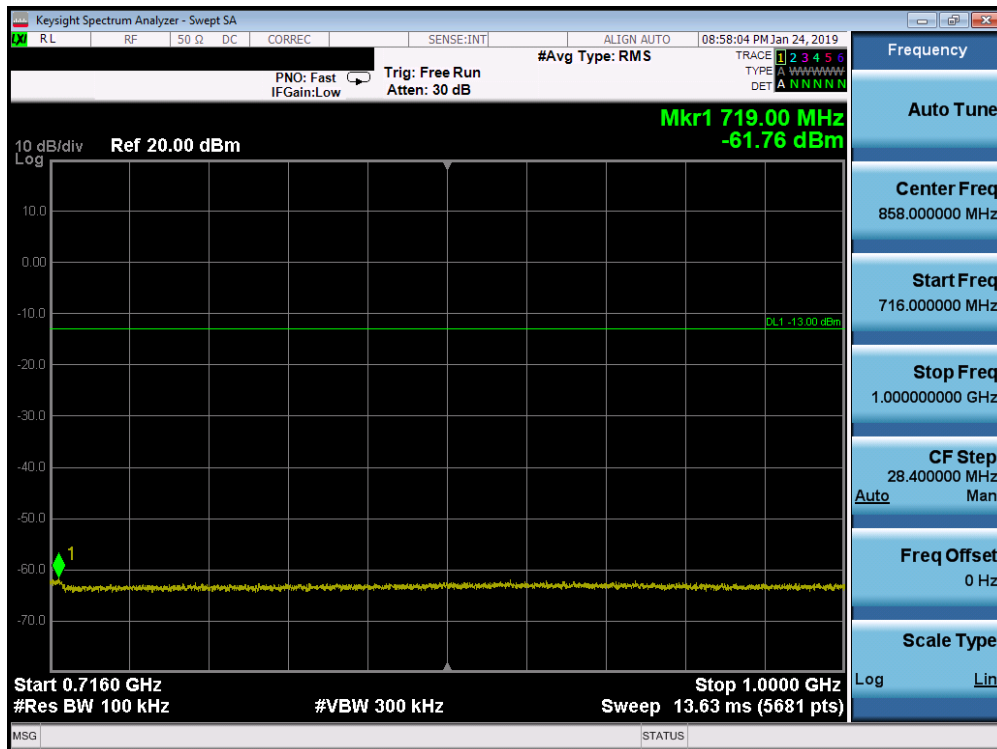
Plot 7-167. Conducted Spurious Plot (Band 12 - 10.0MHz QPSK - RB Size 1, RB Offset 0 - Low Channel)
