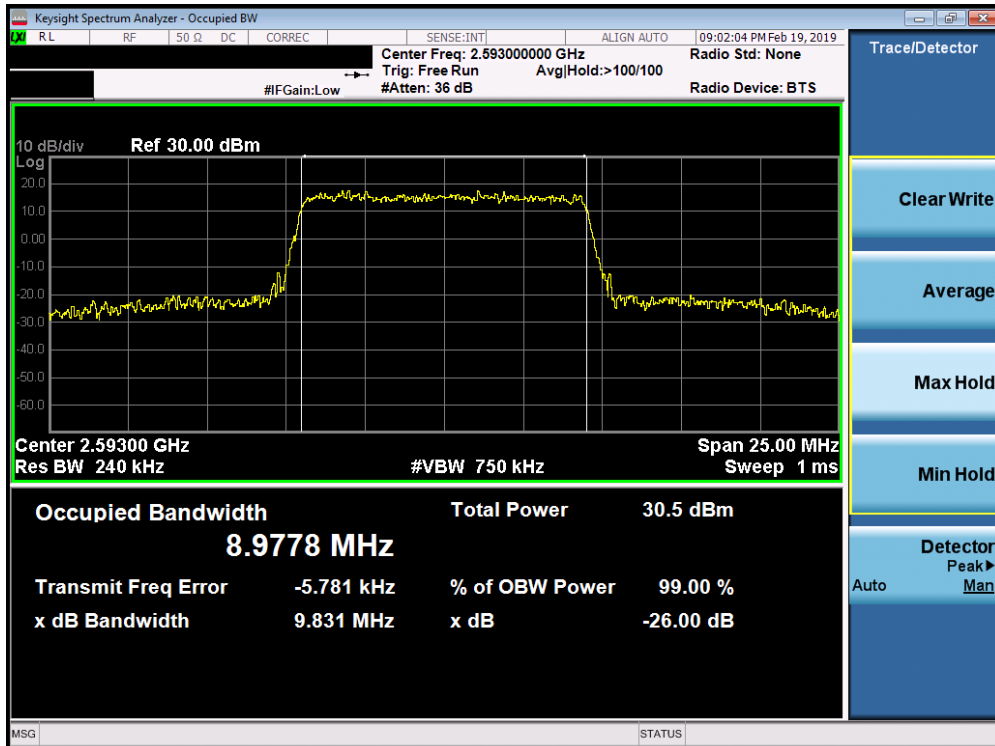
Plot 7-130. Occupied Bandwidth Plot (Band 41 PC3 / Band 38 - 10.0MHz 16-QAM - Full RB Configuration)
