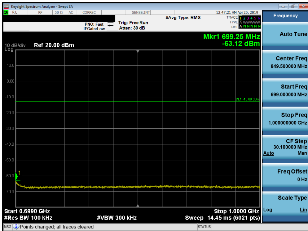
Plot 7-164. Conducted Spurious Plot (Band 71 - 20.0MHz QPSK - RB Size 1, RB Offset 0 - High Channel)
