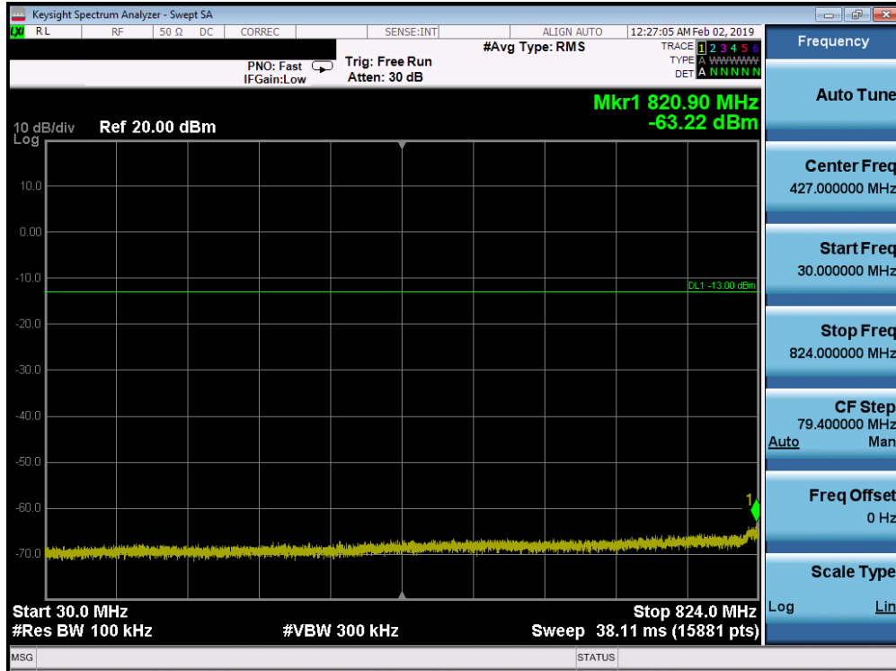
Plot 7-184. Conducted Spurious Plot (Band 26/5 - 10.0MHz QPSK - RB Size 1, RB Offset 0 - High Channel)
