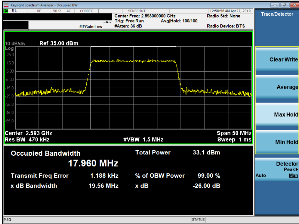
Plot 7-155. Occupied Bandwidth Plot (Band 41 PC2 - 20.0MHz 64-QAM - Full RB Configuration)
