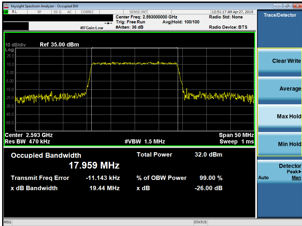
Plot 7-156. Occupied Bandwidth Plot (Band 41 PC2 - 20.0MHz 256-QAM - Full RB Configuration)
