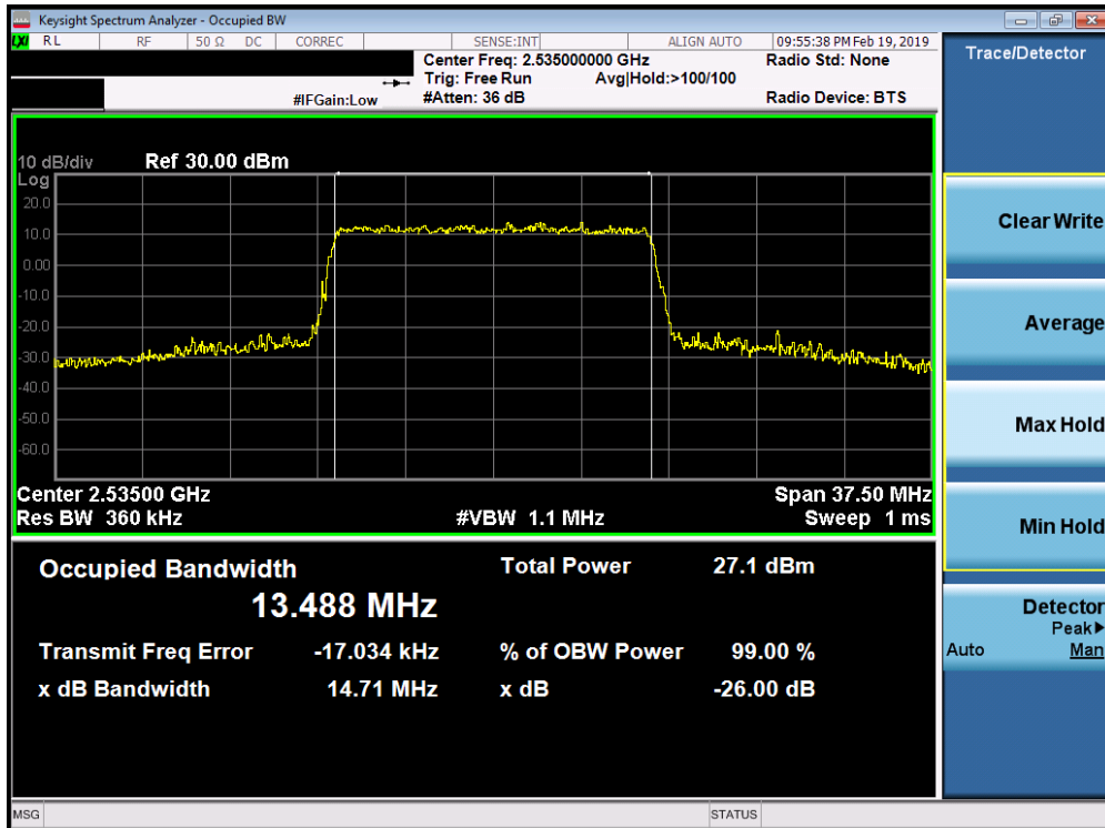
Plot 7-120. Occupied Bandwidth Plot (Band 7 - 15.0MHz 256-QAM - Full RB Configuration)
