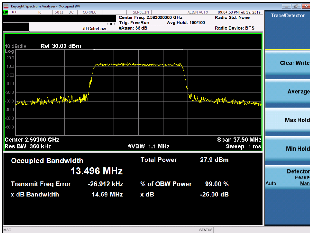
Plot 7-136. Occupied Bandwidth Plot (Band 41 PC3 / Band 38 - 15.0MHz 256-QAM - Full RB Configuration)
