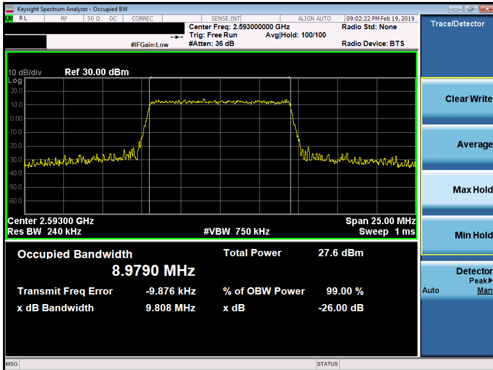
Plot 7-132. Occupied Bandwidth Plot (Band 41 PC3 / Band 38 - 10.0MHz 256-QAM - Full RB Configuration)
