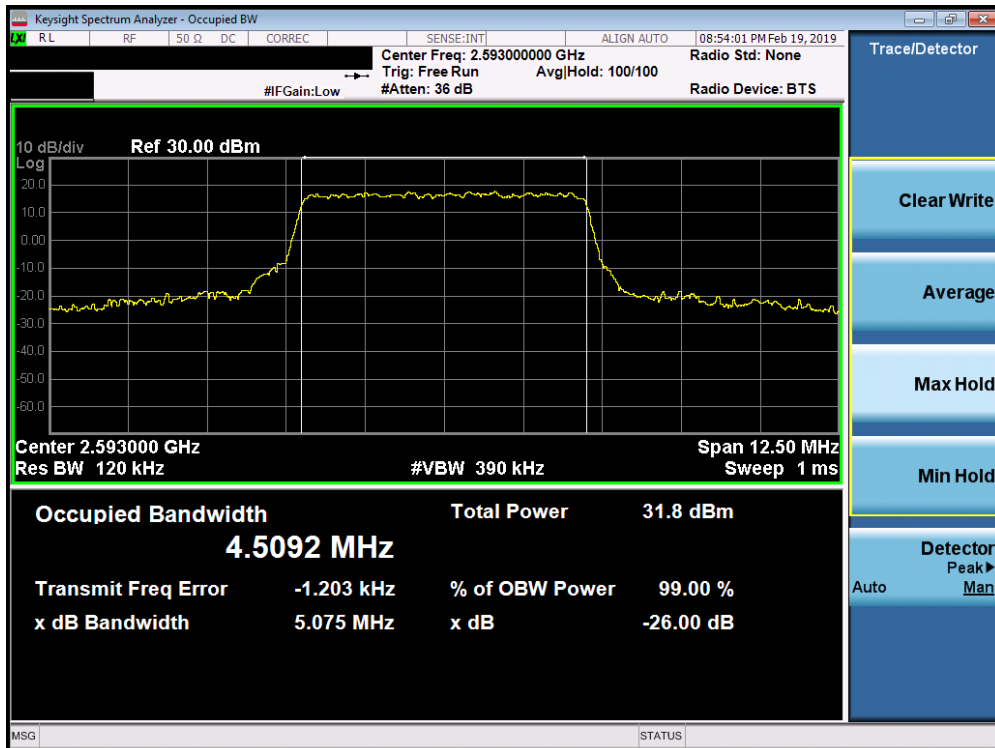
Plot 7-126. Occupied Bandwidth Plot (Band 41 PC3 / Band 38 – 5.0MHz 16-QAM - Full RB Configuration)
