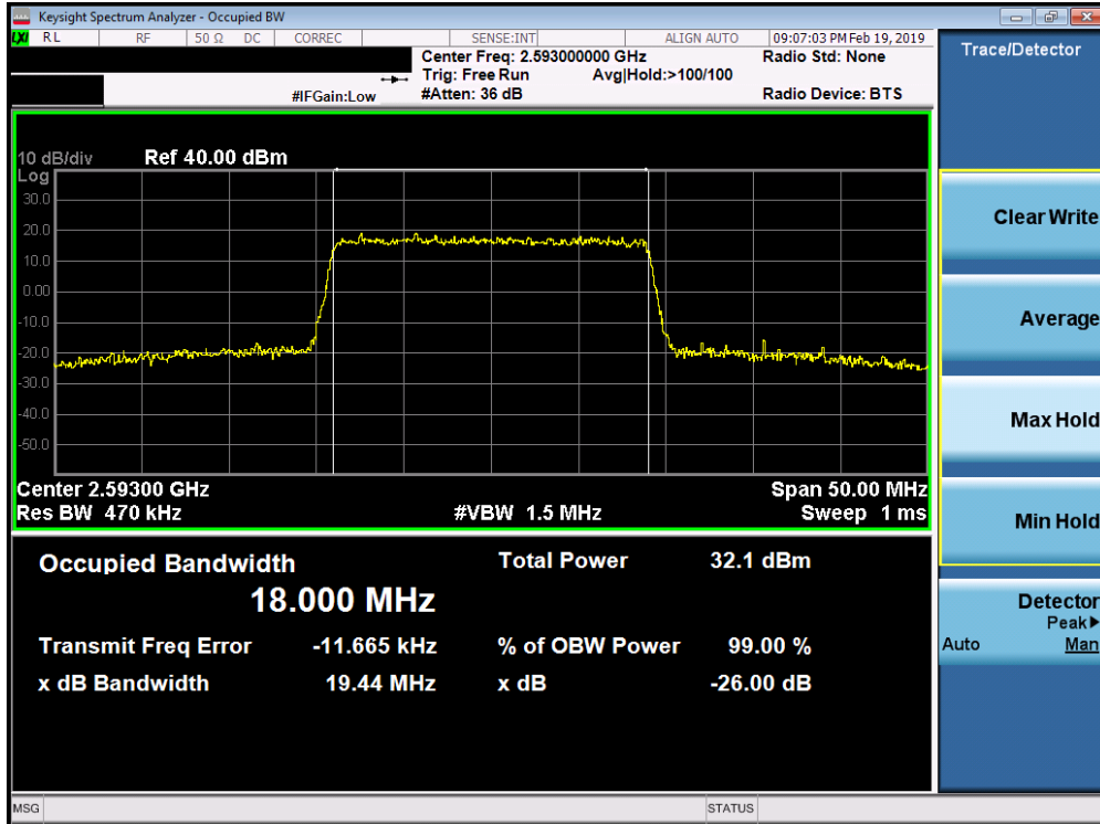
Plot 7-137. Occupied Bandwidth Plot (Band 41 PC3 / Band 38 - 20.0MHz QPSK - Full RB Configuration)
