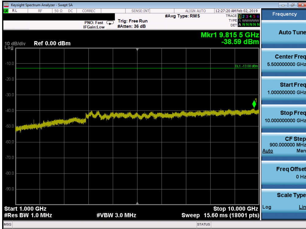
Plot 7-186. Conducted Spurious Plot (Band 26/5 - 10.0MHz QPSK - RB Size 1, RB Offset 0 - High Channel)
