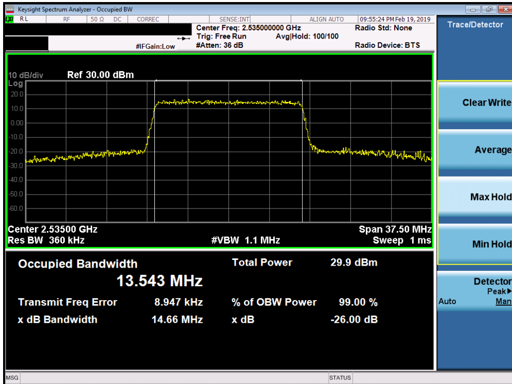
Plot 7-118. Occupied Bandwidth Plot (Band 7 - 15.0MHz 16-QAM - Full RB Configuration)
