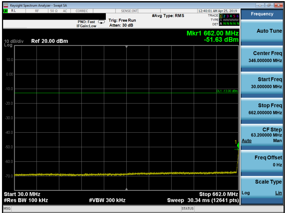
Plot 7-157. Conducted Spurious Plot (Band 71 - 20.0MHz QPSK - RB Size 1, RB Offset 0 - Low Channel)
