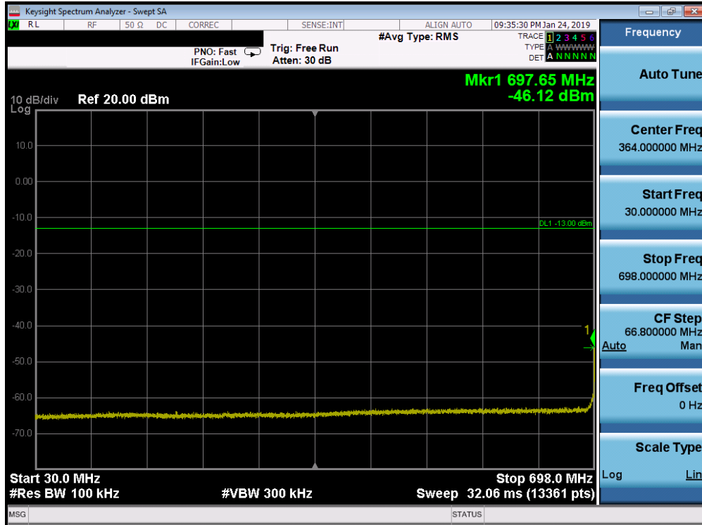
Plot 7-172. Conducted Spurious Plot (Band 12 - 10.0MHz QPSK - RB Size 1, RB Offset 0 - High Channel)
