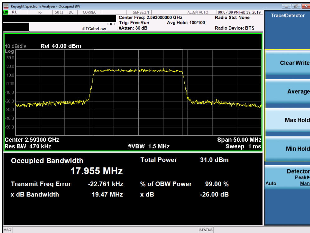
Plot 7-138. Occupied Bandwidth Plot (Band 41 PC3 / Band 38 - 20.0MHz 16-QAM - Full RB Configuration)
