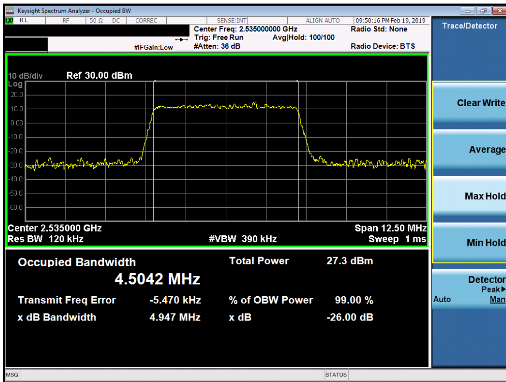
Plot 7-112. Occupied Bandwidth Plot (Band 7 – 5.0MHz 256-QAM - Full RB Configuration)
