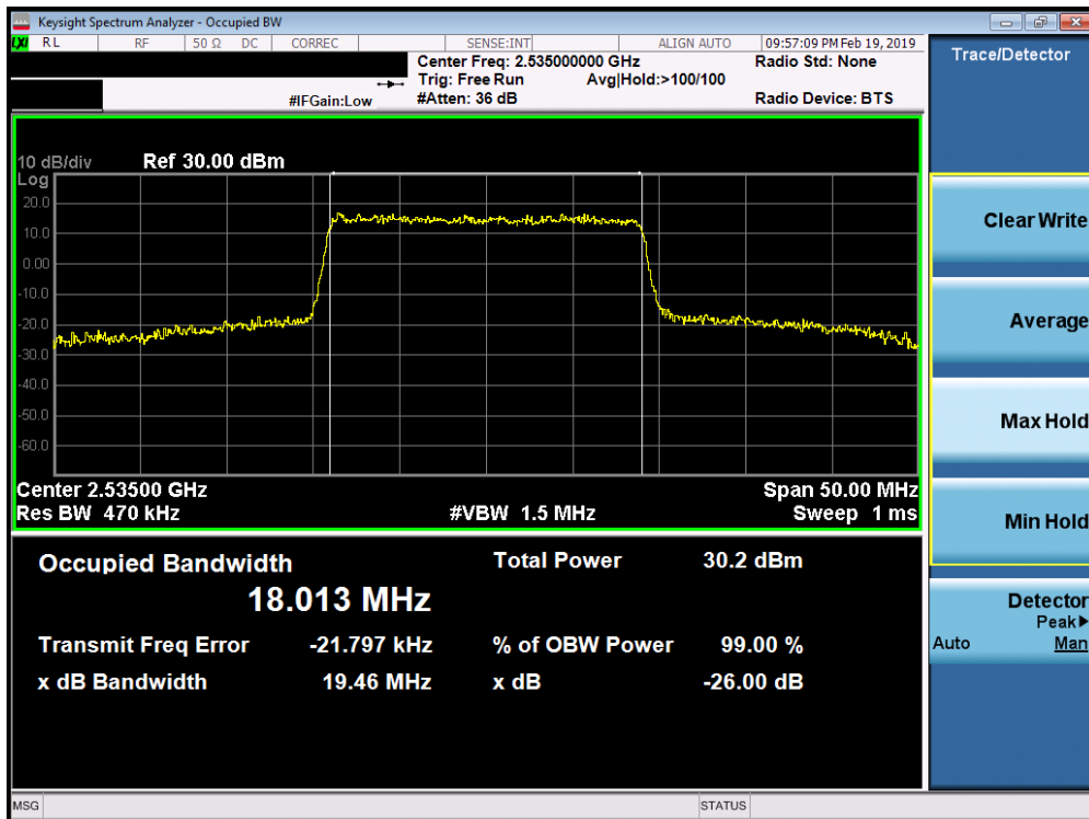
Plot 7-122. Occupied Bandwidth Plot (Band 7 - 20.0MHz 16-QAM - Full RB Configuration)
