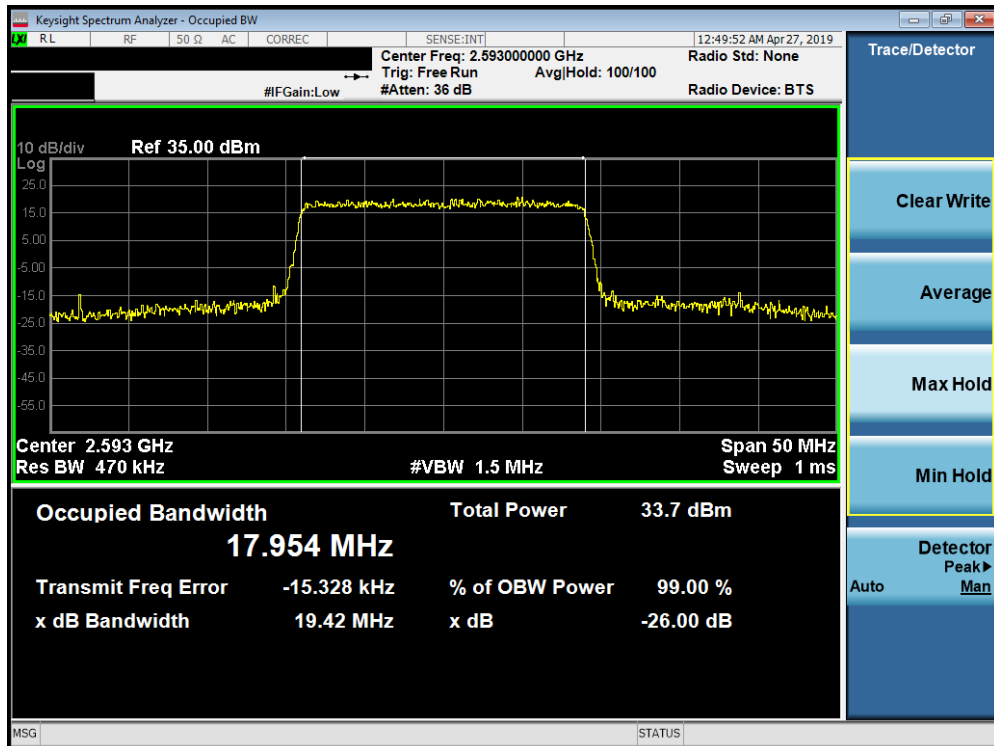
Plot 7-154. Occupied Bandwidth Plot (Band 41 PC2 - 20.0MHz 16-QAM - Full RB Configuration)
