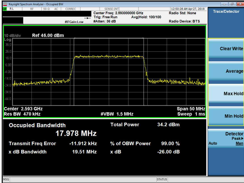
Plot 7-153. Occupied Bandwidth Plot (Band 41 PC2 - 20.0MHz QPSK - Full RB Configuration)
