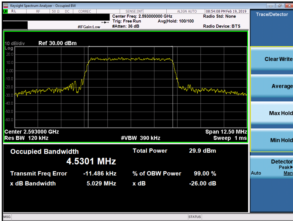
Plot 7-127. Occupied Bandwidth Plot (Band 41 PC3 / Band 38 – 5.0MHz 64-QAM - Full RB Configuration)
