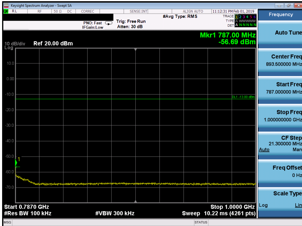
Plot 7-176. Conducted Spurious Plot (Band 13 - 10.0MHz QPSK - RB Size 1, RB Offset 0)
