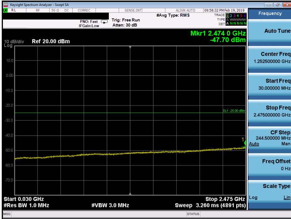
Plot 7-205. Conducted Spurious Plot (Band 7 - 20.0MHz QPSK - RB Size 1, RB Offset 0 - Low Channel)
