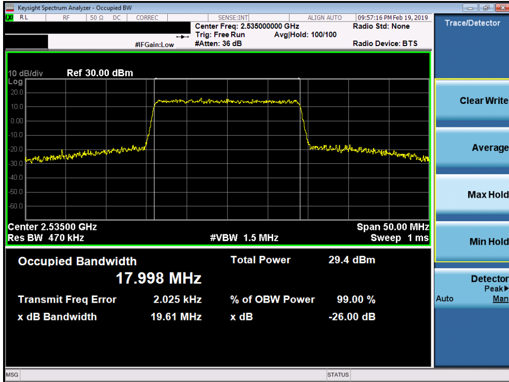
Plot 7-123. Occupied Bandwidth Plot (Band 7 - 20.0MHz 64-QAM - Full RB Configuration)
