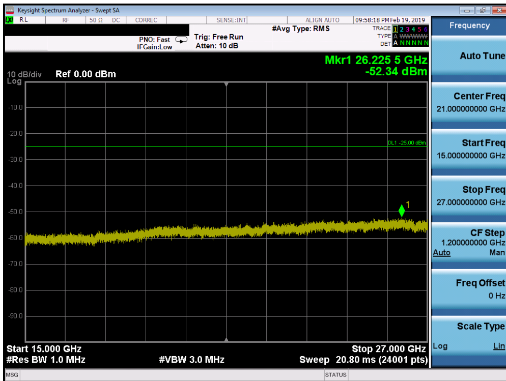
Plot 7-210. Conducted Spurious Plot (Band 7 - 20.0MHz QPSK - RB Size 1, RB Offset 0 - Mid Channel)
