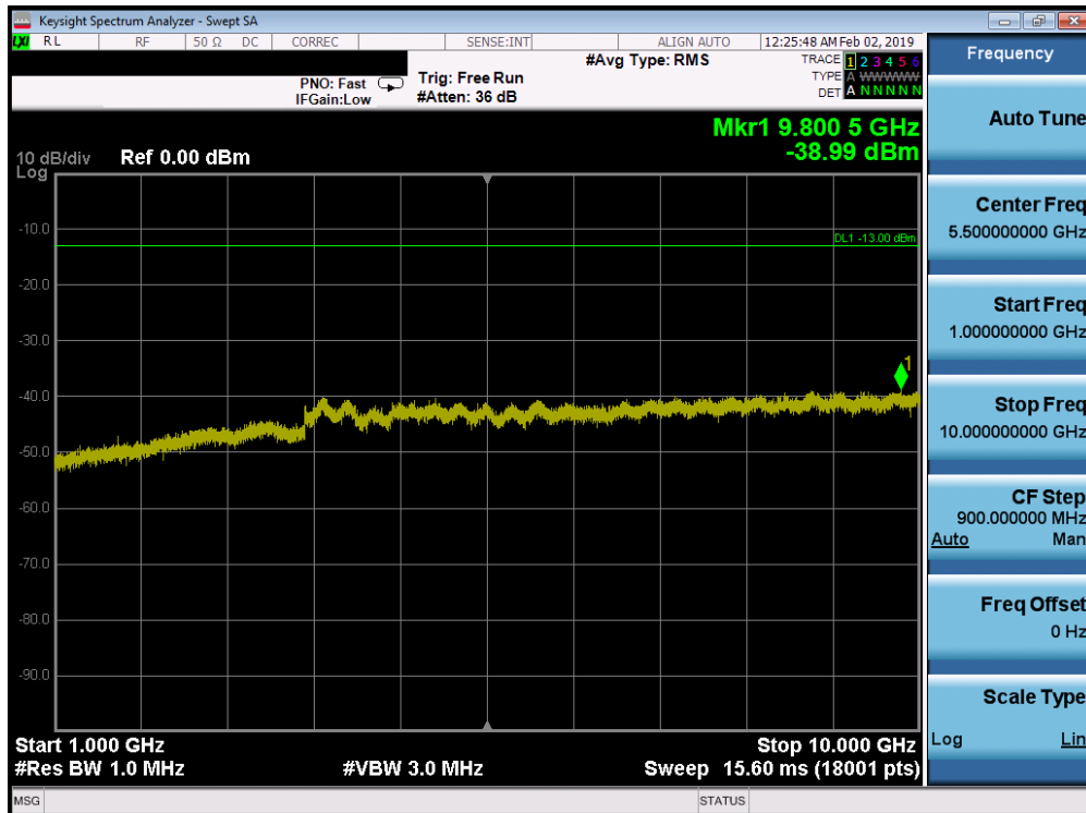
Plot 7-183. Conducted Spurious Plot (Band 26/5 - 10.0MHz QPSK - RB Size 1, RB Offset 0 - Mid Channel)
