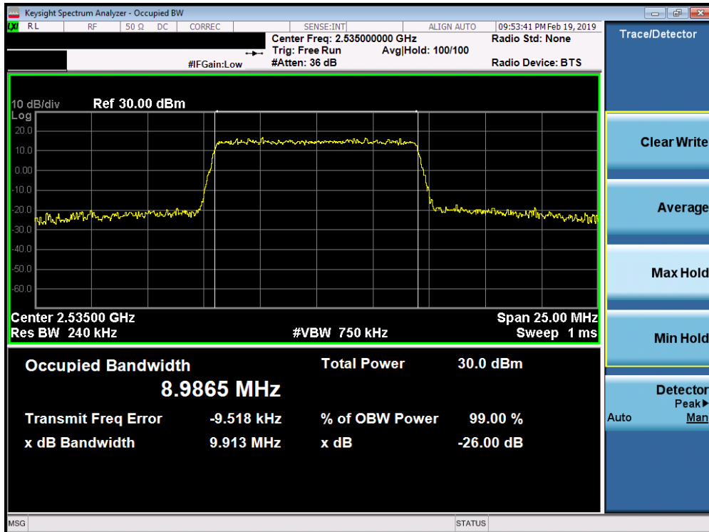
Plot 7-114. Occupied Bandwidth Plot (Band 7 - 10.0MHz 16-QAM - Full RB Configuration)
