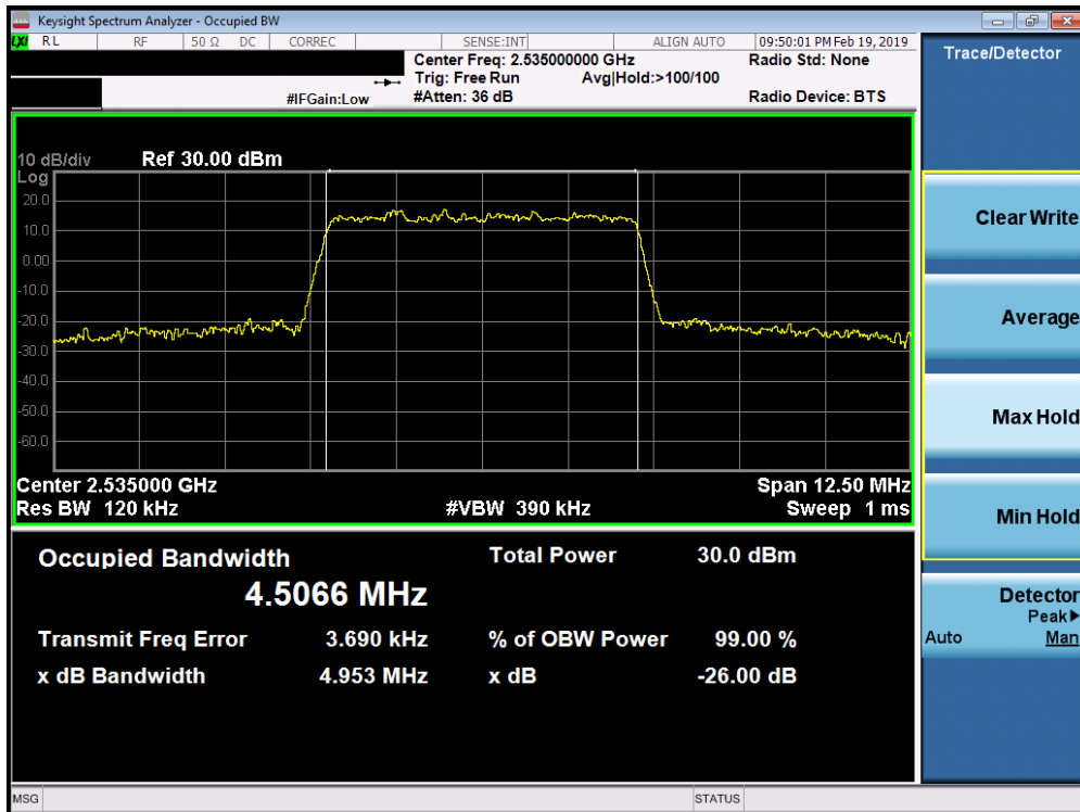
Plot 7-110. Occupied Bandwidth Plot (Band 7 – 5.0MHz 16-QAM - Full RB Configuration)
