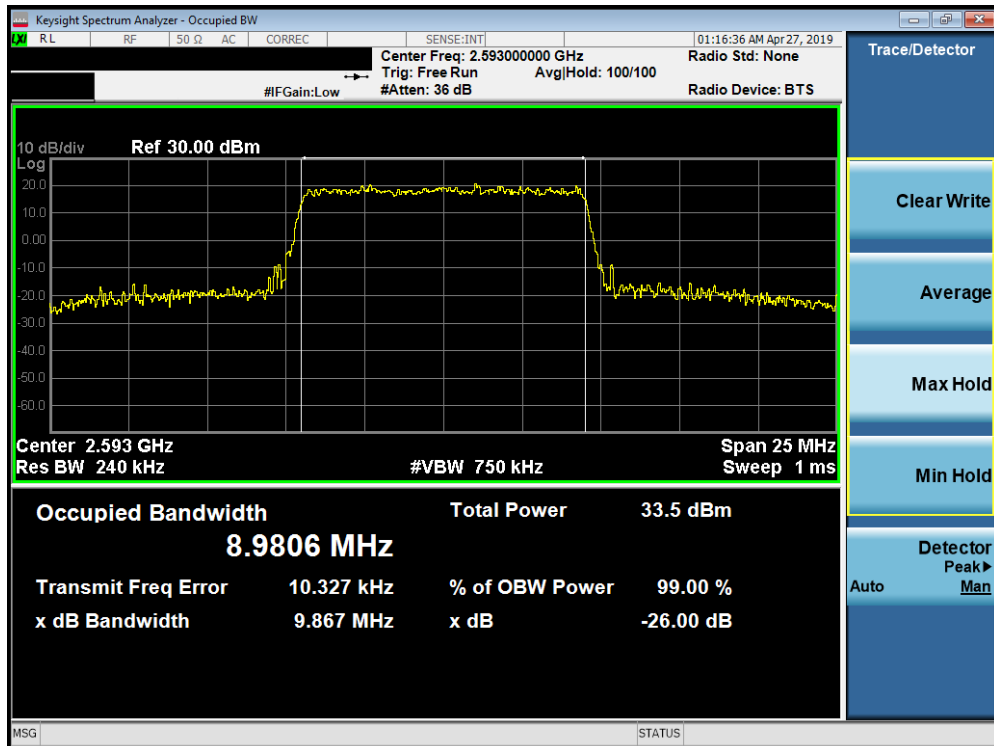
Plot 7-146. Occupied Bandwidth Plot (Band 41 PC2 - 10.0MHz 16-QAM - Full RB Configuration)
