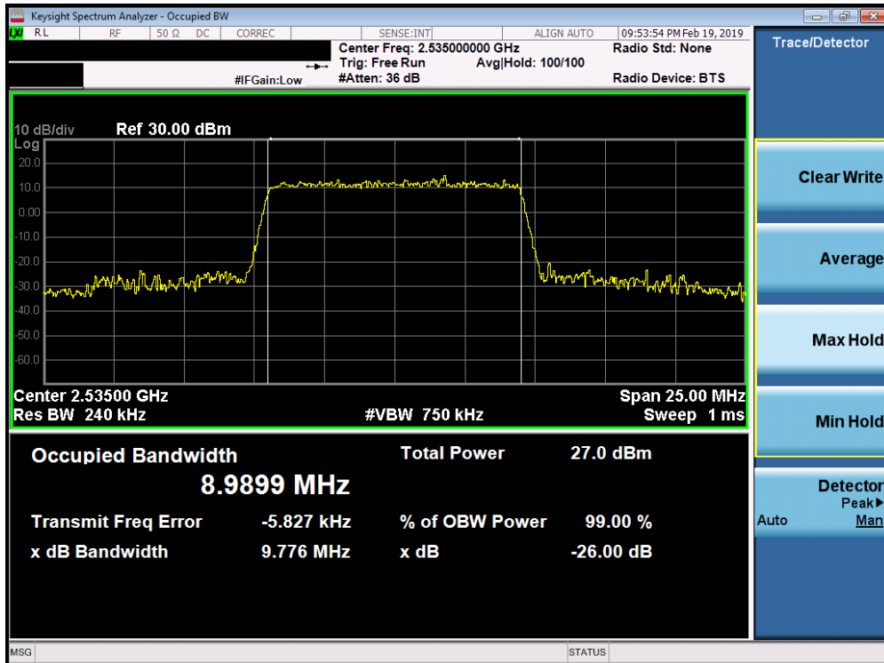
Plot 7-116. Occupied Bandwidth Plot (Band 7 - 10.0MHz 256-QAM - Full RB Configuration)
