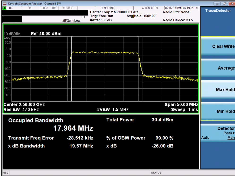
Plot 7-139. Occupied Bandwidth Plot (Band 41 PC3 / Band 38 - 20.0MHz 64-QAM - Full RB Configuration)
