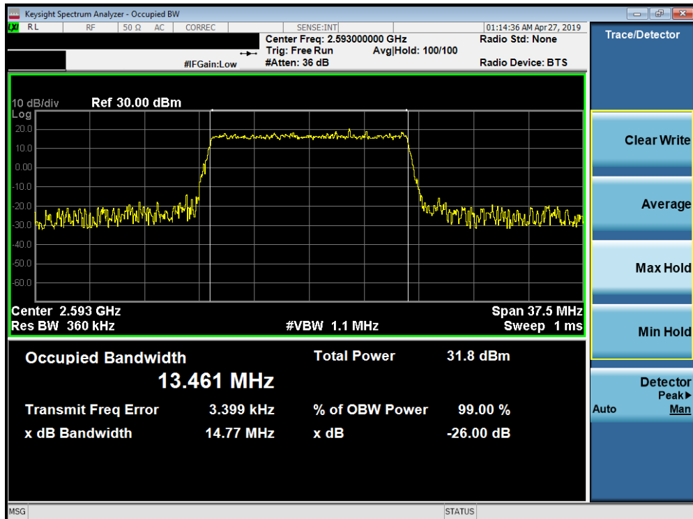
Plot 7-152. Occupied Bandwidth Plot (Band 41 PC2 - 15.0MHz 256-QAM - Full RB Configuration)
