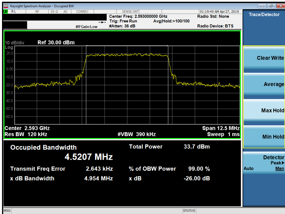
Plot 7-142. Occupied Bandwidth Plot (Band 41 PC2 – 5.0MHz 16-QAM - Full RB Configuration)
