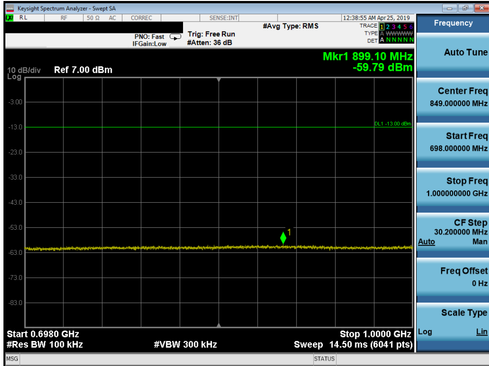
Plot 7-161. Conducted Spurious Plot (Band 71 - 20.0MHz QPSK - RB Size 1, RB Offset 0 - Mid Channel)
