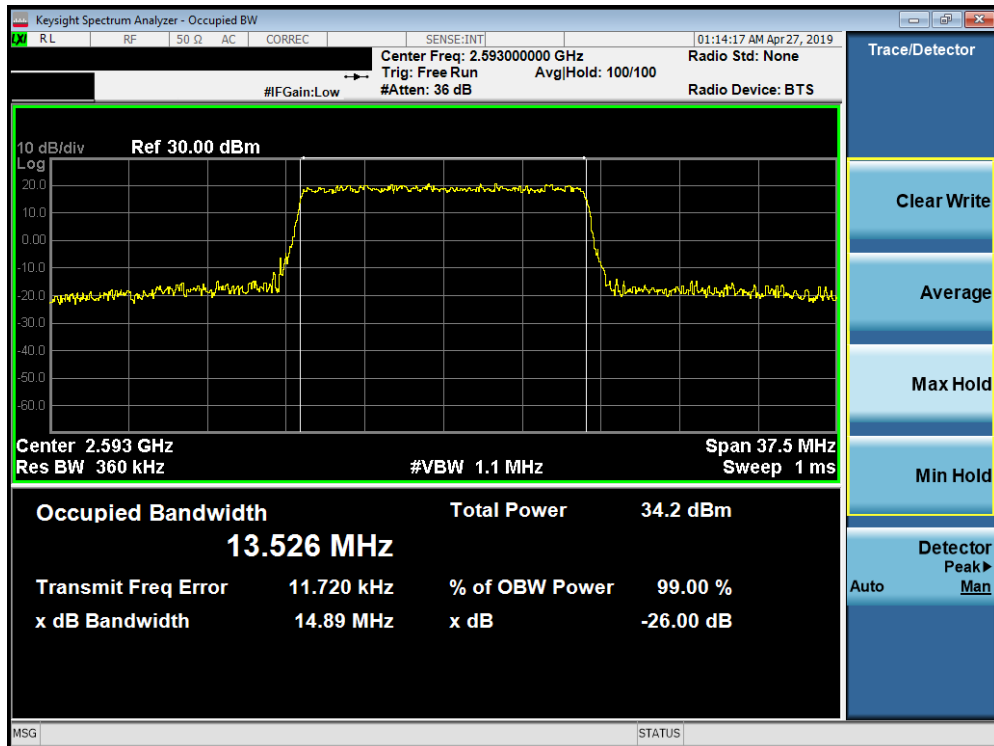
Plot 7-150. Occupied Bandwidth Plot (Band 41 PC2 - 15.0MHz 16-QAM - Full RB Configuration)
