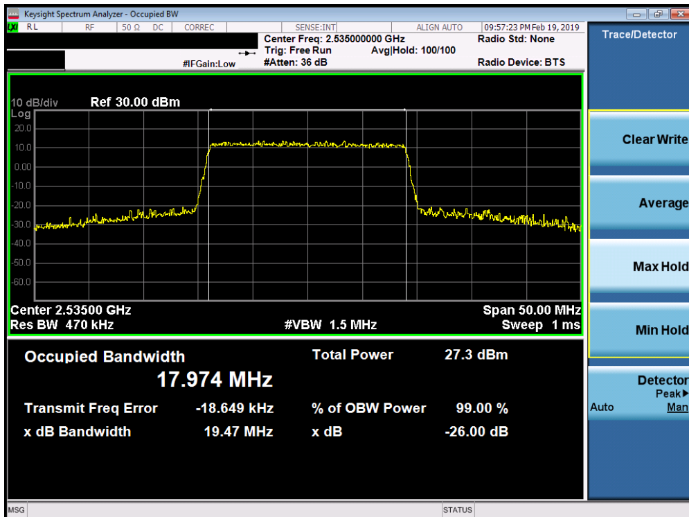
Plot 7-124. Occupied Bandwidth Plot (Band 7 - 20.0MHz 256-QAM - Full RB Configuration)
