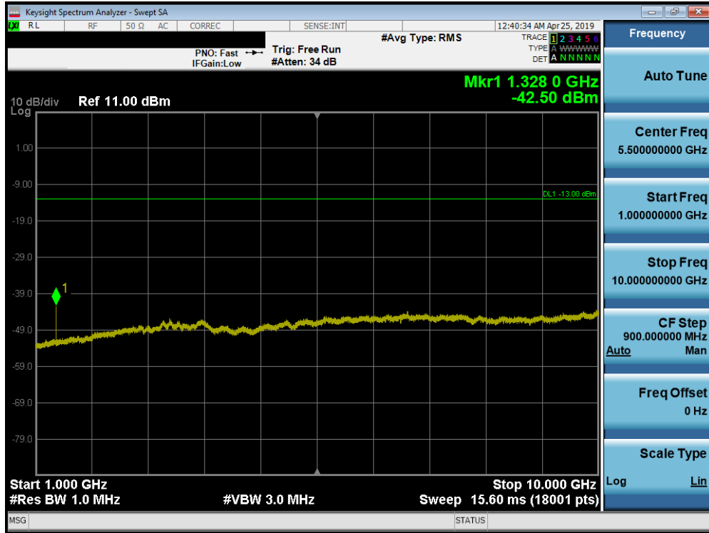
Plot 7-159. Conducted Spurious Plot (Band 71 - 20.0MHz QPSK - RB Size 1, RB Offset 0 - Low Channel)
