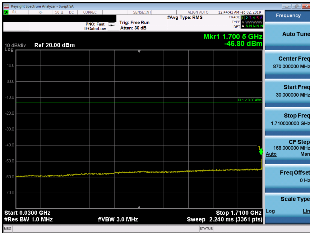
Plot 7-190. Conducted Spurious Plot (Band 66/4 - 20.0MHz QPSK - RB Size 1, RB Offset 0 - Mid Channel)
