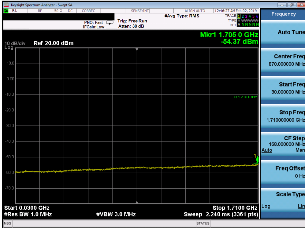
Plot 7-193. Conducted Spurious Plot (Band 66/4 - 20.0MHz QPSK - RB Size 1, RB Offset 0 - High Channel)
