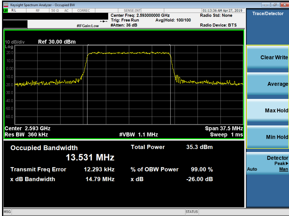
Plot 7-149. Occupied Bandwidth Plot (Band 41 PC2 - 15.0MHz QPSK - Full RB Configuration)
