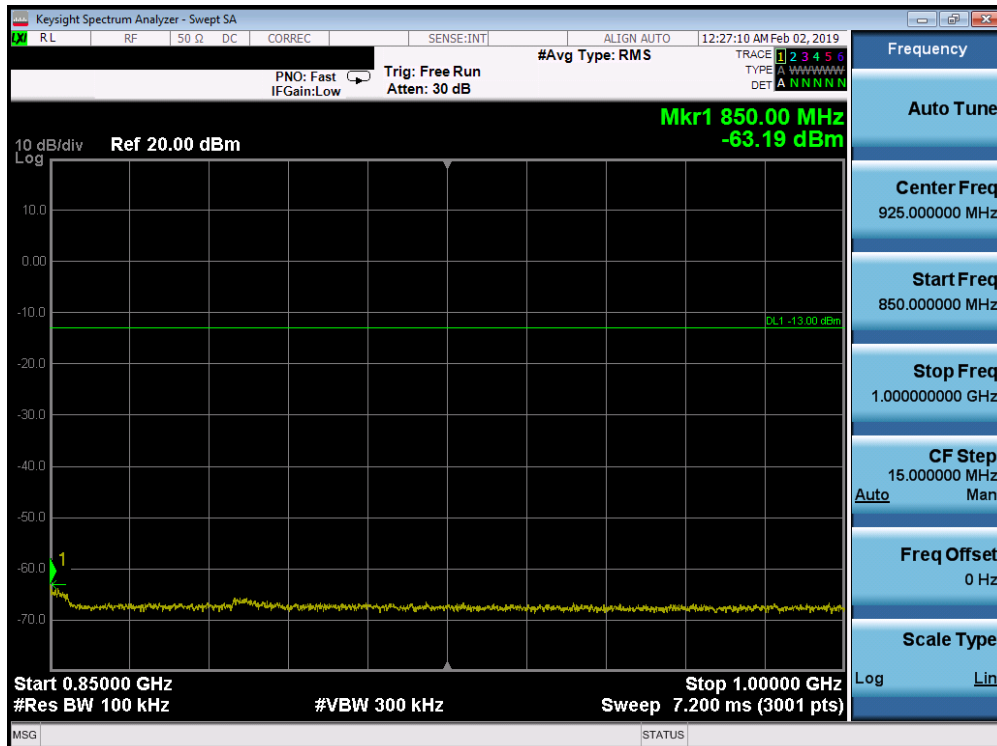
Plot 7-185. Conducted Spurious Plot (Band 26/5 - 10.0MHz QPSK - RB Size 1, RB Offset 0 - High Channel)
