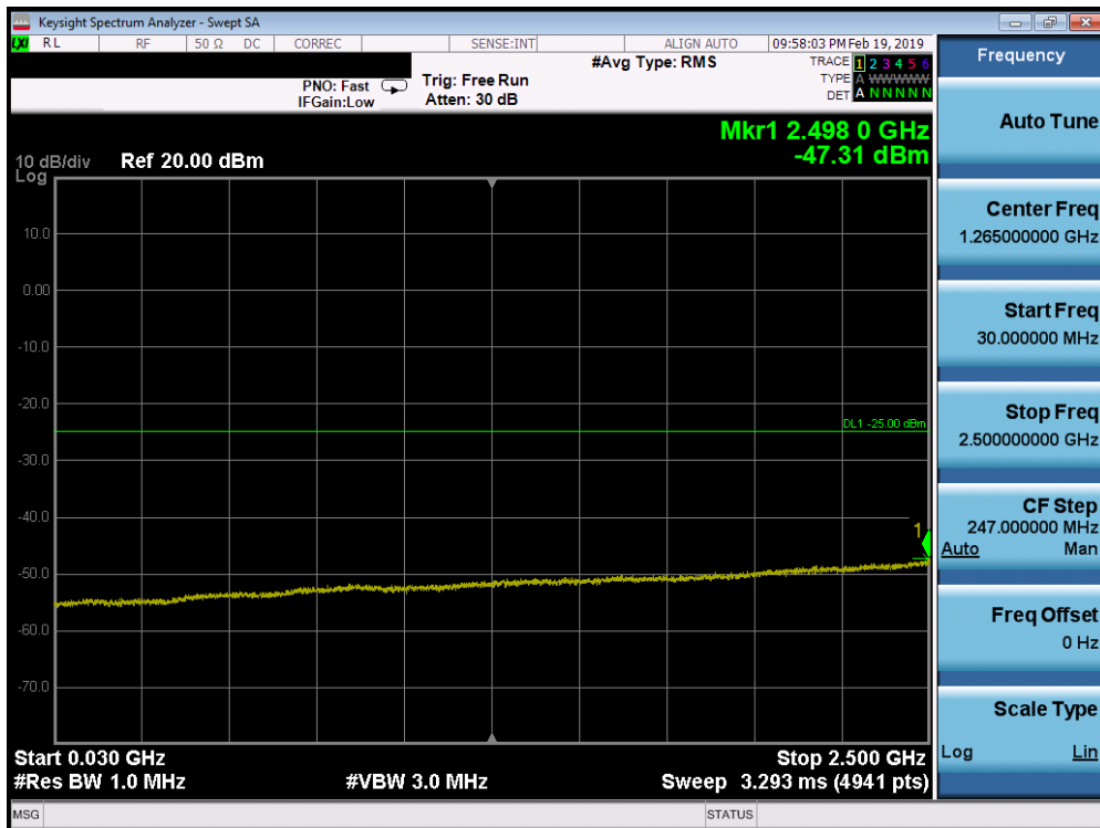
Plot 7-208. Conducted Spurious Plot (Band 7 - 20.0MHz QPSK - RB Size 1, RB Offset 0 - Mid Channel)
