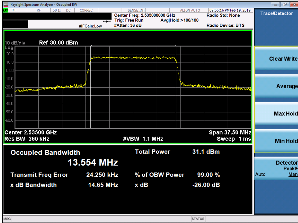
Plot 7-117. Occupied Bandwidth Plot (Band 7 - 15.0MHz QPSK - Full RB Configuration)
