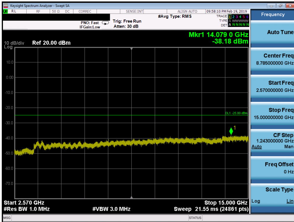
Plot 7-209. Conducted Spurious Plot (Band 7 - 20.0MHz QPSK - RB Size 1, RB Offset 0 - Mid Channel)
