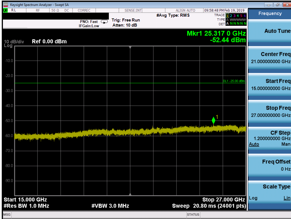
Plot 7-207. Conducted Spurious Plot (Band 7 - 20.0MHz QPSK - RB Size 1, RB Offset 0 - Low Channel)
