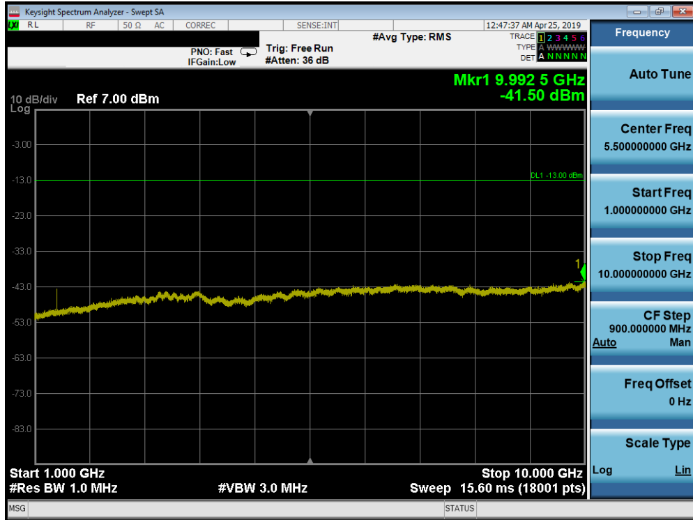
Plot 7-165. Conducted Spurious Plot (Band 71 - 20.0MHz QPSK - RB Size 1, RB Offset 0 - High Channel)
