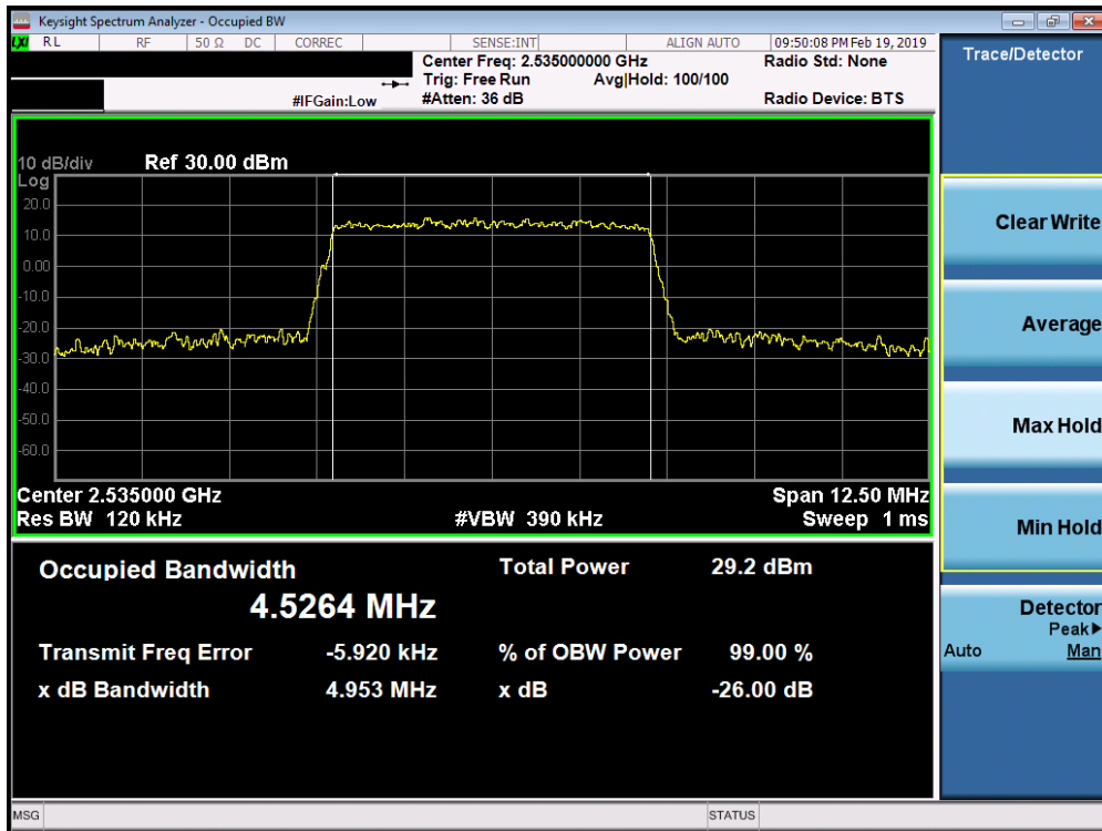
Plot 7-111. Occupied Bandwidth Plot (Band 7 – 5.0MHz 64-QAM - Full RB Configuration)
