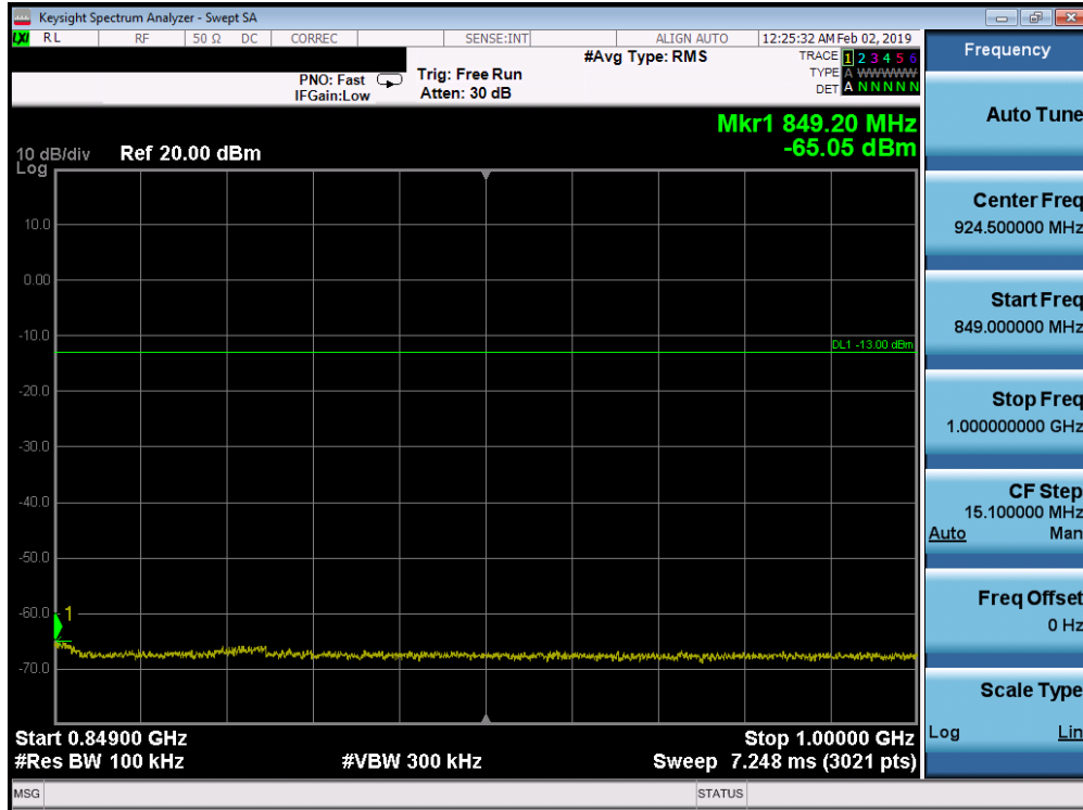
Plot 7-182. Conducted Spurious Plot (Band 26/5 - 10.0MHz QPSK - RB Size 1, RB Offset 0 - Mid Channel)
