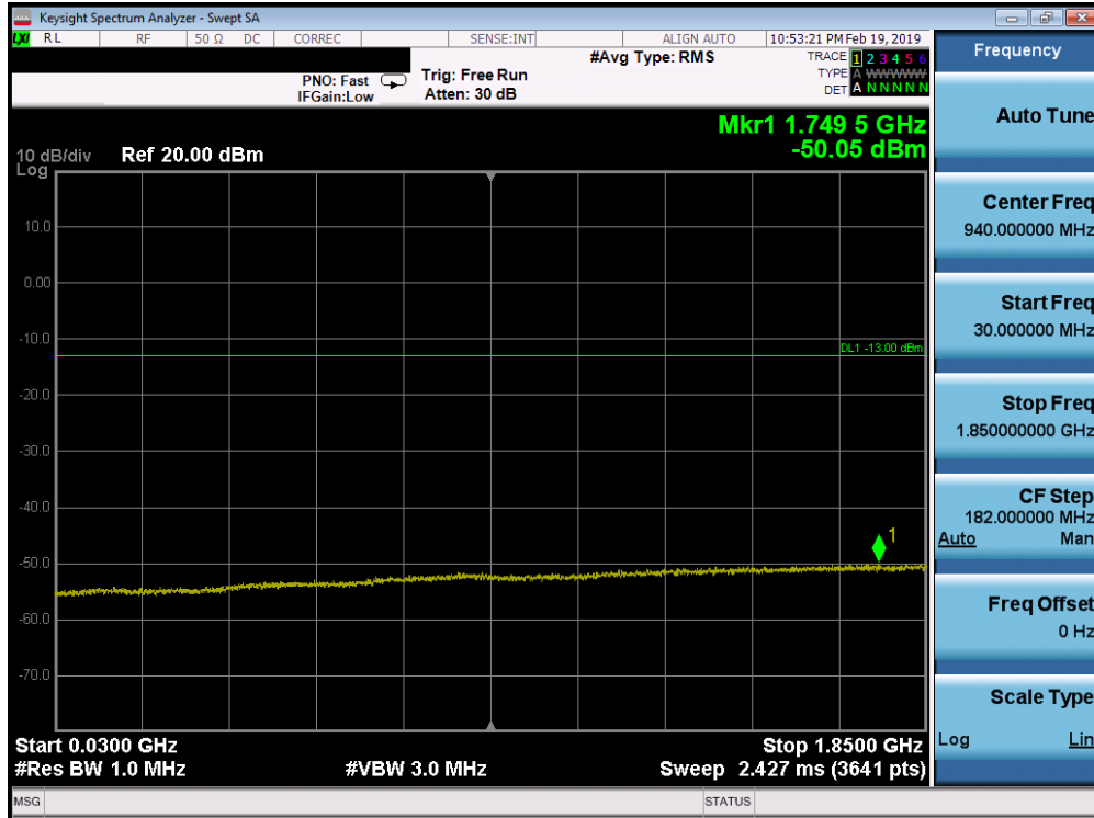
Plot 7-202. Conducted Spurious Plot (Band 25/2- 20.0MHz QPSK - RB Size 1, RB Offset 0 - High Channel)
