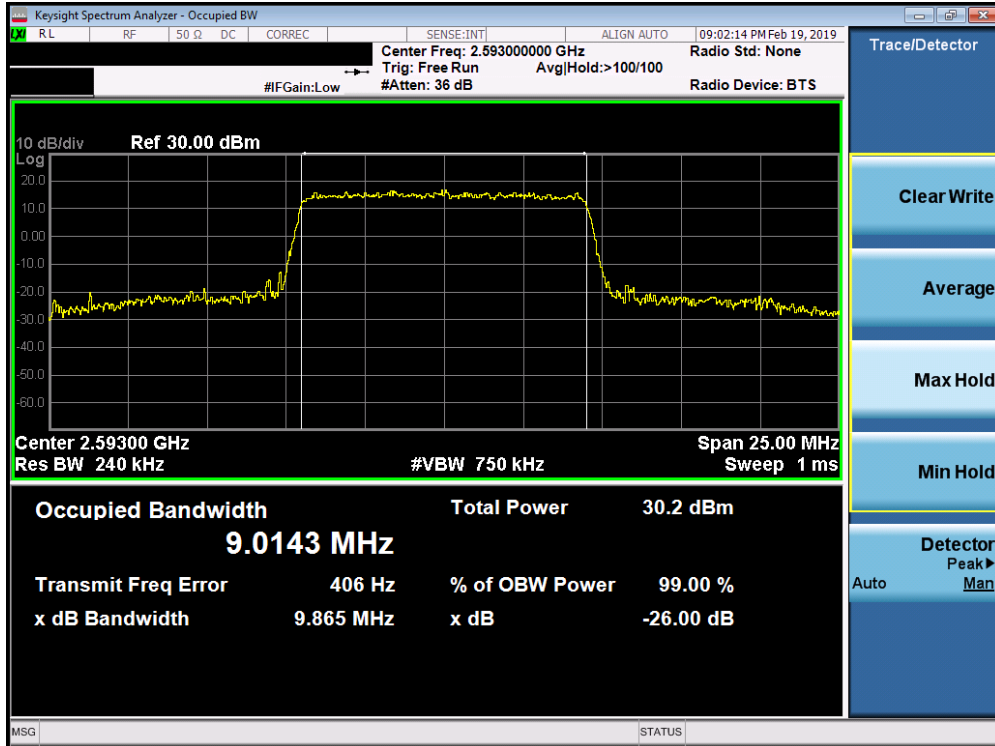
Plot 7-131. Occupied Bandwidth Plot (Band 41 PC3 / Band 38 - 10.0MHz 64-QAM - Full RB Configuration)
