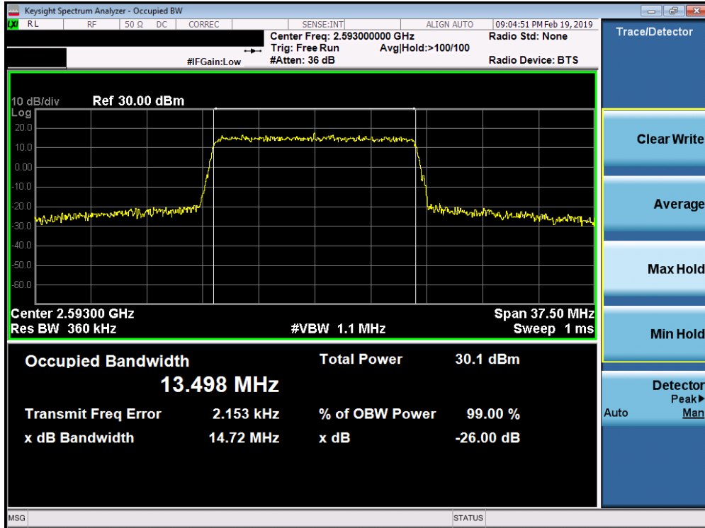
Plot 7-135. Occupied Bandwidth Plot (Band 41 PC3 / Band 38 - 15.0MHz 64-QAM - Full RB Configuration)
