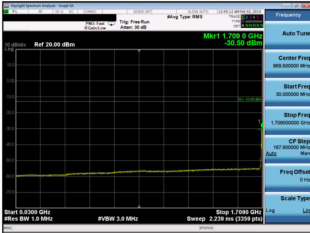
Plot 7-187. Conducted Spurious Plot (Band 66/4 - 20.0MHz QPSK - RB Size 1, RB Offset 0 - Low Channel)
