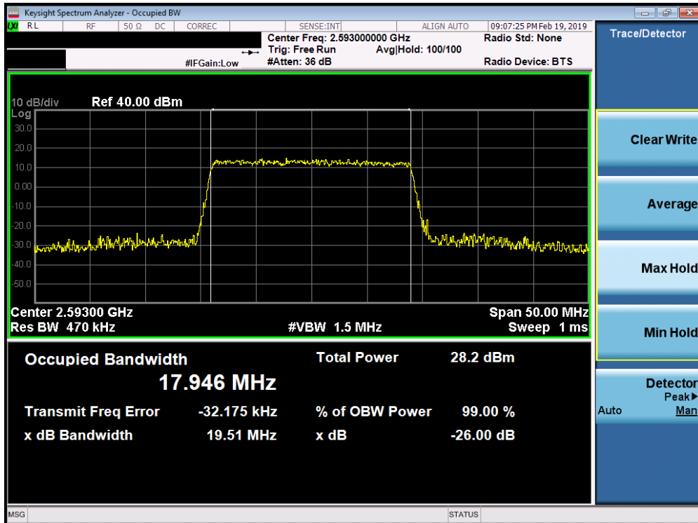
Plot 7-140. Occupied Bandwidth Plot (Band 41 PC3 / Band 38 - 20.0MHz 256-QAM - Full RB Configuration)
