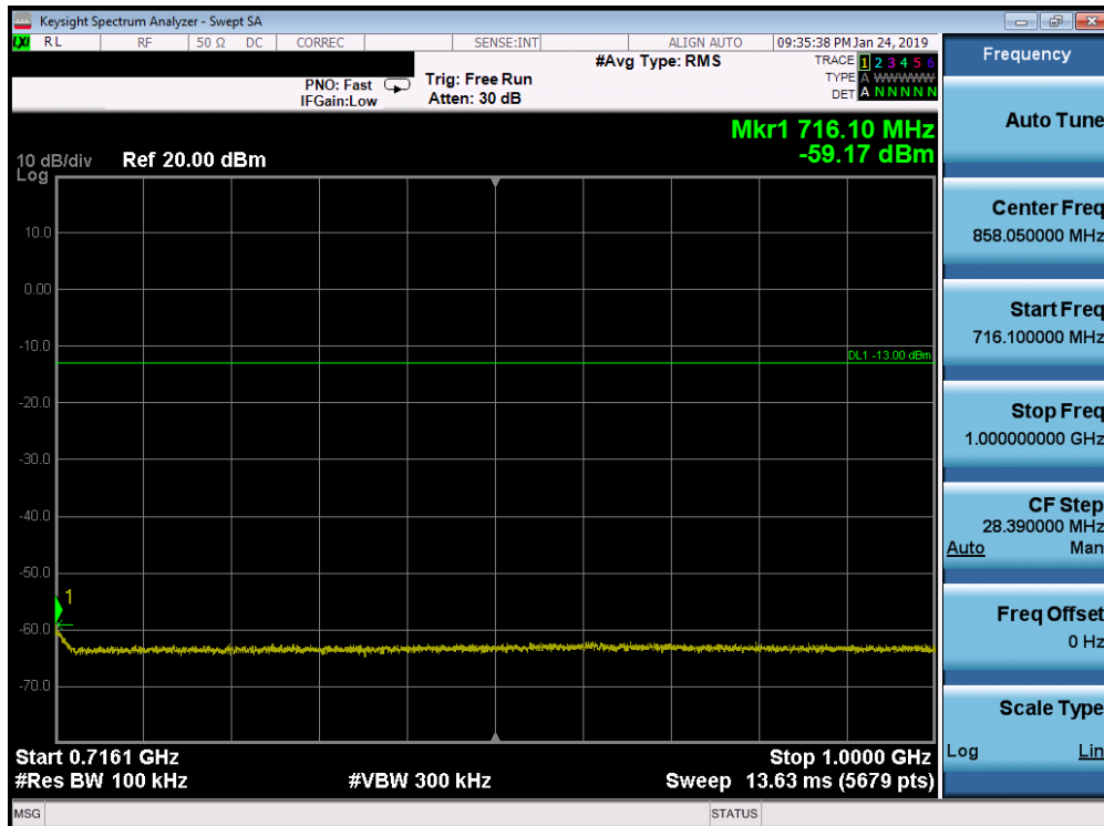
Plot 7-173. Conducted Spurious Plot (Band 12 - 10.0MHz QPSK - RB Size 1, RB Offset 0 - High Channel)
