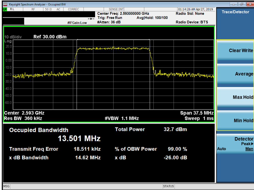
Plot 7-151. Occupied Bandwidth Plot (Band 41 PC2 - 15.0MHz 64-QAM - Full RB Configuration)
