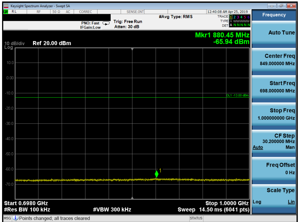
Plot 7-158. Conducted Spurious Plot (Band 71 - 20.0MHz QPSK - RB Size 1, RB Offset 0 - Low Channel)
