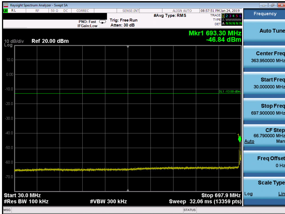
Plot 7-166. Conducted Spurious Plot (Band 12 - 10.0MHz QPSK - RB Size 1, RB Offset 0 - Low Channel)
