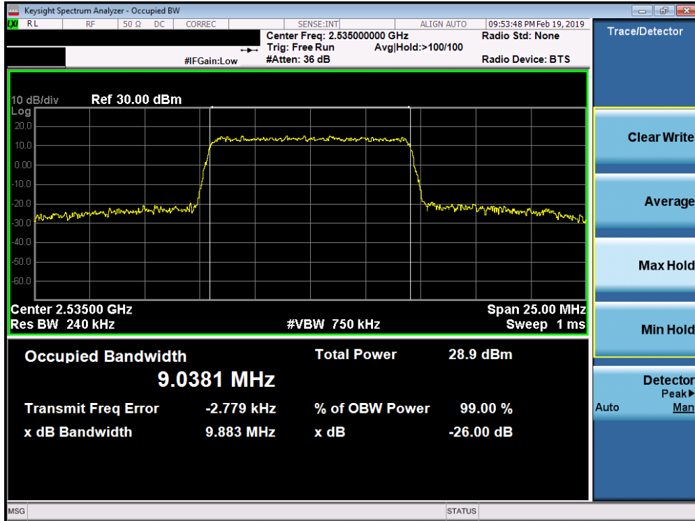
Plot 7-115. Occupied Bandwidth Plot (Band 7 - 10.0MHz 64-QAM - Full RB Configuration)
