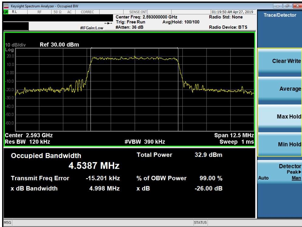
Plot 7-143. Occupied Bandwidth Plot (Band 41 PC2 – 5.0MHz 64-QAM - Full RB Configuration)
