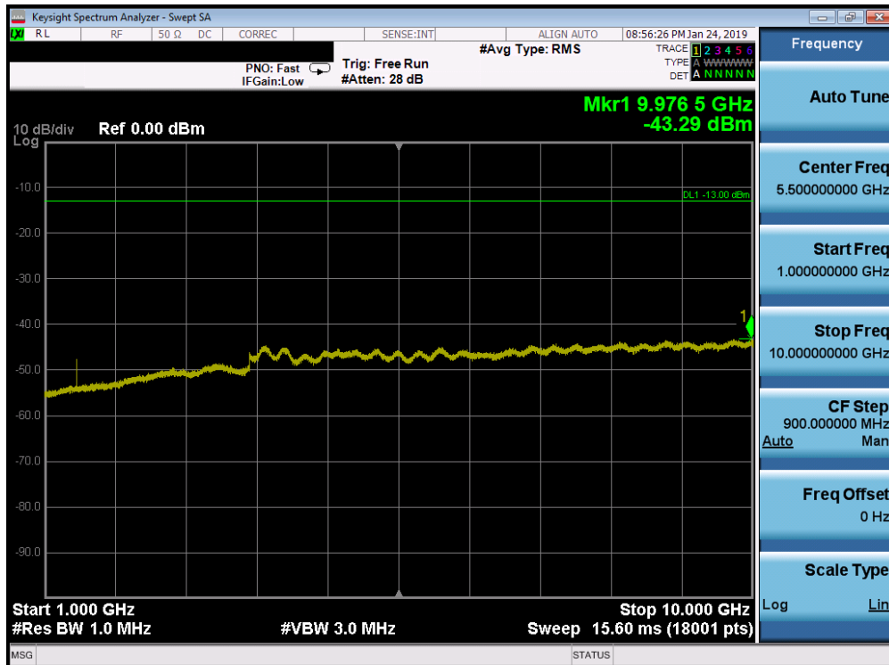
Plot 7-171. Conducted Spurious Plot (Band 12 - 10.0MHz QPSK - RB Size 1, RB Offset 0 - Mid Channel)
