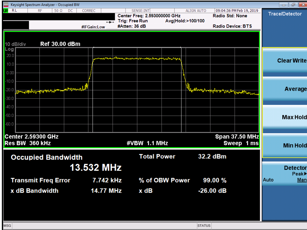
Plot 7-133. Occupied Bandwidth Plot (Band 41 PC3 / Band 38 - 15.0MHz QPSK - Full RB Configuration)
