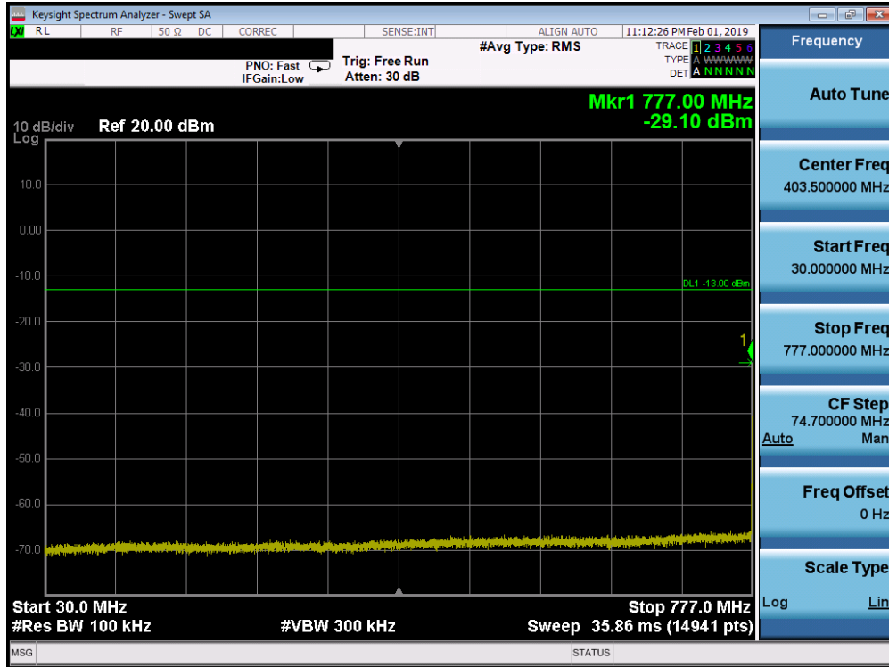
Plot 7-175. Conducted Spurious Plot (Band 13 - 10.0MHz QPSK - RB Size 1, RB Offset 0)
