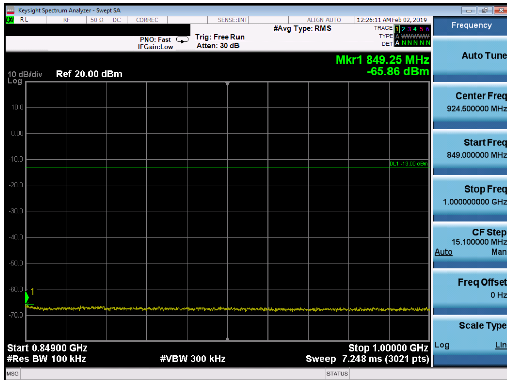
Plot 7-179. Conducted Spurious Plot (Band 26/5 - 10.0MHz QPSK - RB Size 1, RB Offset 0 - Low Channel)
