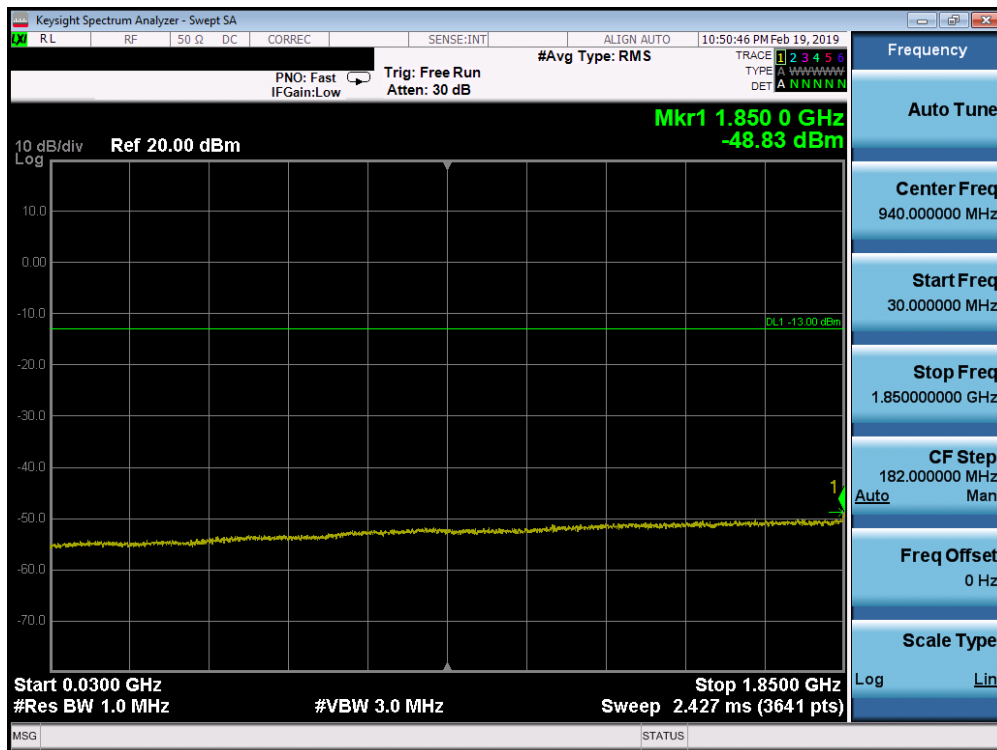
Plot 7-199. Conducted Spurious Plot (Band 25/2- 20.0MHz QPSK - RB Size 1, RB Offset 0 - Mid Channel)
