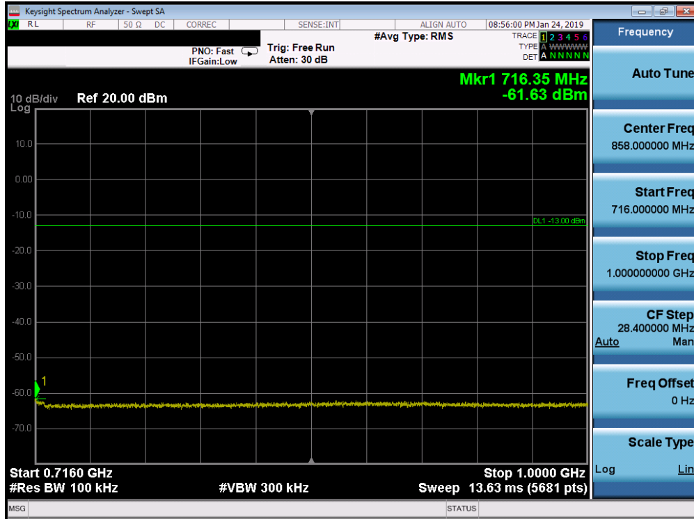
Plot 7-170. Conducted Spurious Plot (Band 12 - 10.0MHz QPSK - RB Size 1, RB Offset 0 - Mid Channel)
