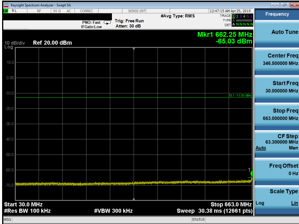
Plot 7-163. Conducted Spurious Plot (Band 71 - 20.0MHz QPSK - RB Size 1, RB Offset 0 - High Channel)
