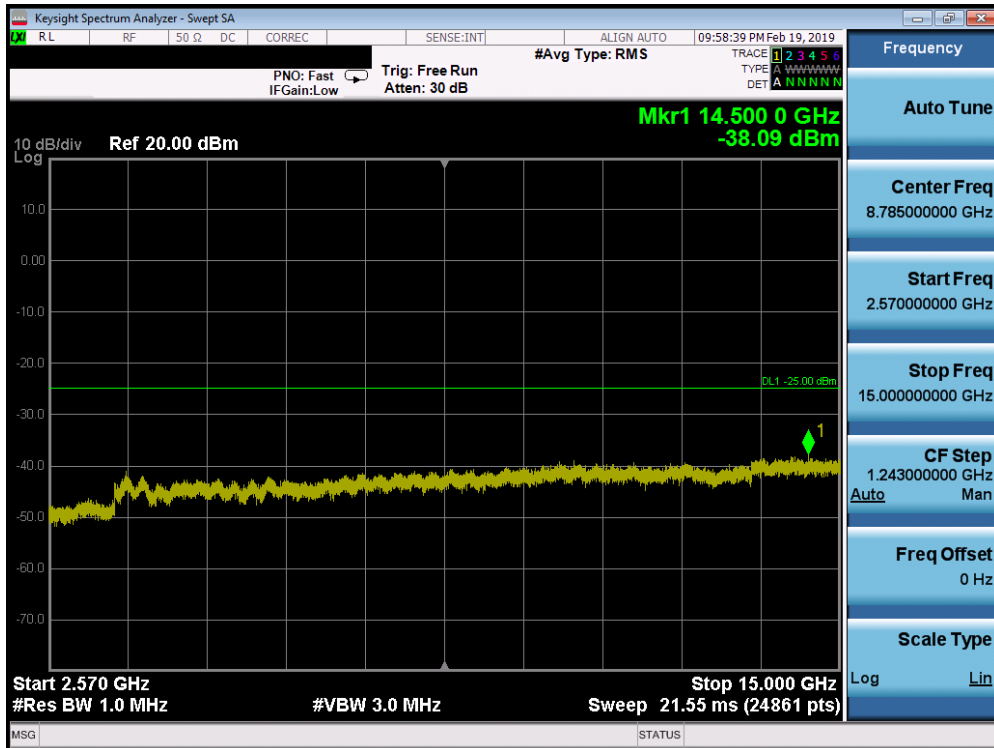
Plot 7-206. Conducted Spurious Plot (Band 7 - 20.0MHz QPSK - RB Size 1, RB Offset 0 - Low Channel)
