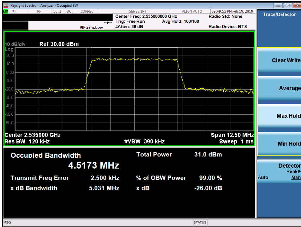
Plot 7-109. Occupied Bandwidth Plot (Band 7 – 5.0MHz QPSK - Full RB Configuration)
