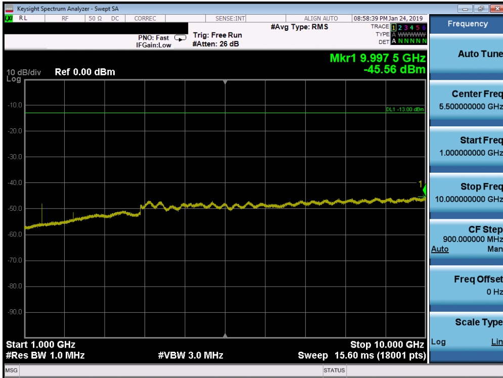
Plot 7-168. Conducted Spurious Plot (Band 12 - 10.0MHz QPSK - RB Size 1, RB Offset 0 - Low Channel)
