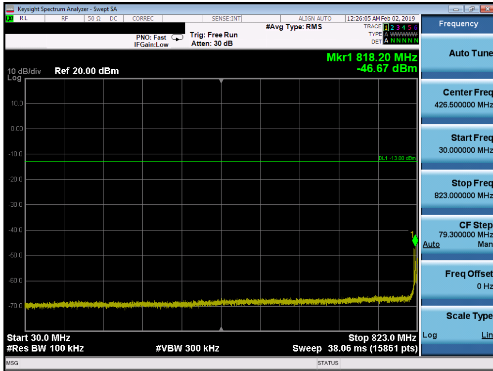
Plot 7-178. Conducted Spurious Plot (Band 26/5 - 10.0MHz QPSK - RB Size 1, RB Offset 0 - Low Channel)
