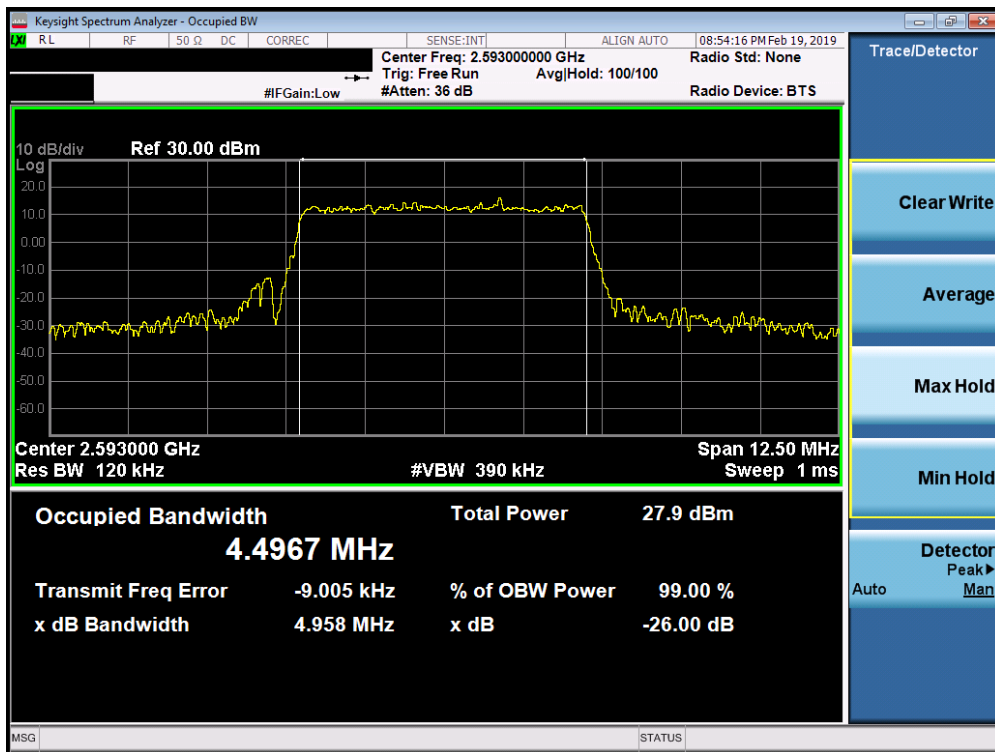
Plot 7-128. Occupied Bandwidth Plot (Band 41 PC3 / Band 38 – 5.0MHz 256-QAM - Full RB Configuration)
