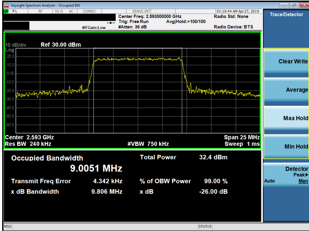
Plot 7-147. Occupied Bandwidth Plot (Band 41 PC2 - 10.0MHz 64-QAM - Full RB Configuration)
