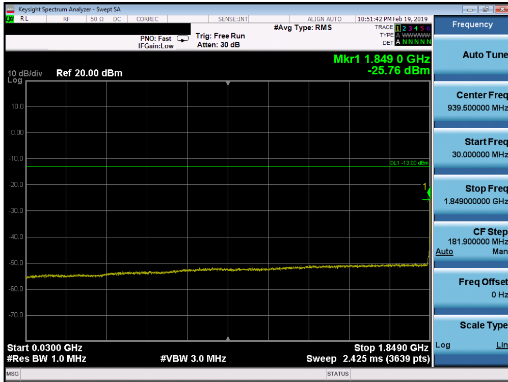
Plot 7-196. Conducted Spurious Plot (Band 25/2- 20.0MHz QPSK - RB Size 1, RB Offset 0 - Low Channel)
