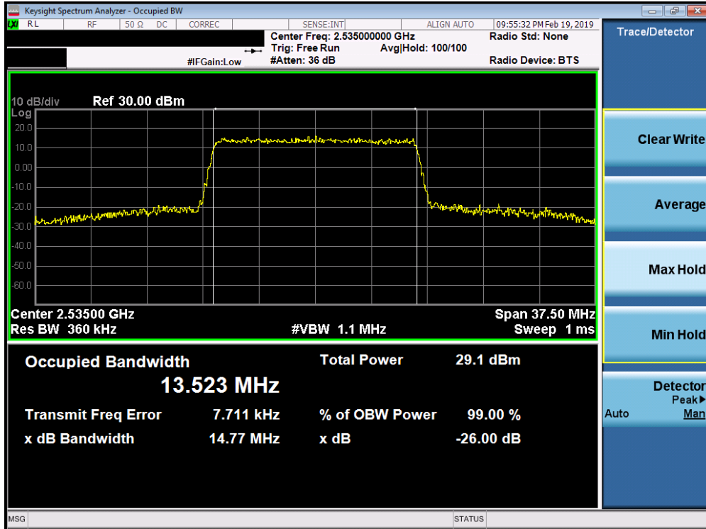
Plot 7-119. Occupied Bandwidth Plot (Band 7 - 15.0MHz 64-QAM - Full RB Configuration)
