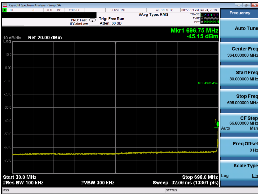
Plot 7-169. Conducted Spurious Plot (Band 12 - 10.0MHz QPSK - RB Size 1, RB Offset 0 - Mid Channel)
