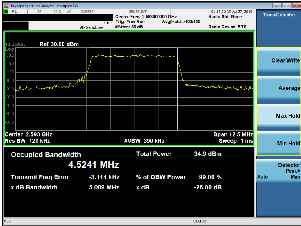
Plot 7-141. Occupied Bandwidth Plot (Band 41 PC2– 5.0MHz QPSK - Full RB Configuration)
