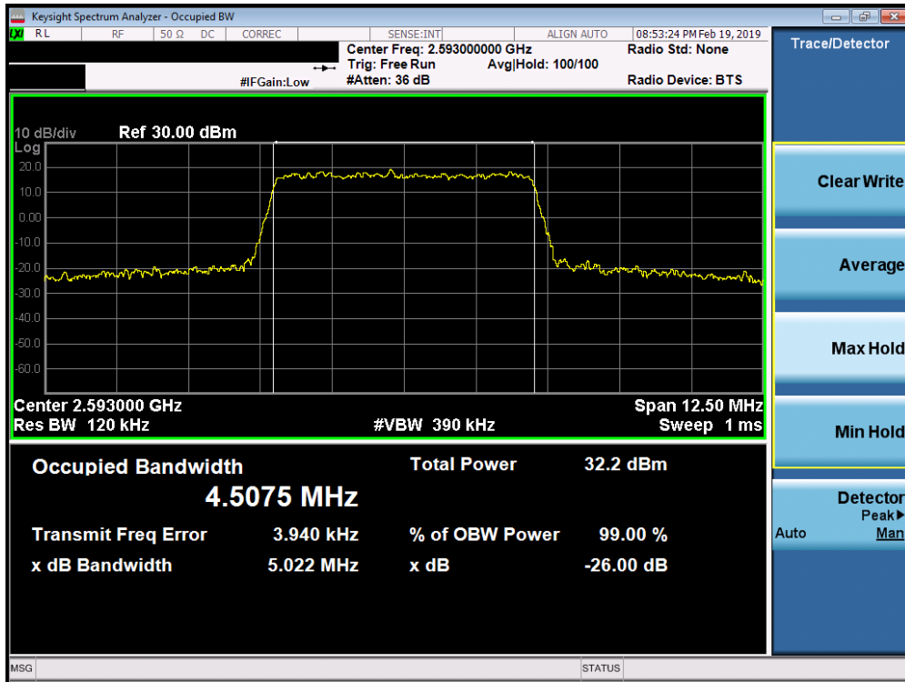
Plot 7-125. Occupied Bandwidth Plot (Band 41 PC3 / Band 38– 5.0MHz QPSK - Full RB Configuration)
