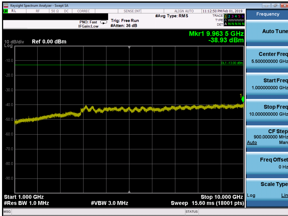
Plot 7-177. Conducted Spurious Plot (Band 13 - 10.0MHz QPSK - RB Size 1, RB Offset 0)
