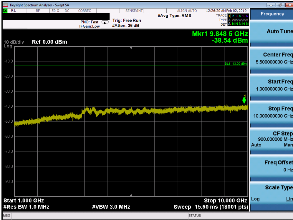
Plot 7-180. Conducted Spurious Plot (Band 26/5 - 10.0MHz QPSK - RB Size 1, RB Offset 0 - Low Channel)
