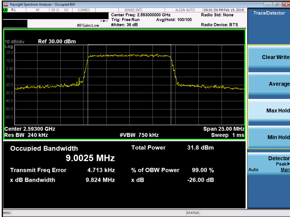
Plot 7-129. Occupied Bandwidth Plot (Band 41 PC3 / Band 38 - 10.0MHz QPSK - Full RB Configuration)
