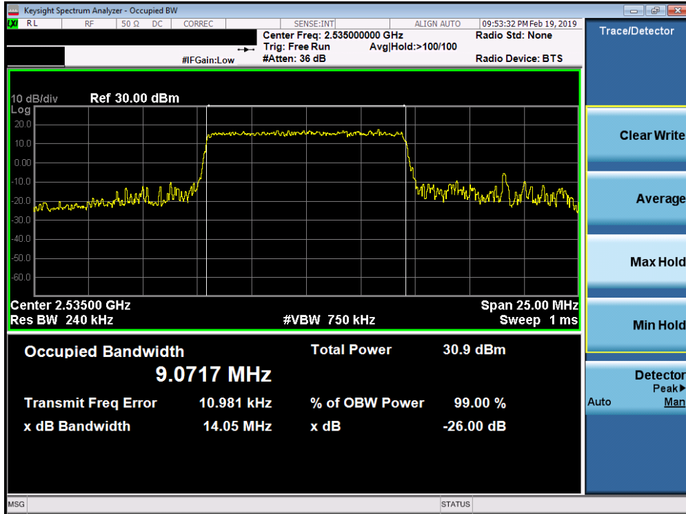
Plot 7-113. Occupied Bandwidth Plot (Band 7 - 10.0MHz QPSK - Full RB Configuration)
