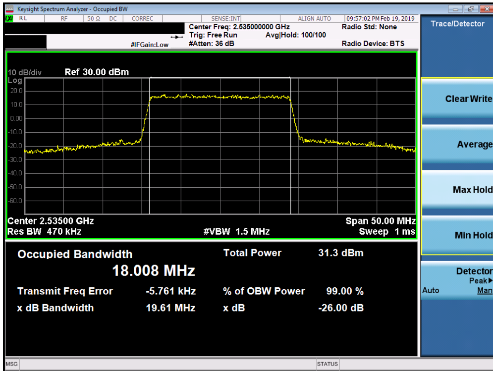
Plot 7-121. Occupied Bandwidth Plot (Band 7 - 20.0MHz QPSK - Full RB Configuration)
