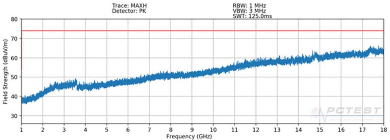
Plot 7-15. Radiated Spurious Plot above 1GHz (Configuration 4 - H)
