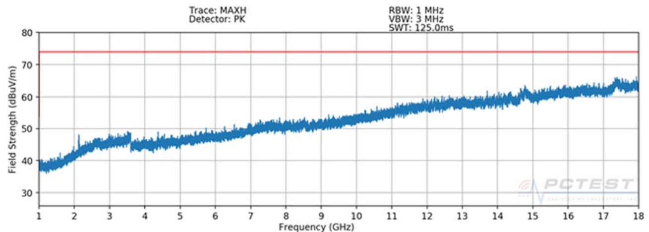
Plot 7-19. Radiated Spurious Plot above 1GHz (Configuration 5 - H)
