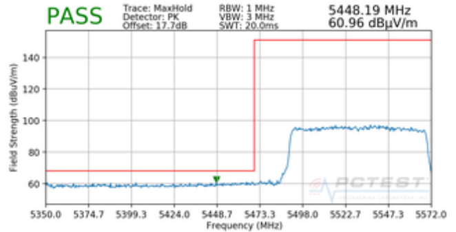
Plot 7-381. Radiated Band Edge Plot ANT (Peak – WCP)
