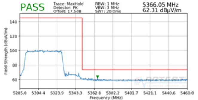
Plot 7-331. Radiated Upper Band Edge Plot SISO ANT2 (Peak – UNII Band 2A)
