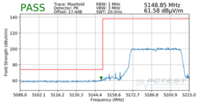
Plot 7-329. Radiated Lower Band Edge Plot SISO ANT2 (Peak – UNII Band 1)
