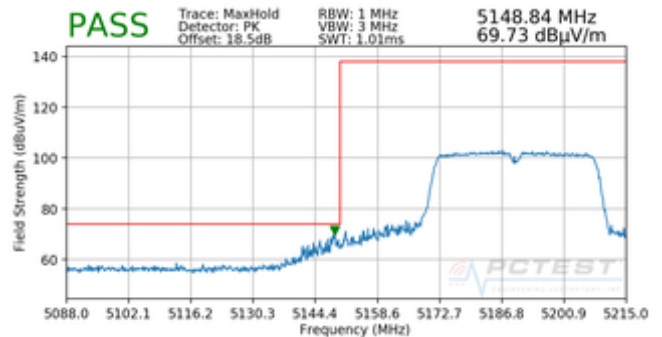
Plot 7-302. Radiated Lower Band Edge Plot SISO ANT1 (Peak – UNII Band 1)
