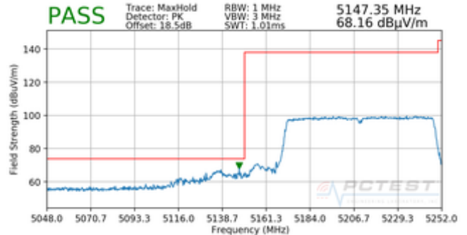
Plot 7-311. Radiated Lower Band Edge Plot SISO ANT1 (Peak – UNII Band 1)
