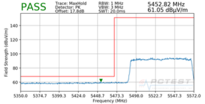
Plot 7-315. Radiated Lower Band Edge Plot SISO ANT1 (Peak – UNII Band 2C)
