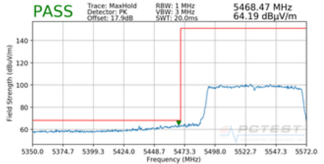
Plot 7-378. Radiated Lower Band Edge Plot MIMO (Peak – UNII Band 2C)
