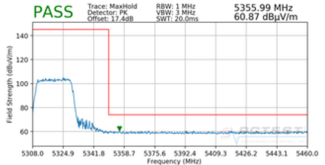
Plot 7-295. Radiated Upper Band Edge Plot SISO ANT1 (Peak – UNII Band 2A)
