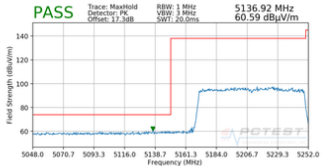
Plot 7-338. Radiated Lower Band Edge Plot SISO ANT2 (Peak – UNII Band 1)
