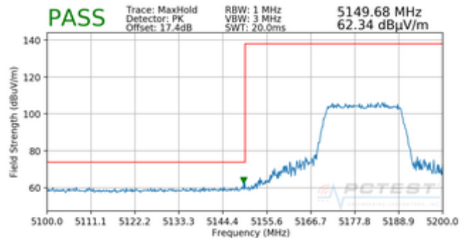
Plot 7-293. Radiated Lower Band Edge Plot SISO ANT1 (Peak – UNII Band 1)
