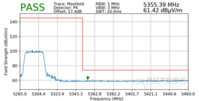
Plot 7-304. Radiated Upper Band Edge Plot SISO ANT1 (Peak – UNII Band 2A)
