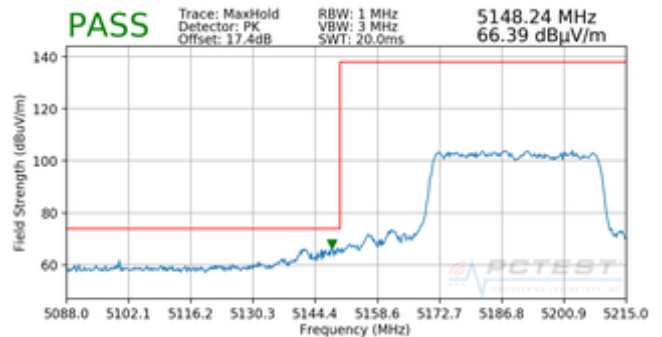
Plot 7-365. Radiated Lower Band Edge Plot MIMO (Peak – UNII Band 1)
