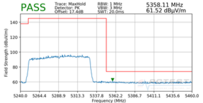
Plot 7-313. Radiated Upper Band Edge Plot SISO ANT1 (Peak – UNII Band 2A)
