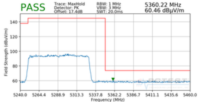
Plot 7-340. Radiated Upper Band Edge Plot SISO ANT2 (Peak – UNII Band 2A)
