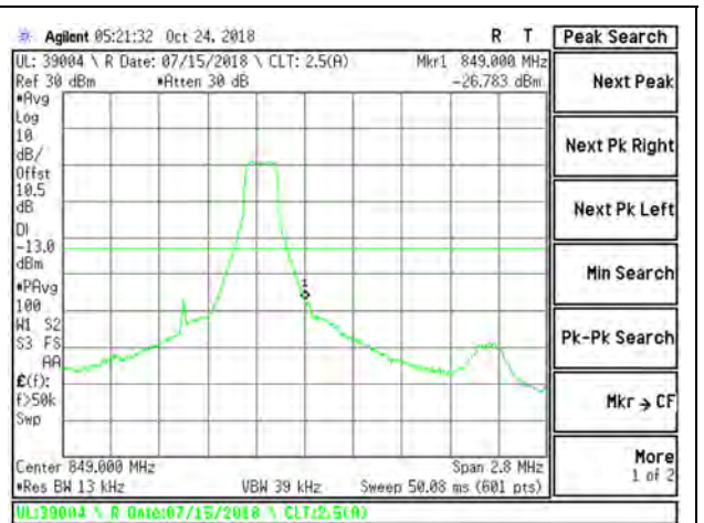
LTE B5 1.4MHz 16QAM High Channel RB1-
