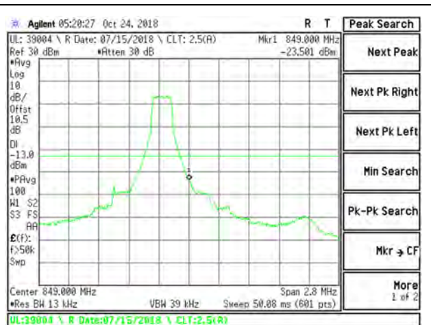
LTE B5 1.4MHz QPSK High Channel RB1-
