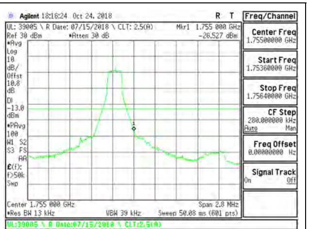
LTE B4 1.4MHz 16QAM High Channel RB1-50
