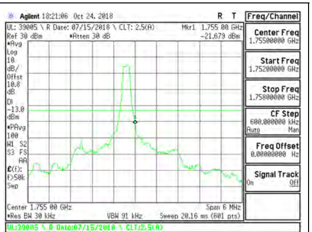
LTE B4 3MHz 16QAM High Channel RB1-140
