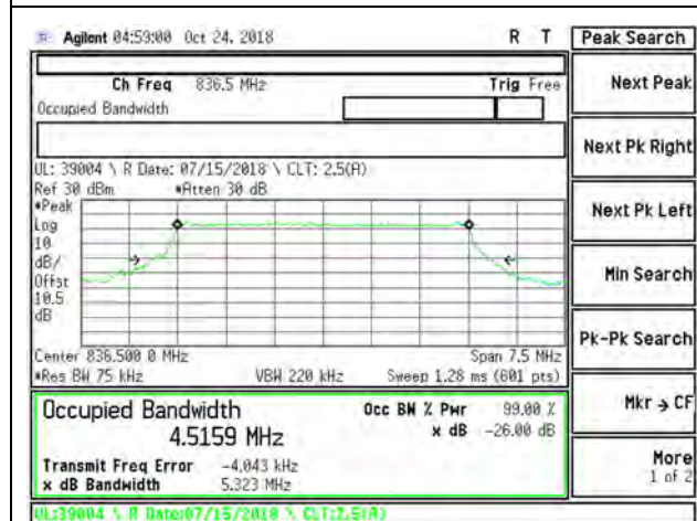
LTE B5 5MHz QPSK Mid Channel RB25-0
