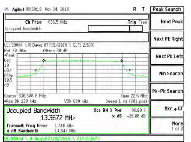
LTE B26 15MHz 16QAM Mid Channel RB75-0
