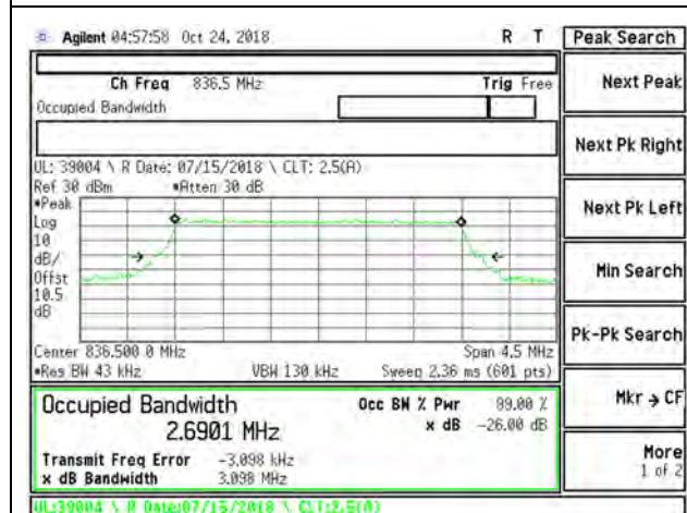
LTE B5 3MHz QPSK Mid Channel RB15-0
