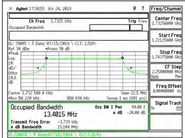
LTE B4 15MHz QPSK Mid Channel RB75-0
