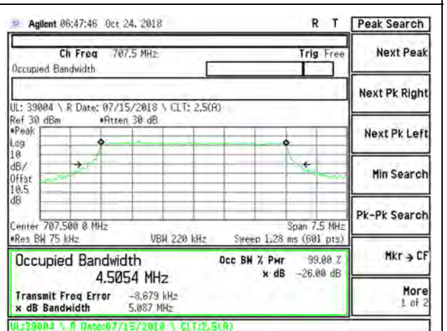
LTE B12 5MHz 16QAM Mid Channel RB25-0
