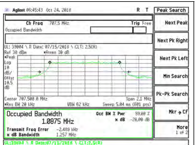
LTE B12 1.4MHz 16QAM Mid Channel RB6-0
