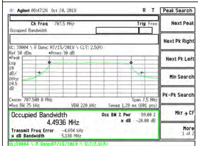
LTE B12 5MHz QPSK Mid Channel RB25-0
