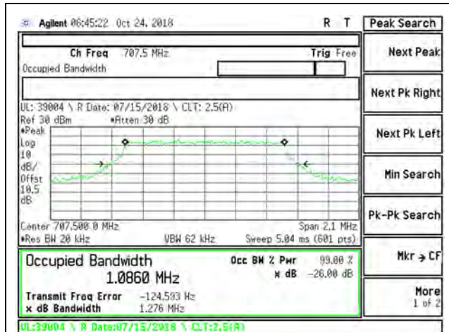
LTE B12 1.4MHz QPSK Mid Channel RB6-0
